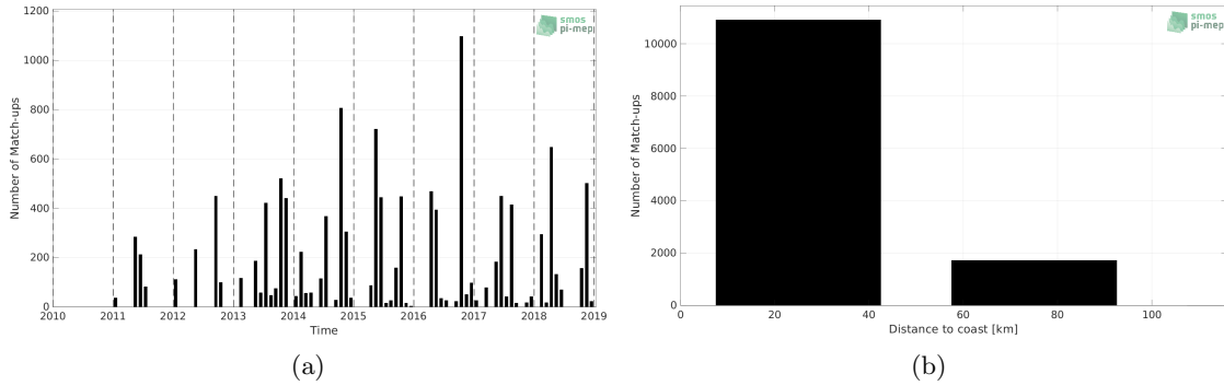
Figure 1: Number of match-ups between TSG (LEGOS-DM) and SMOS and SMAP SSS L4 OI v1 - 7 Days (LOPS) SSS as a function of time (a) and as function of the distance to coast (b) over the Baltic Sea Pi-MEP region and for the full satellite product period.
