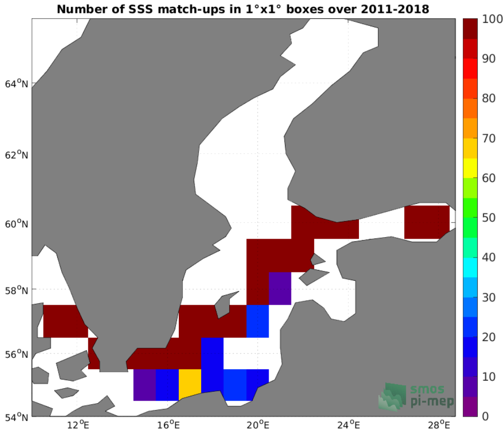
Figure 4: Number of SSS match-ups between TSG (LEGOS-DM) SSS and the SMOS and SMAP SSS L4 OI v1 - 7 Days (LOPS) SSS product for the Baltic Sea Pi-MEP region over 1^\circ \times 1^\circ boxes and for the full satellite product period.
