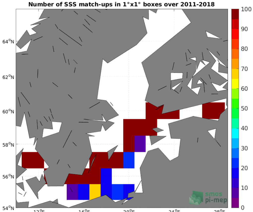
Figure 4: Number of SSS match-ups between TSG (LEGOS-DM) SSS and the SMOS and SMAP SSS L4 OI v1 - 7 Days (LOPS) SSS product for the Baltic Sea Pi-MEP region over 1°x1° boxes and for the full satellite product period.
