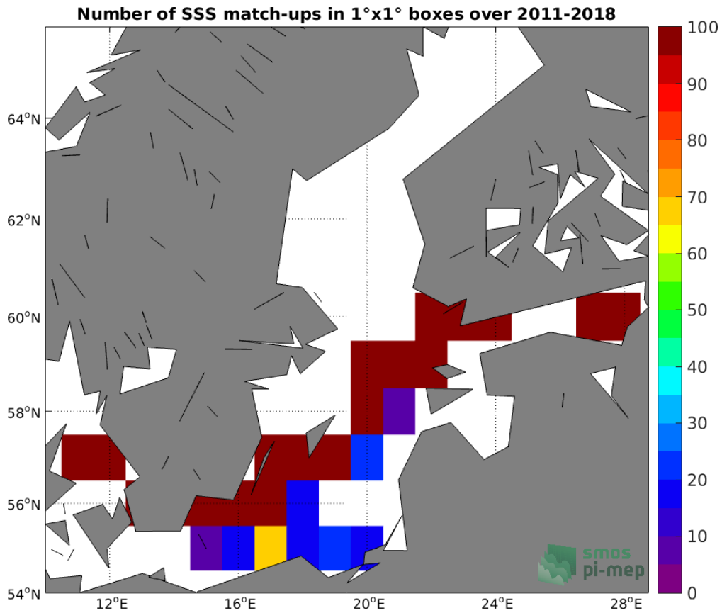
Figure 4: Number of SSS match-ups between TSG (LEGOS-DM) SSS and the SMOS and SMAP SSS L4 OI v1 - 7 Days (LOPS) SSS product for the Baltic Sea Pi-MEP region over 1°×1° boxes and for the full satellite product period.
