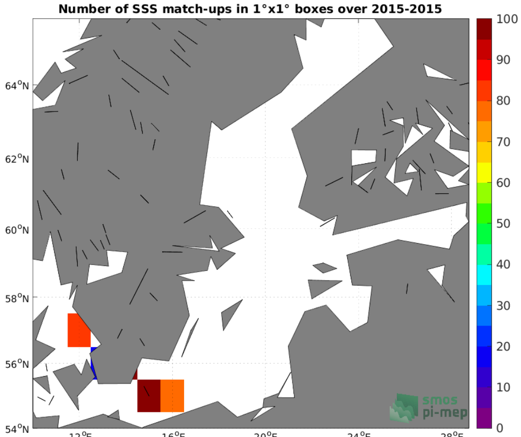
Figure 4: Number of SSS match-ups between TSG (GOSUD-Research-vessel) SSS and the SMOS and SMAP SSS L4 OI v1 - 7 Days (LOPS) SSS product for the Baltic Sea Pi-MEP region over 1°x1° boxes and for the full satellite product period.
