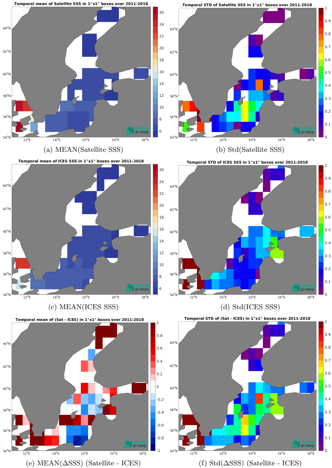
Figure 6: Temporal mean (left) and Std (right) of SSS from SMOS and SMAP SSS L4 OI v1 - 7 Days (LOPS) (top), ICES (middle), and of \Delta SSS (Satellite - ICES). Only match-up pairs are used to generate these maps.
