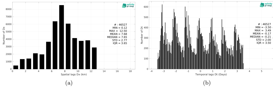
Figure 5: Histograms of the spatial (a) and temporal (b) lags between the location/time of the ICES measurement and the date of the corresponding SMOS and SMAP SSS L4 OI v1 - 7 Days (LOPS) SSS pixel.
