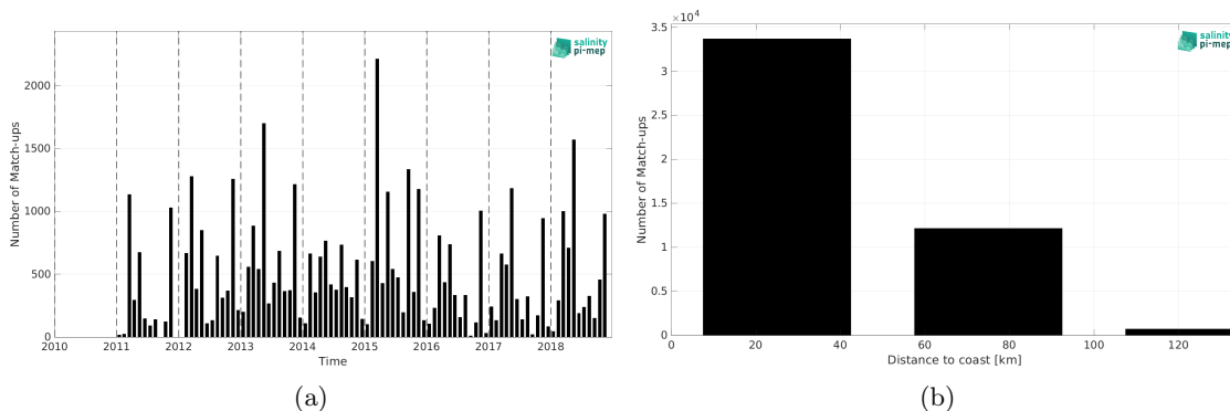
Figure 1: Number of match-ups between ICES and SMOS and SMAP SSS L4 OI v1 - 7 Days (LOPS) SSS as a function of time (a) and as function of the distance to coast (b) over the Baltic Sea Pi-MEP region and for the full satellite product period.
