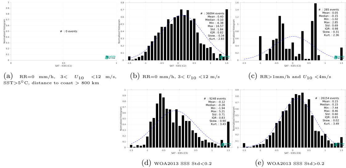
Figure 13: Normalized histogram of \Delta SSS (SMOS and SMAP SSS L4 OI v1 - 7 Days (LOPS) - ICES) for 5 different subdatasets corresponding to: RR=0 mm/h, 3 < U_{10} < 12 m/s, SST > 5°C, distance to coast > 800 km (a), RR=0 mm/h, 3 < U_{10} < 12 m/s (b), RR > 1mm/h and U_{10} < 4 m/s (c), WOA2013 SSS Std < 0.2 (d), WOA2013 SSS Std > 0.2 (e).
