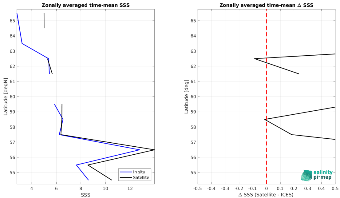
Figure 8: Left panel: Zonal mean SSS from SMOS and SMAP SSS L4 OI v1 - 7 Days (LOPS) satellite product (black) and from ICES (blue). Right panel: Zonal mean of \Delta SSS (Satellite - ICES) for all the collected Pi-MEP match-up pairs estimated over the full satellite product period.
