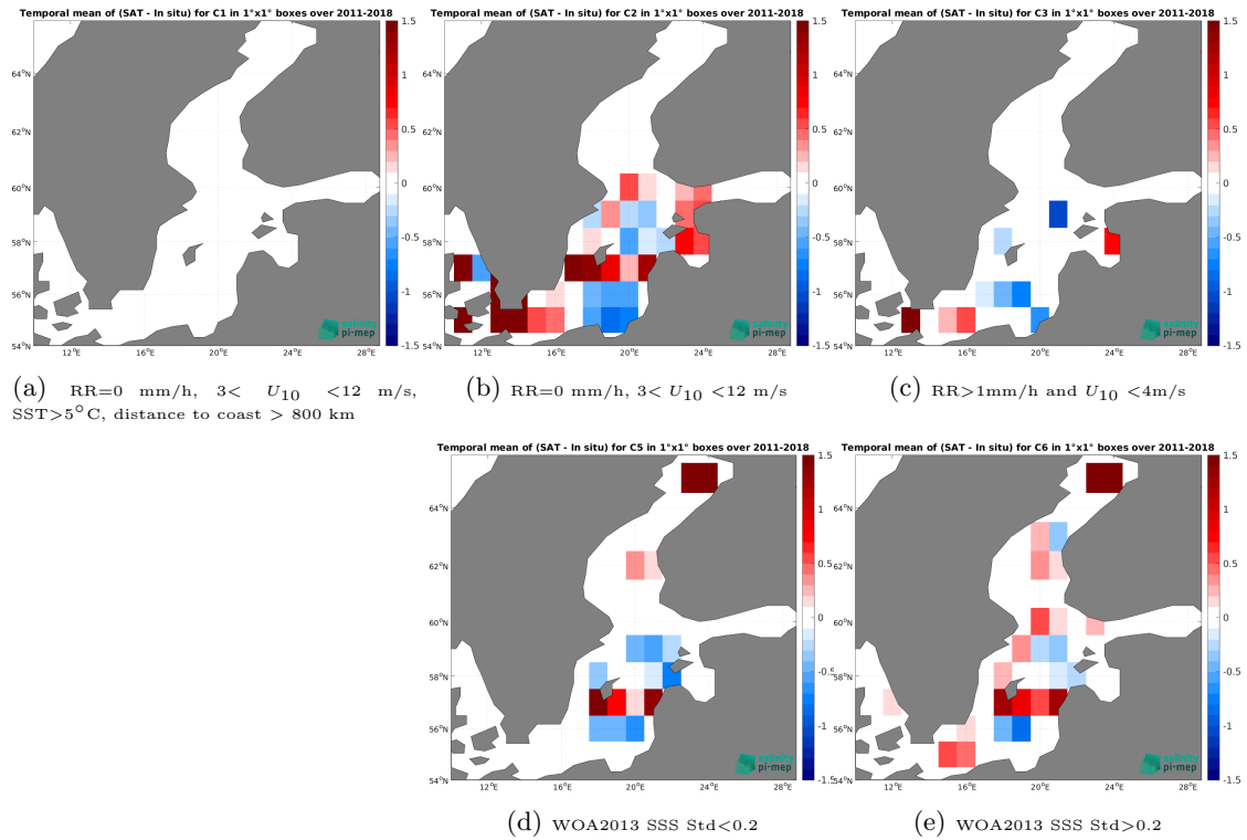
Figure 12: Temporal mean gridded over spatial boxes of size 1^{\circ}\times 1^{\circ} of \Delta\text{SSS} (SMOS and SMAP SSS L4 OI v1 - 7 Days (LOPS) - ICES) for 5 different subdatasets corresponding to:RR=0 mm/h, 3 < U_{10} < 12 m/s, SST > 5^{\circ}\text{C} , distance to coast > 800 km (a), RR=0 mm/h, 3 < U_{10} < 12 m/s (b), RR > 1 mm/h and U_{10} < 4 m/s (c), WOA2013 SSS Std < 0.2 (d), WOA2013 SSS Std > 0.2 (e).
