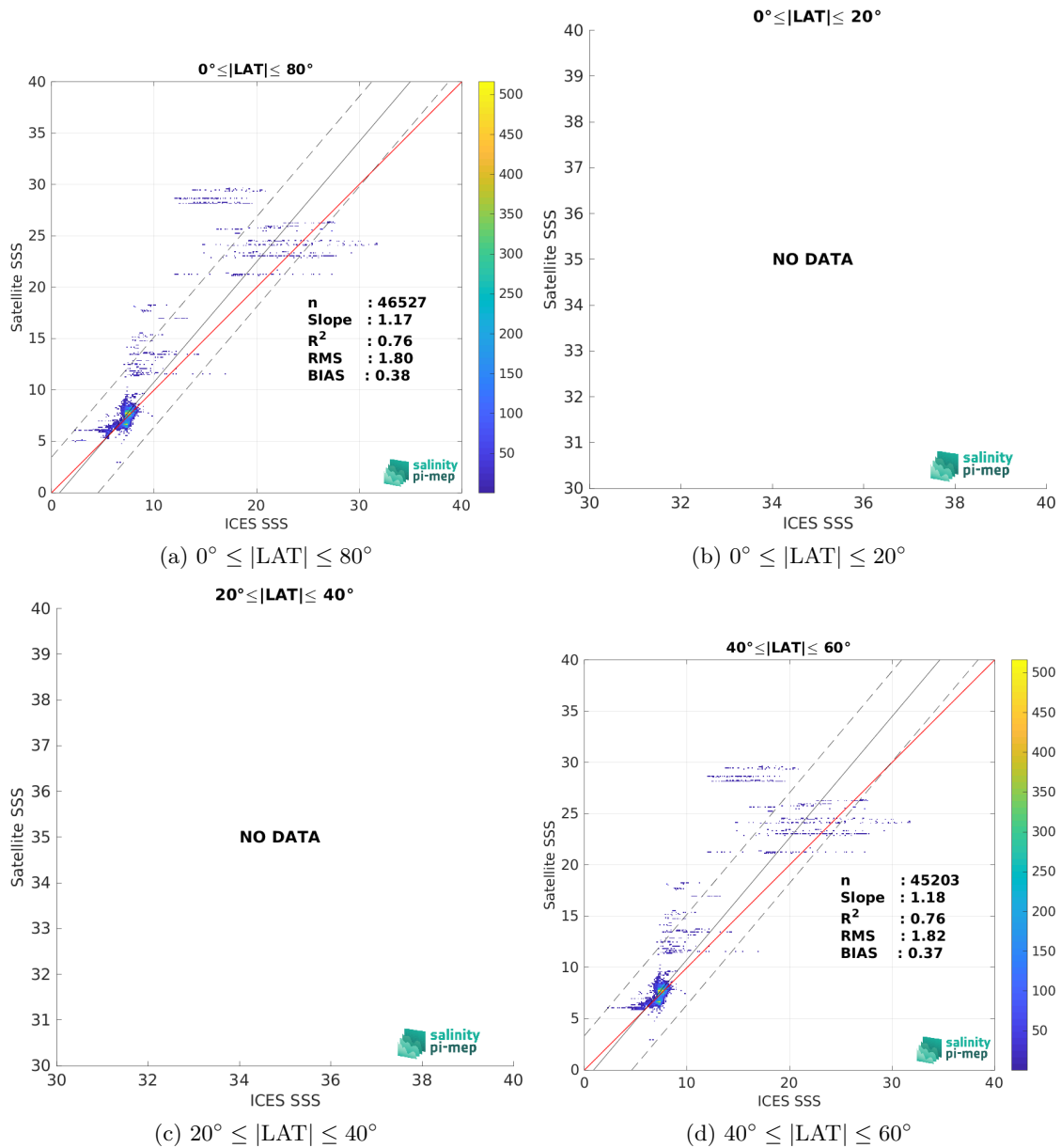
Figure 9: Contour maps of the concentration of SMOS and SMAP SSS L4 OI v1 - 7 Days (LOPS) SSS (y-axis) versus ICES SSS (x-axis) at match-up pairs for different latitude bands. For each plot, the red line shows x=y . The black thin and dashed lines indicate a linear fit through the data cloud and the \pm 95\% confidence levels, respectively. The number match-up pairs n , the slope and R^2 coefficient of the linear fit, the root mean square (RMS) and the mean bias between satellite and in situ data are indicated for each latitude band in each plots.
