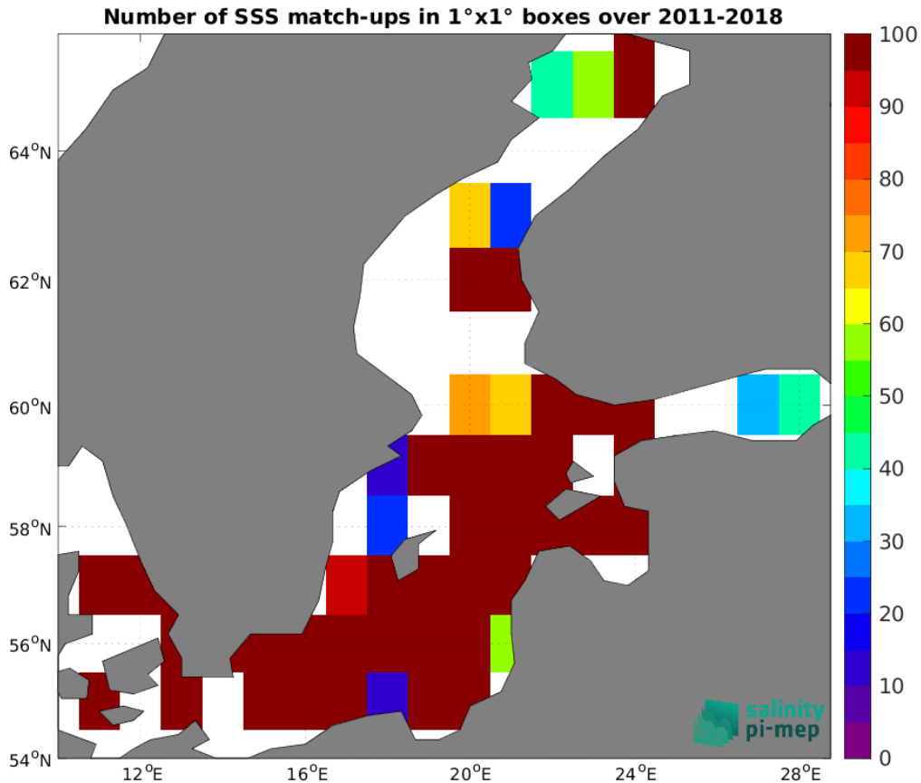
Figure 4: Number of SSS match-ups between ICES SSS and the SMOS and SMAP SSS L4 OI v1 - 7 Days (LOPS) SSS product for the Baltic Sea Pi-MEP region over 1^\circ \times 1^\circ boxes and for the full satellite product period.
