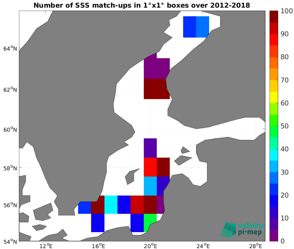
Figure 4: Number of SSS match-ups between Argo SSS and the SMOS and SMAP SSS L4 OI v1 - 7 Days (LOPS) SSS product for the Baltic Sea Pi-MEP region over 1^\circ \times 1^\circ boxes and for the full satellite product period.
