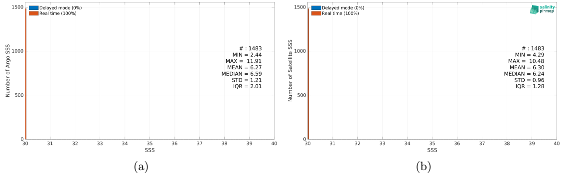
Figure 2: Histograms of SSS from Argo (a) and SMOS and SMAP SSS L4 OI v1 - 7 Days (LOPS) (b) considering all match-up pairs per bins of 0.1 over the Baltic Sea Pi-MEP region and for the full satellite product period.
