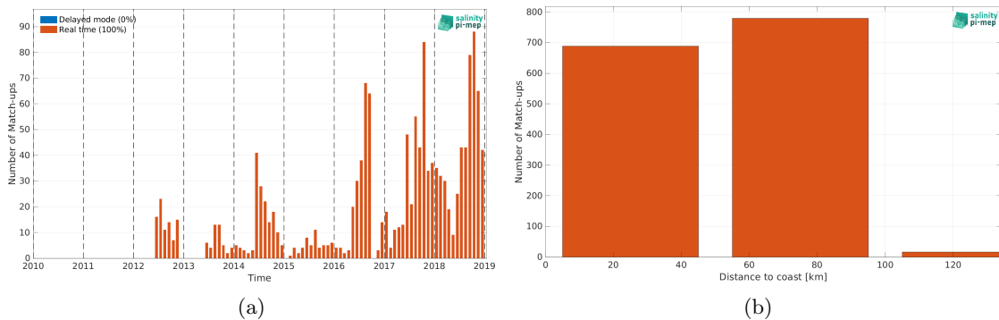
Figure 1: Number of match-ups between Argo and SMOS and SMAP SSS L4 OI v1 - 7 Days (LOPS) SSS as a function of time (a) and as function of the distance to coast (b) over the Baltic Sea Pi-MEP region and for the full satellite product period.
