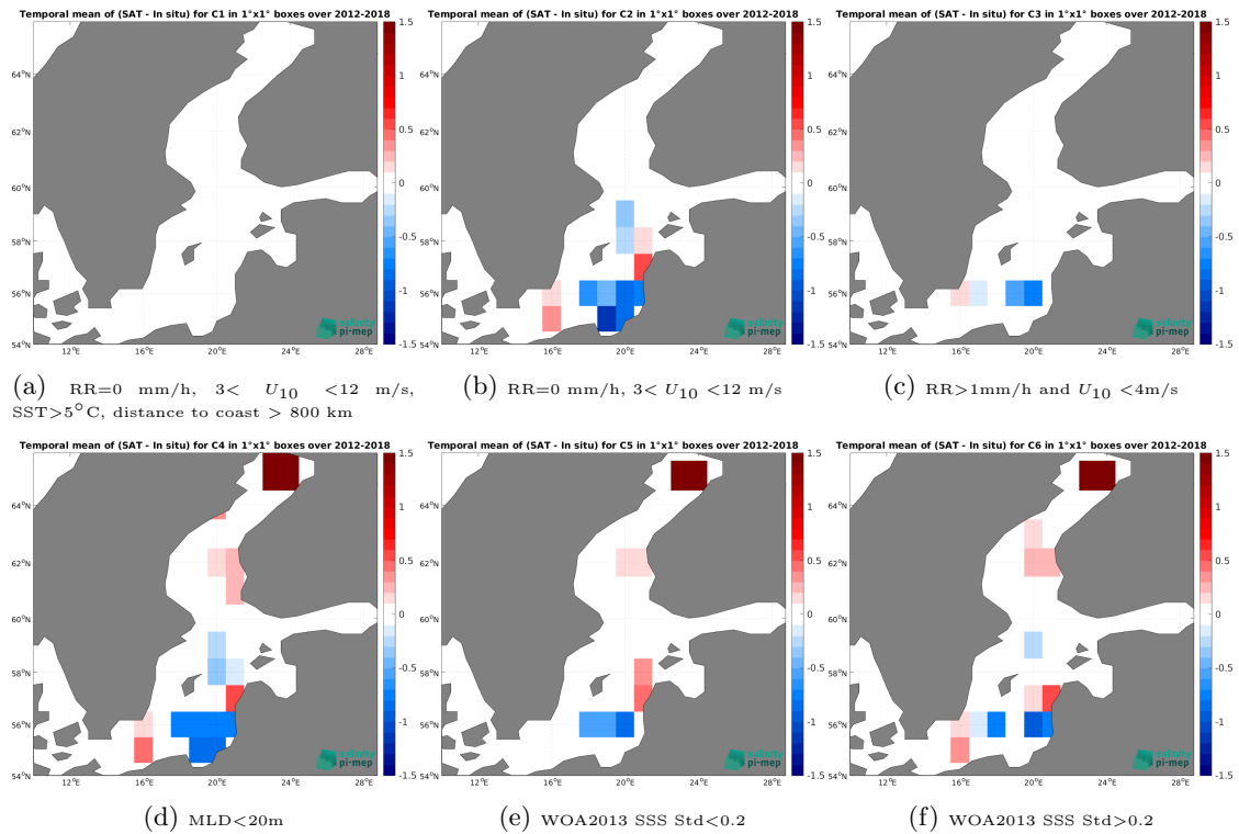
Figure 12: Temporal mean gridded over spatial boxes of size 1^{\circ}\times 1^{\circ} of \Delta\text{SSS} (SMOS and SMAP SSS L4 OI v1 - 7 Days (LOPS) - Argo) for 6 different subdatasets corresponding to:RR=0 mm/h, 3 < U_{10} < 12 m/s, SST >5^{\circ}\text{C} , distance to coast > 800 km (a), RR=0 mm/h, 3 < U_{10} < 12 m/s (b), RR >1\text{mm/h} and U_{10} < 4\text{m/s} (c),MLD <20\text{m} (d),WOA2013 SSS Std <0.2 (e),WOA2013 SSS Std >0.2 (f).
