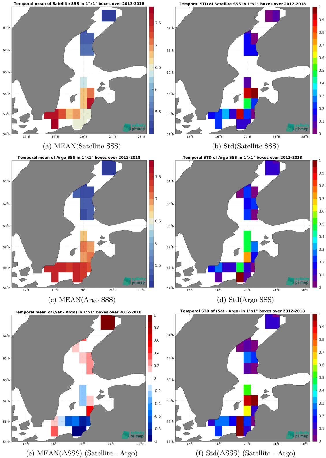
Figure 6: Temporal mean (left) and Std (right) of SSS from SMOS and SMAP SSS L4 OI v1 - 7 Days (LOPS) (top), Argo (middle), and of \Delta SSS (Satellite - Argo). Only match-up pairs are used to generate these maps.
