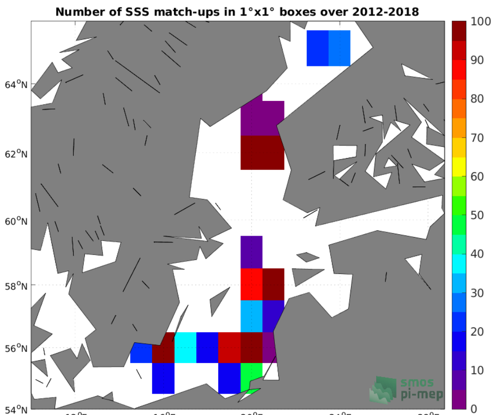
Figure 4: Number of SSS match-ups between Argo SSS and the SMOS and SMAP SSS L4 OI v1 - 7 Days (LOPS) SSS product for the Baltic Sea Pi-MEP region over 1°x1° boxes and for the full satellite product period.
