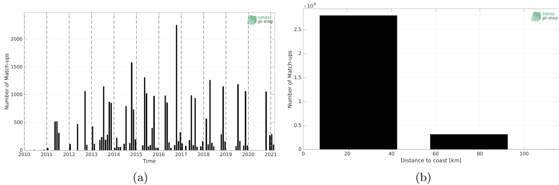
Figure 1: Number of match-ups between TSG (LEGOS-DM) and SMOS SSS L4 v1 - Weekly (CMEMS-CNR) SSS as a function of time (a) and as function of the distance to coast (b) over the Baltic Sea Pi-MEP region and for the full satellite product period.
