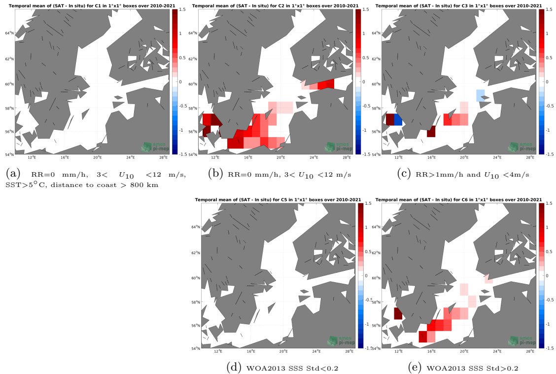
Figure 12: Temporal mean gridded over spatial boxes of size 1^{\circ}\times 1^{\circ} of \Delta\text{SSS} (SMOS SSS L4 v1 - Weekly (CMEMS-CNR) - TSG (LEGOS-DM)) for 5 different subdatasets corresponding to: \text{RR}=0 mm/h, 3 < U_{10} < 12 m/s, \text{SST} > 5^{\circ}\text{C} , distance to coast > 800 km (a), \text{RR}=0 mm/h, 3 < U_{10} < 12 m/s (b), \text{RR} > 1 mm/h and U_{10} < 4 m/s (c), WOA2013 SSS Std < 0.2 (d), WOA2013 SSS Std > 0.2 (e).
