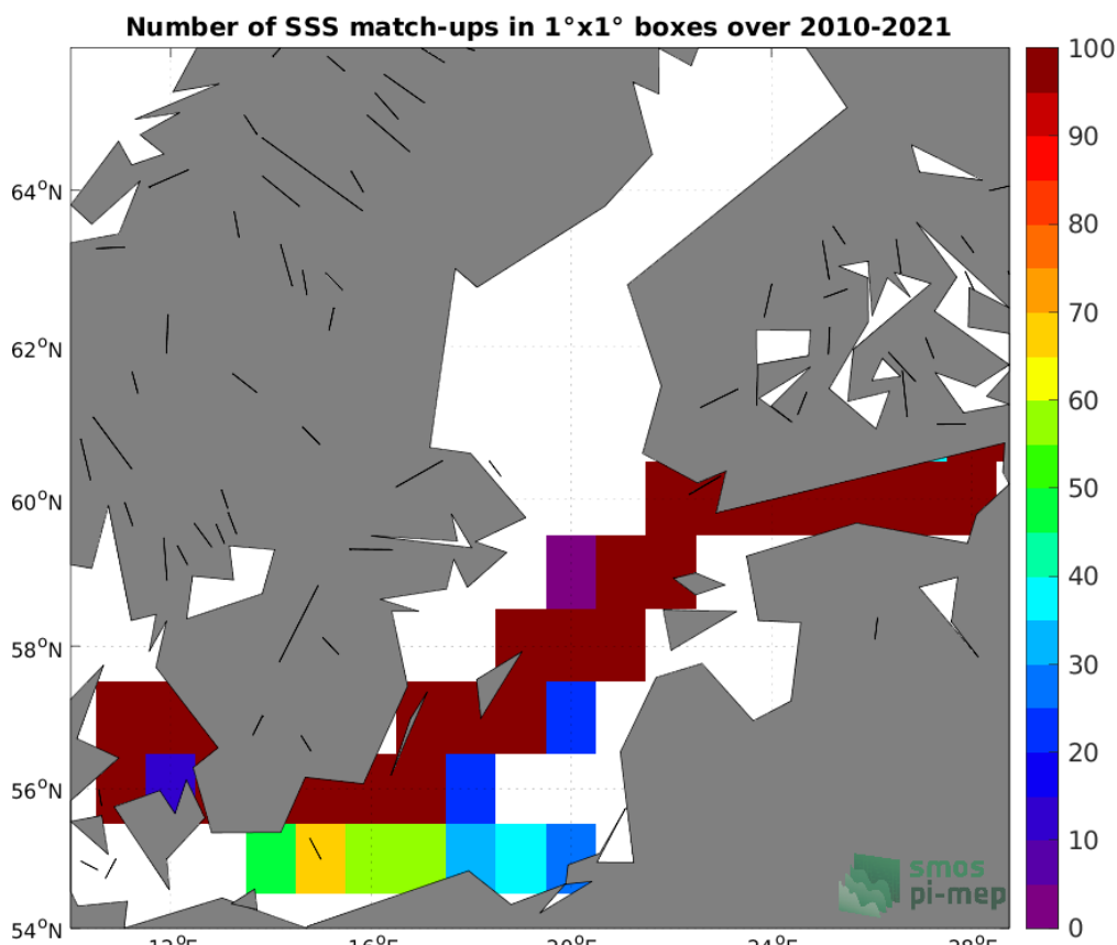
Figure 4: Number of SSS match-ups between TSG (LEGOS-DM) SSS and the SMOS SSS L4 v1 - Weekly (CMEMS-CNR) SSS product for the Baltic Sea Pi-MEP region over 1°x1° boxes and for the full satellite product period.
