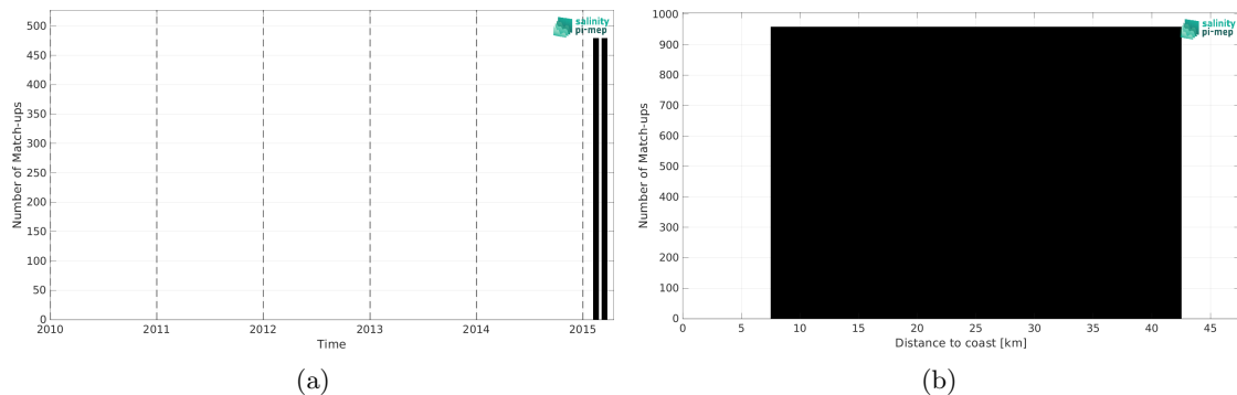
Figure 1: Number of match-ups between TSG (GOSUD-Research-vessel) and SMOS SSS L4 v1 - Weekly (CMEMS-CNR) SSS as a function of time (a) and as function of the distance to coast (b) over the Baltic Sea Pi-MEP region and for the full satellite product period.
