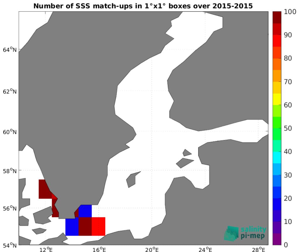
Figure 4: Number of SSS match-ups between TSG (GOSUD-Research-vessel) SSS and the SMOS SSS L4 v1 - Weekly (CMEMS-CNR) SSS product for the Baltic Sea Pi-MEP region over 1°x1° boxes and for the full satellite product period.
