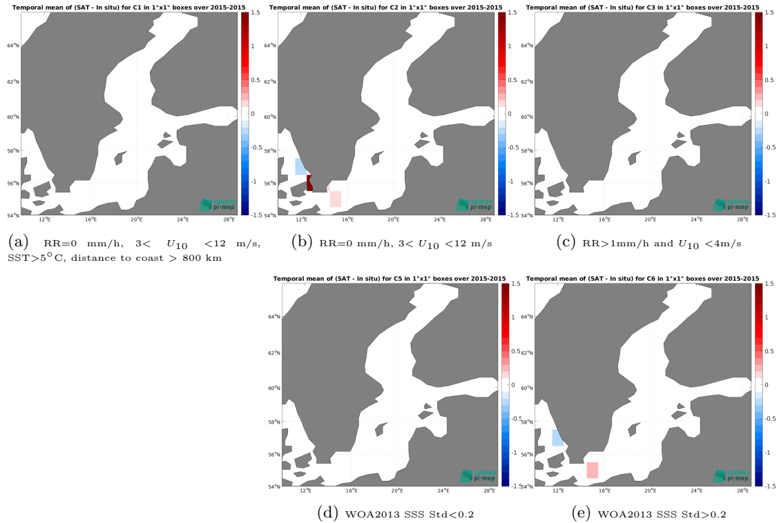
Figure 12: Temporal mean gridded over spatial boxes of size 1^{\circ}\times 1^{\circ} of \Delta SSS (SMOS SSS L4 v1 - Weekly (CMEMS-CNR) - TSG (GOSUD-Research-vessel)) for 5 different subdatasets corresponding to:RR=0 mm/h, 3 < U_{10} < 12 m/s, SST >5^{\circ}\text{C} , distance to coast > 800 km (a), RR=0 mm/h, 3 < U_{10} < 12 m/s (b), RR >1 mm/h and U_{10} < 4 m/s (c), WOA2013 SSS Std <0.2 (d), WOA2013 SSS Std >0.2 (e).
