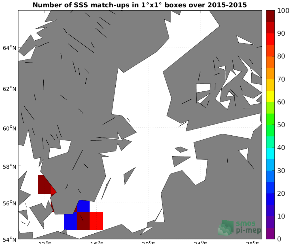
Figure 4: Number of SSS match-ups between TSG (GOSUD-Research-vessel) SSS and the SMOS SSS L4 v1 - Weekly (CMEMS-CNR) SSS product for the Baltic Sea Pi-MEP region over 1^\circ \times 1^\circ boxes and for the full satellite product period.
