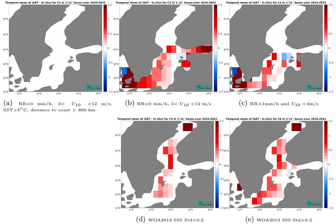
Figure 12: Temporal mean gridded over spatial boxes of size 1^{\circ}\times 1^{\circ} of \Delta\text{SSS} (SMOS SSS L4 v1 - Weekly (CMEMS-CNR) - ICES) for 5 different subdatasets corresponding to: \text{RR}=0 mm/h, 3 < U_{10} < 12 m/s, \text{SST} > 5^{\circ}\text{C} , distance to coast > 800 km (a), \text{RR}=0 mm/h, 3 < U_{10} < 12 m/s (b), \text{RR} > 1\text{mm/h} and U_{10} < 4\text{m/s} (c), WOA2013 SSS Std < 0.2 (d), WOA2013 SSS Std > 0.2 (e).
