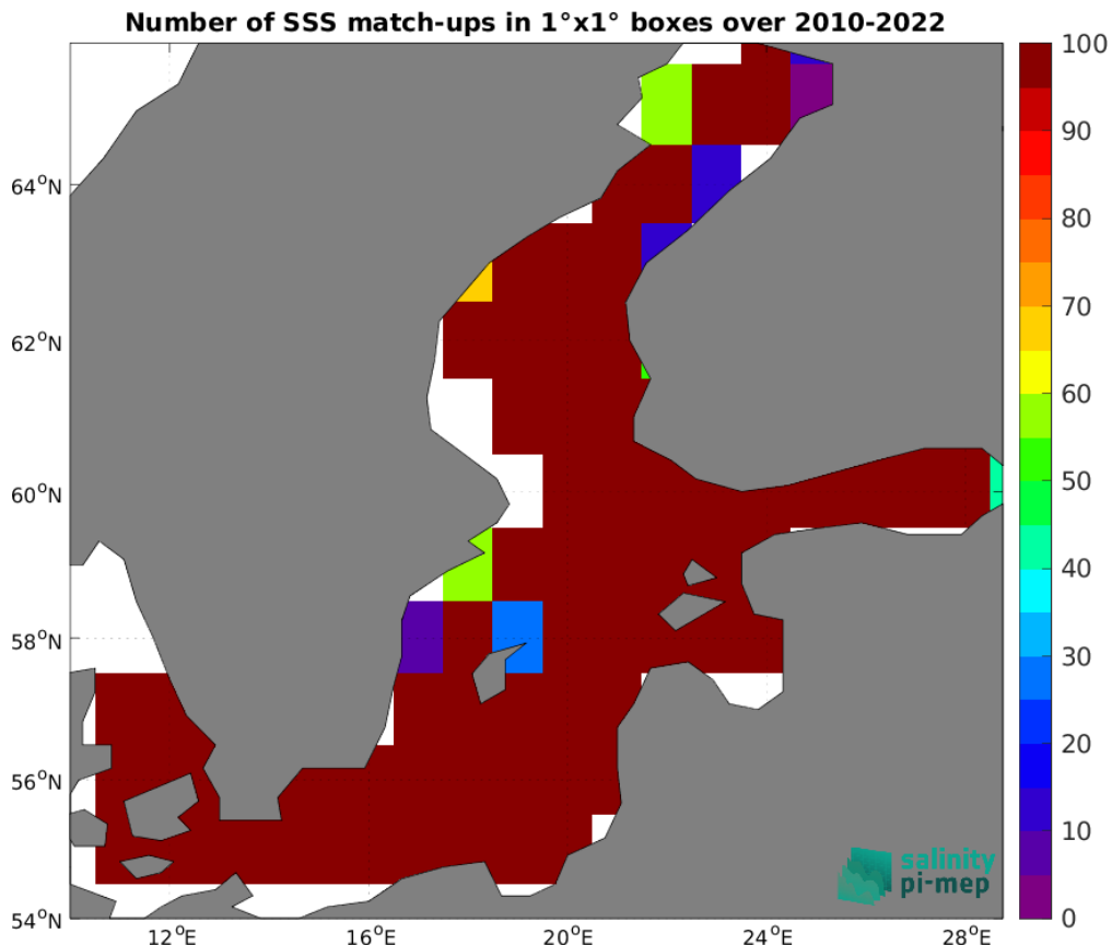
Figure 4: Number of SSS match-ups between ICES SSS and the SMOS SSS L4 v1 - Weekly (CMEMS-CNR) SSS product for the Baltic Sea Pi-MEP region over 1^{\circ} \times 1^{\circ} boxes and for the full satellite product period.
