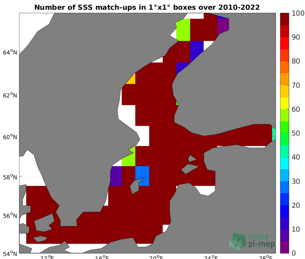
Figure 4: Number of SSS match-ups between ICES SSS and the SMOS SSS L4 v1 - Weekly (CMEMS-CNR) SSS product for the Baltic Sea Pi-MEP region over 1°x1° boxes and for the full satellite product period.
