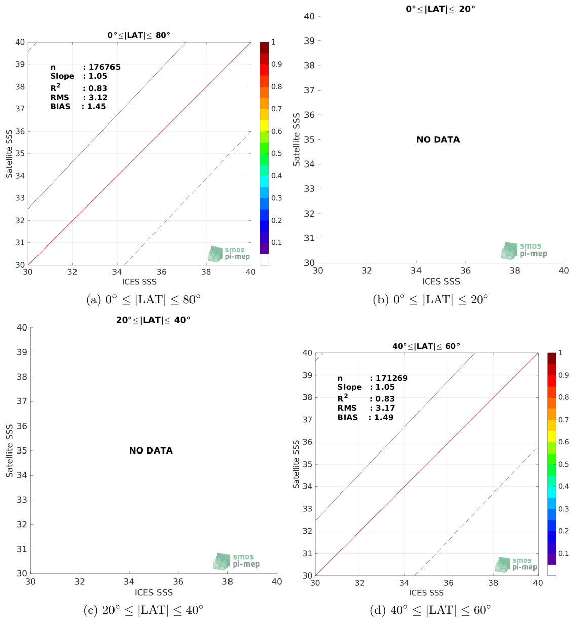
Figure 9: Contour maps of the concentration of SMOS SSS L4 v1 - Weekly (CMEMS-CNR) SSS (y-axis) versus ICES SSS (x-axis) at match-up pairs for different latitude bands. For each plot, the red line shows x=y . The black thin and dashed lines indicate a linear fit through the data cloud and the \pm 95\% confidence levels, respectively. The number match-up pairs n , the slope and R^2 coefficient of the linear fit, the root mean square (RMS) and the mean bias between satellite and in situ data are indicated for each latitude band in each plots.
