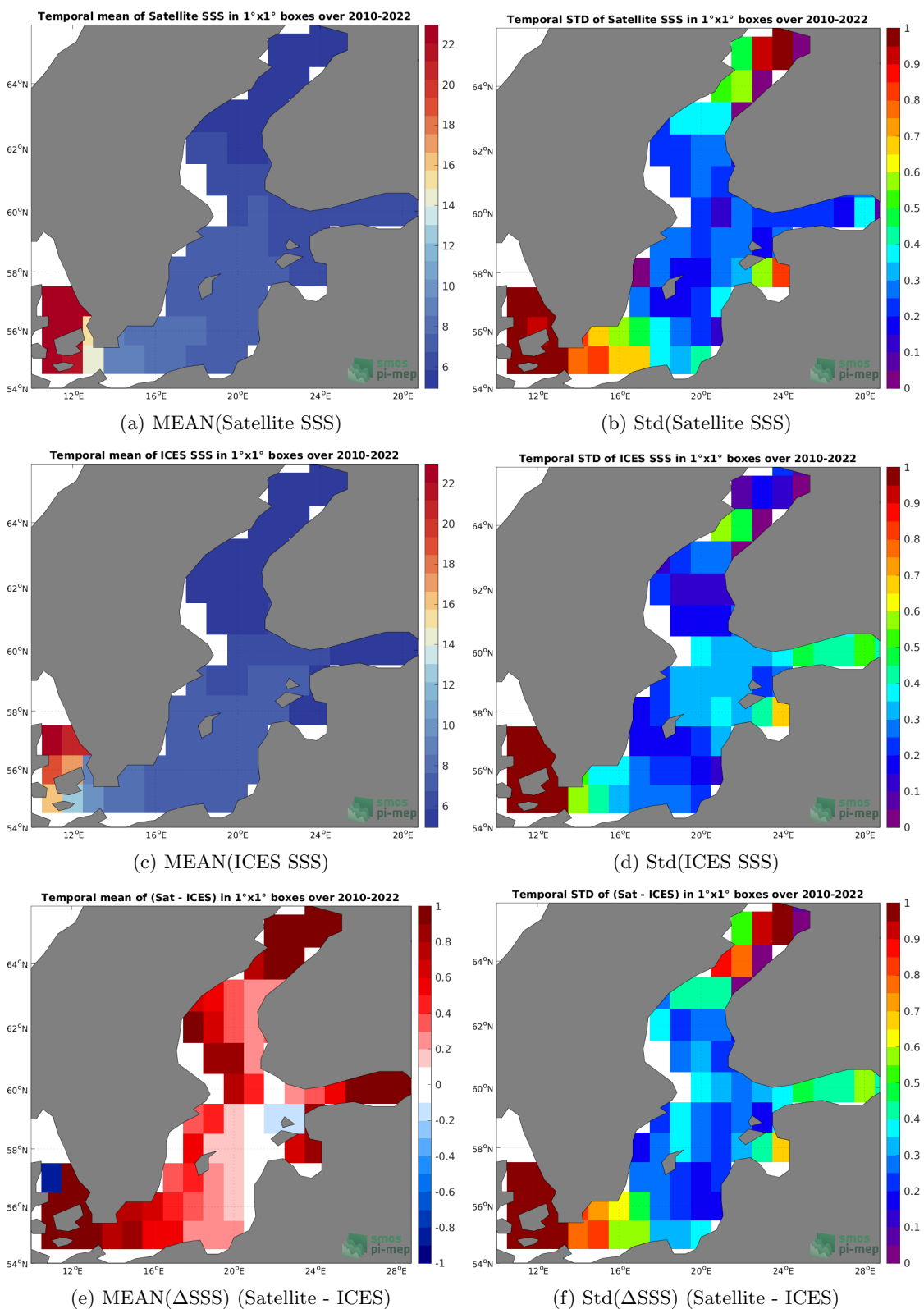
Figure 6: Temporal mean (left) and Std (right) of SSS from SMOS SSS L4 v1 - Weekly (CMEMS-CNR) (top), ICES (middle), and of \Delta SSS (Satellite - ICES). Only match-up pairs are used to generate these maps.
