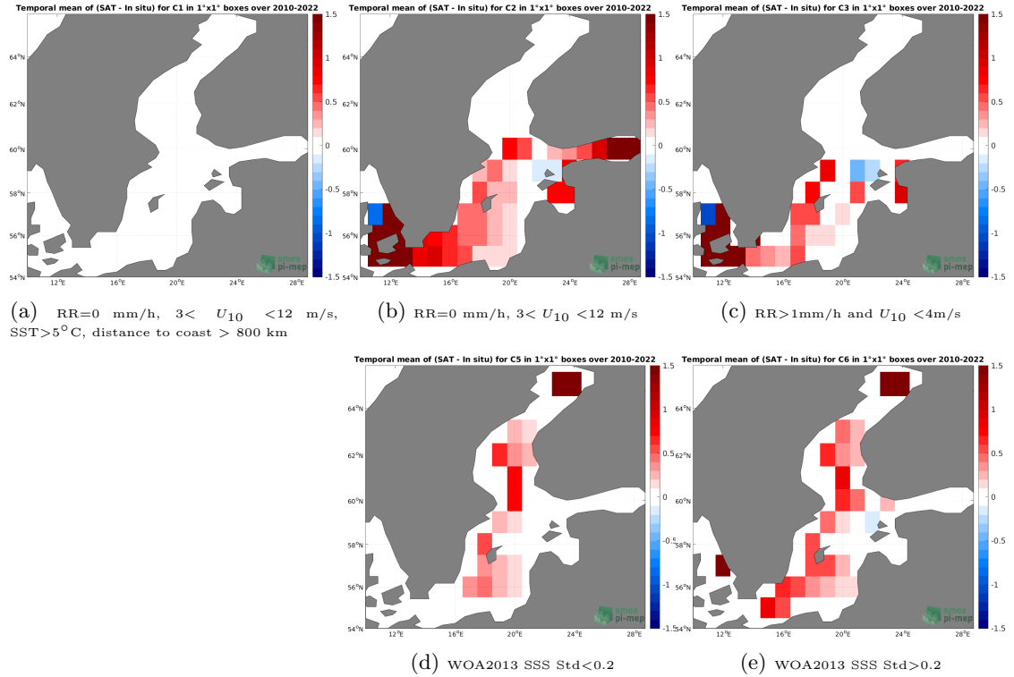
Figure 12: Temporal mean gridded over spatial boxes of size 1^{\circ}\times 1^{\circ} of \Delta\text{SSS} (SMOS SSS L4 v1 - Weekly (CMEMS-CNR) - ICES) for 5 different subdatasets corresponding to:RR=0 mm/h, 3 < U_{10} < 12 m/s, SST > 5^{\circ}\text{C} , distance to coast > 800 km (a), RR=0 mm/h, 3 < U_{10} < 12 m/s (b), RR > 1 mm/h and U_{10} < 4 m/s (c), WOA2013 SSS Std < 0.2 (d), WOA2013 SSS Std > 0.2 (e).
