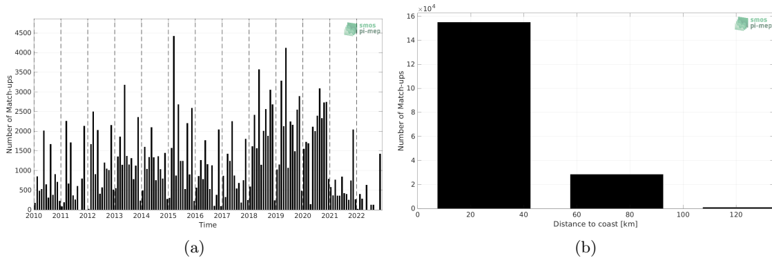
Figure 1: Number of match-ups between ICES and SMOS SSS L4 v1 - Weekly (CMEMS-CNR) SSS as a function of time (a) and as function of the distance to coast (b) over the Baltic Sea Pi-MEP region and for the full satellite product period.
