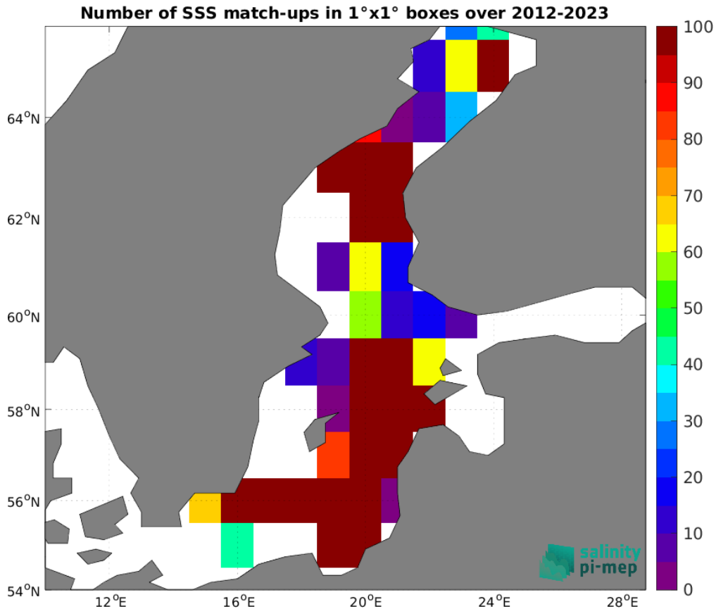
Figure 4: Number of SSS match-ups between Argo SSS and the SMOS SSS L4 v1 - Weekly (CMEMS-CNR) SSS product for the Baltic Sea Pi-MEP region over 1^\circ \times 1^\circ boxes and for the full satellite product period.
