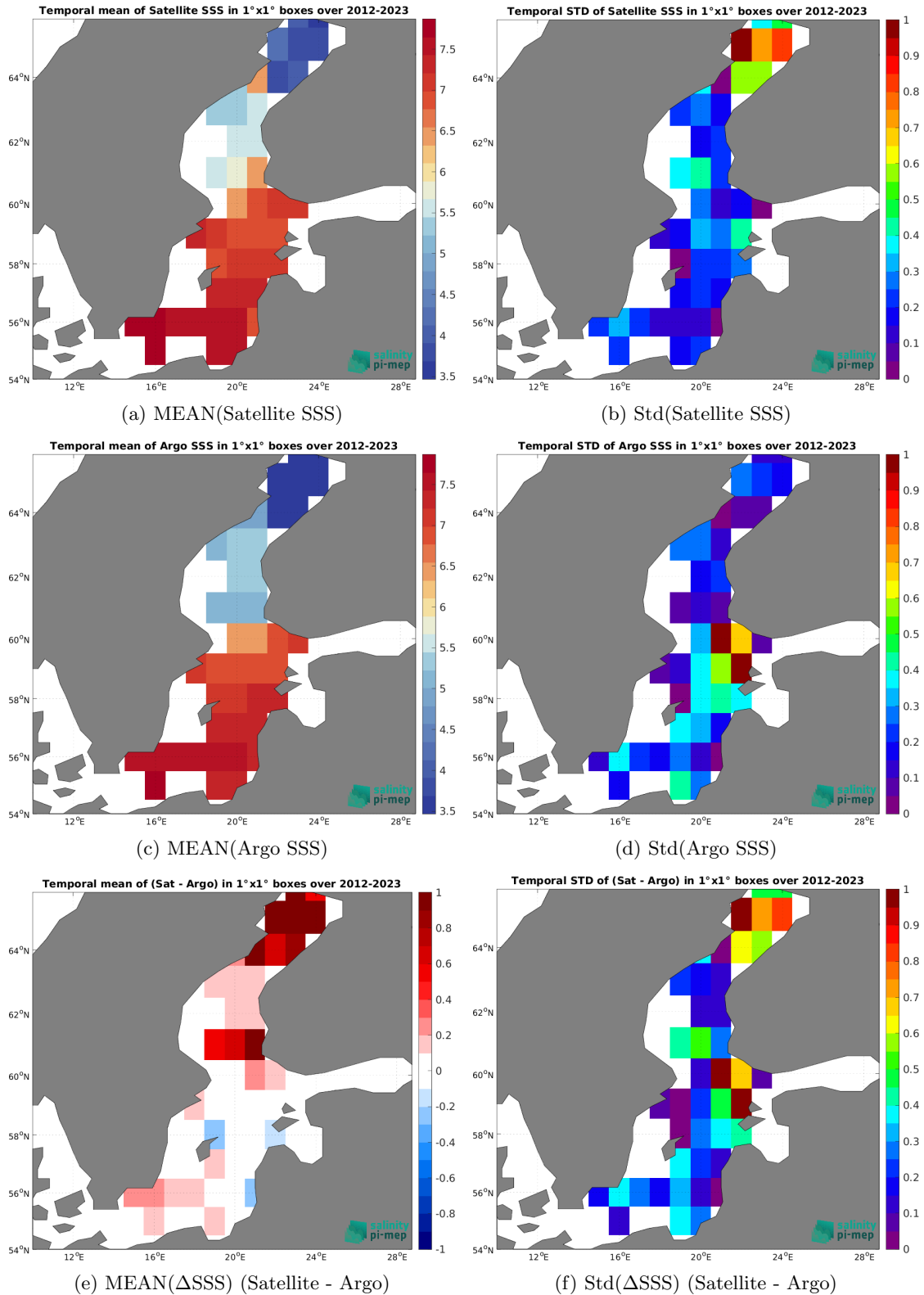
Figure 6: Temporal mean (left) and Std (right) of SSS from SMOS SSS L4 v1 - Weekly (CMEMS-CNR) (top), Argo (middle), and of \Delta SSS (Satellite - Argo). Only match-up pairs are used to generate these maps.
