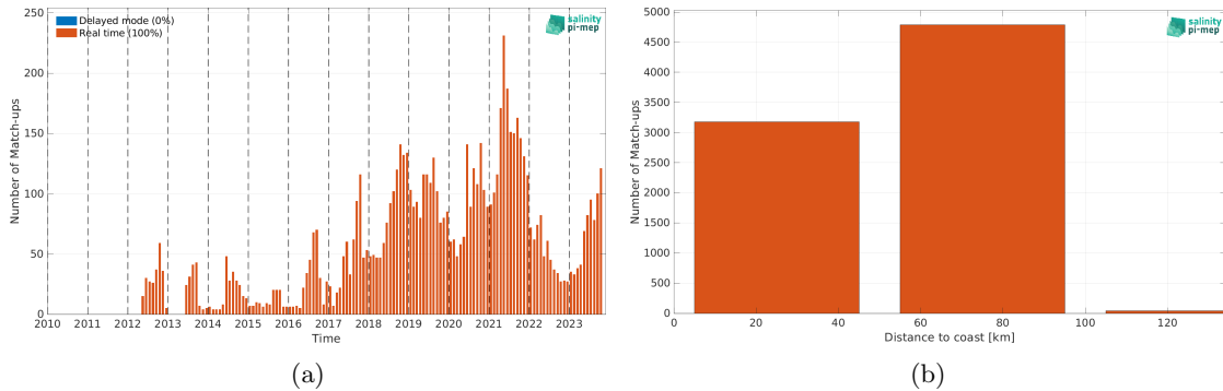
Figure 1: Number of match-ups between Argo and SMOS SSS L4 v1 - Weekly (CMEMS-CNR) SSS as a function of time (a) and as function of the distance to coast (b) over the Baltic Sea Pi-MEP region and for the full satellite product period.
