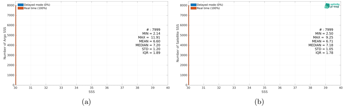
Figure 2: Histograms of SSS from Argo (a) and SMOS SSS L4 v1 - Weekly (CMEMS-CNR) (b) considering all match-up pairs per bins of 0.1 over the Baltic Sea Pi-MEP region and for the full satellite product period.
