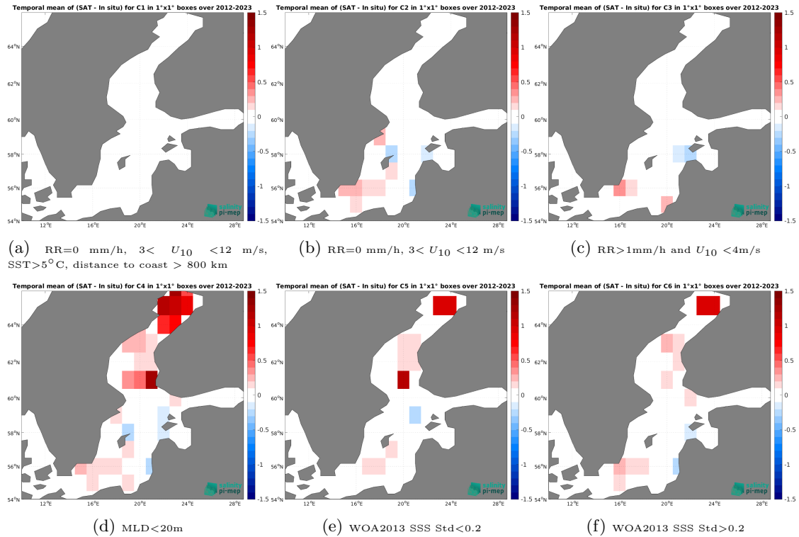
Figure 12: Temporal mean gridded over spatial boxes of size 1^{\circ}\times 1^{\circ} of \Delta\text{SSS} (SMOS SSS L4 v1 - Weekly (CMEMS-CNR) - Argo) for 6 different subdatasets corresponding to:RR=0 mm/h, 3 < U_{10} < 12 m/s, SST >5^{\circ}\text{C} , distance to coast > 800 km (a), RR=0 mm/h, 3 < U_{10} < 12 m/s (b), RR >1\text{mm/h} and U_{10} < 4\text{m/s} (c),MLD <20\text{m} (d),WOA2013 SSS Std <0.2 (e),WOA2013 SSS Std >0.2 (f).
