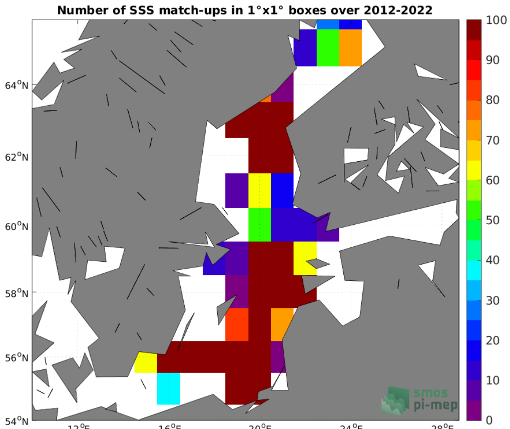
Figure 4: Number of SSS match-ups between Argo SSS and the SMOS SSS L4 v1 - Weekly (CMEMS-CNR) SSS product for the Baltic Sea Pi-MEP region over 1°x1° boxes and for the full satellite product period.
