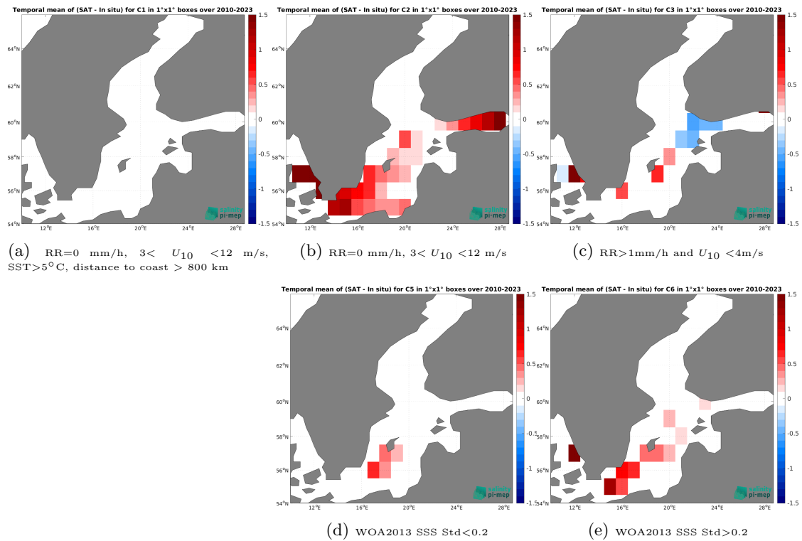
Figure 14: Temporal mean gridded over spatial boxes of size 1^\circ \times 1^\circ of \Delta\text{SSS} (SMOS SSS L4 v1 - Monthly (CMEMS-CNR) - TSG (LEGOS-DM)) for 5 different subdatasets corresponding to:RR=0 mm/h, 3 < U_{10} < 12 m/s, SST>5°C, distance to coast > 800 km (a), RR=0 mm/h, 3 < U_{10} < 12 m/s (b), RR>1mm/h and U_{10} < 4 m/s (c), WOA2013 SSS Std<0.2 (d), WOA2013 SSS Std>0.2 (e).
