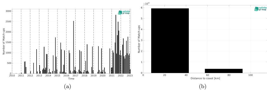
Figure 1: Number of match-ups between TSG (LEGOS-DM) and SMOS SSS L4 v1 - Monthly (CMEMS-CNR) SSS as a function of time (a) and as function of the distance to coast (b) over the Baltic Sea Pi-MEP region and for the full satellite product period.
