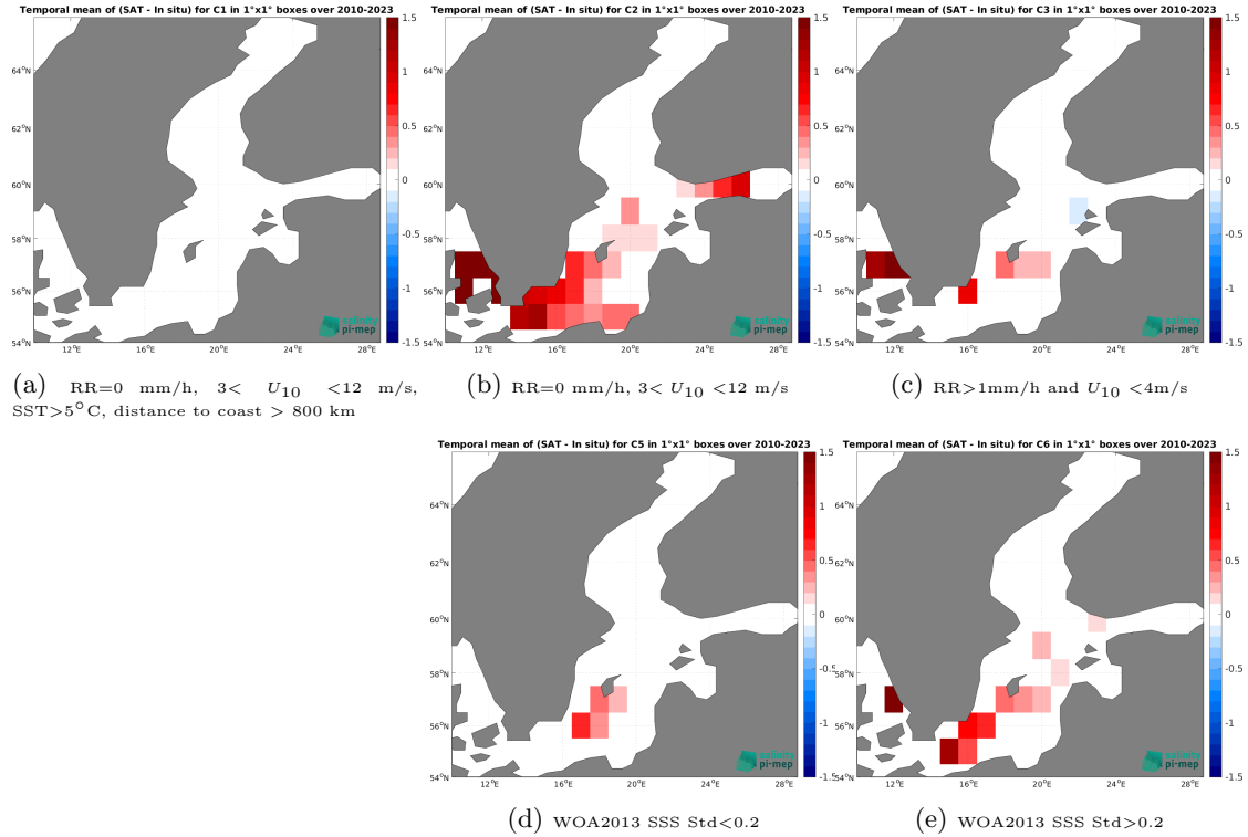
Figure 12: Temporal mean gridded over spatial boxes of size 1^{\circ}\times 1^{\circ} of \Delta\text{SSS} (SMOS SSS L4 v1 - Monthly (CMEMS-CNR) - TSG (LEGOS-DM)) for 5 different subdatasets corresponding to:RR=0 mm/h, 3 < U_{10} < 12 m/s, SST >5^{\circ}\text{C} , distance to coast > 800 km (a), RR=0 mm/h, 3 < U_{10} < 12 m/s (b), RR >1 mm/h and U_{10} < 4 m/s (c), WOA2013 SSS Std <0.2 (d), WOA2013 SSS Std >0.2 (e).
