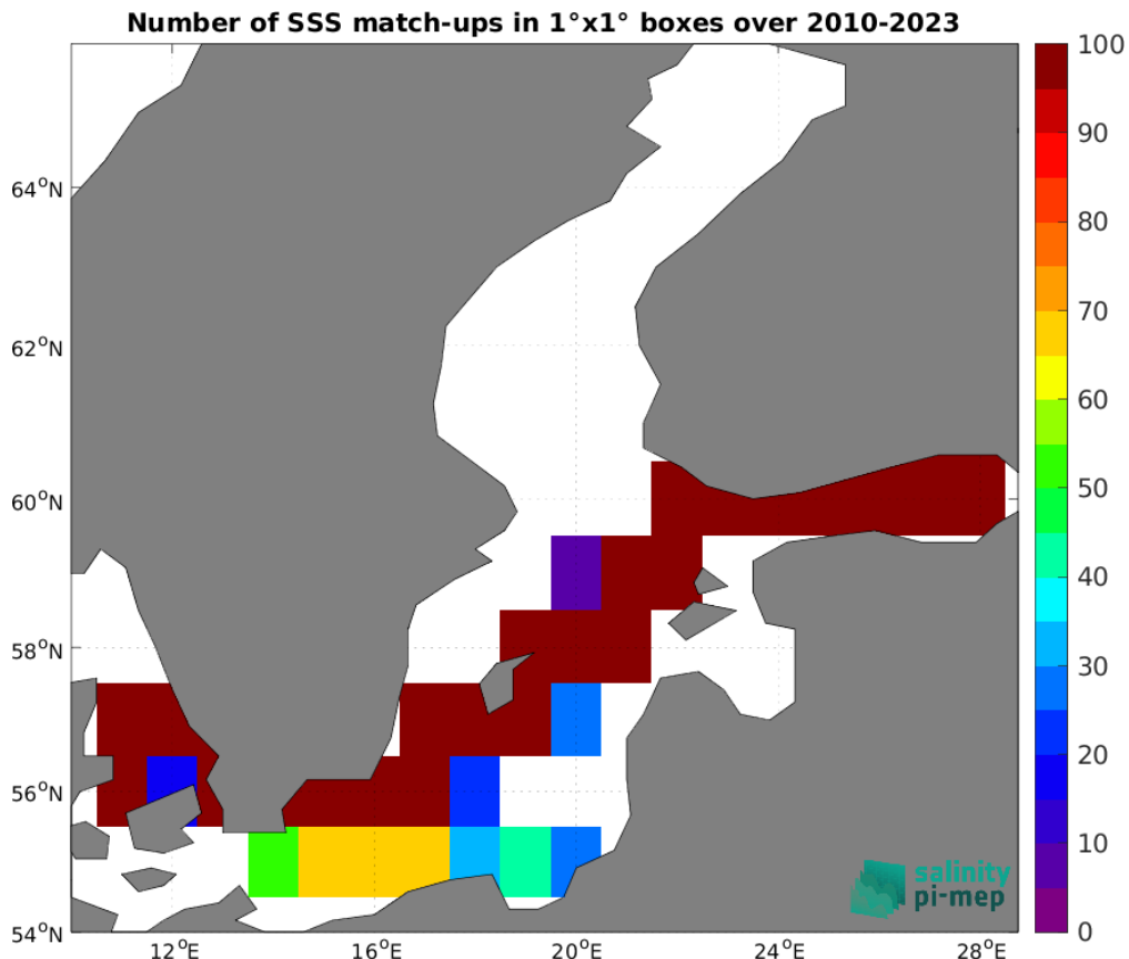
Figure 4: Number of SSS match-ups between TSG (LEGOS-DM) SSS and the SMOS SSS L4 v1 - Monthly (CMEMS-CNR) SSS product for the Baltic Sea Pi-MEP region over 1^\circ \times 1^\circ boxes and for the full satellite product period.
