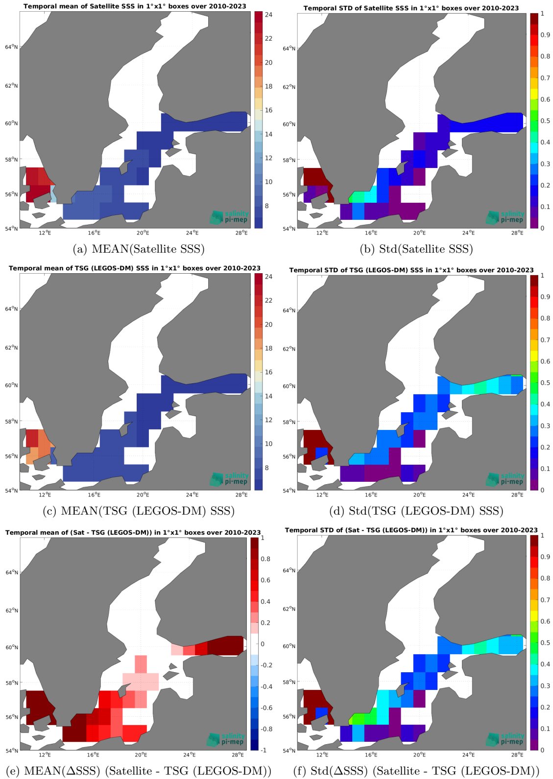
Figure 6: Temporal mean (left) and Std (right) of SSS from SMOS SSS L4 v1 - Monthly (CMEMS-CNR) (top), TSG (LEGOS-DM) (middle), and of \Delta SSS (Satellite - TSG (LEGOS-DM)). Only match-up pairs are used to generate these maps.
