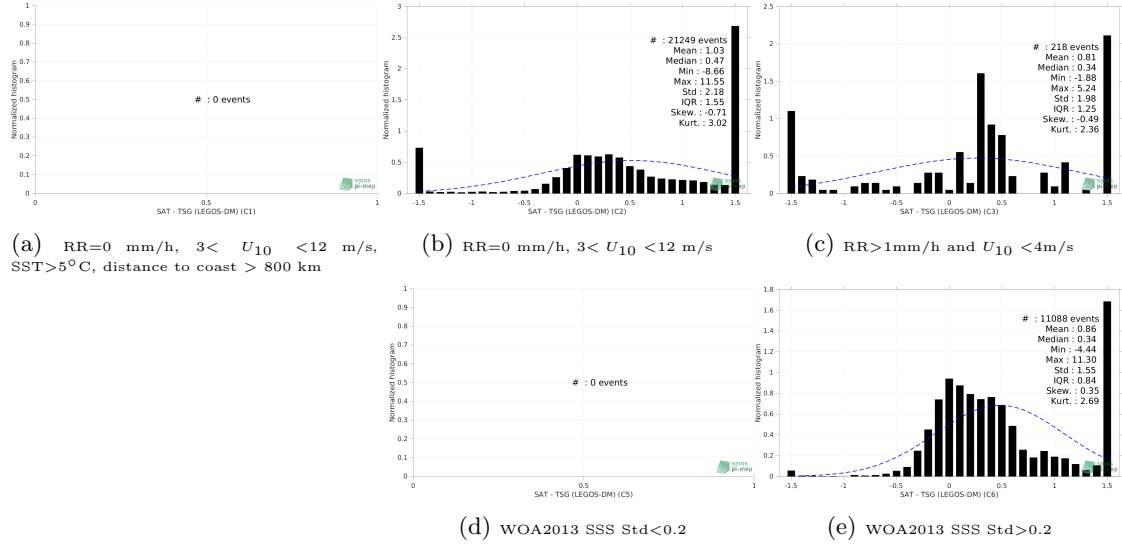
Figure 13: Normalized histogram of \Delta\text{SSS} (SMOS SSS L4 v1 - Monthly (CMEMS-CNR) - TSG (LEGOS-DM)) for 5 different subdatasets corresponding to: RR=0 mm/h, 3 < U_{10} < 12 m/s, SST > 5^\circ\text{C} , distance to coast > 800 km (a), RR=0 mm/h, 3 < U_{10} < 12 m/s (b), RR > 1\text{mm/h} and U_{10} < 4\text{m/s} (c), WOA2013 SSS \text{Std} < 0.2 (d), WOA2013 SSS \text{Std} > 0.2 (e).
