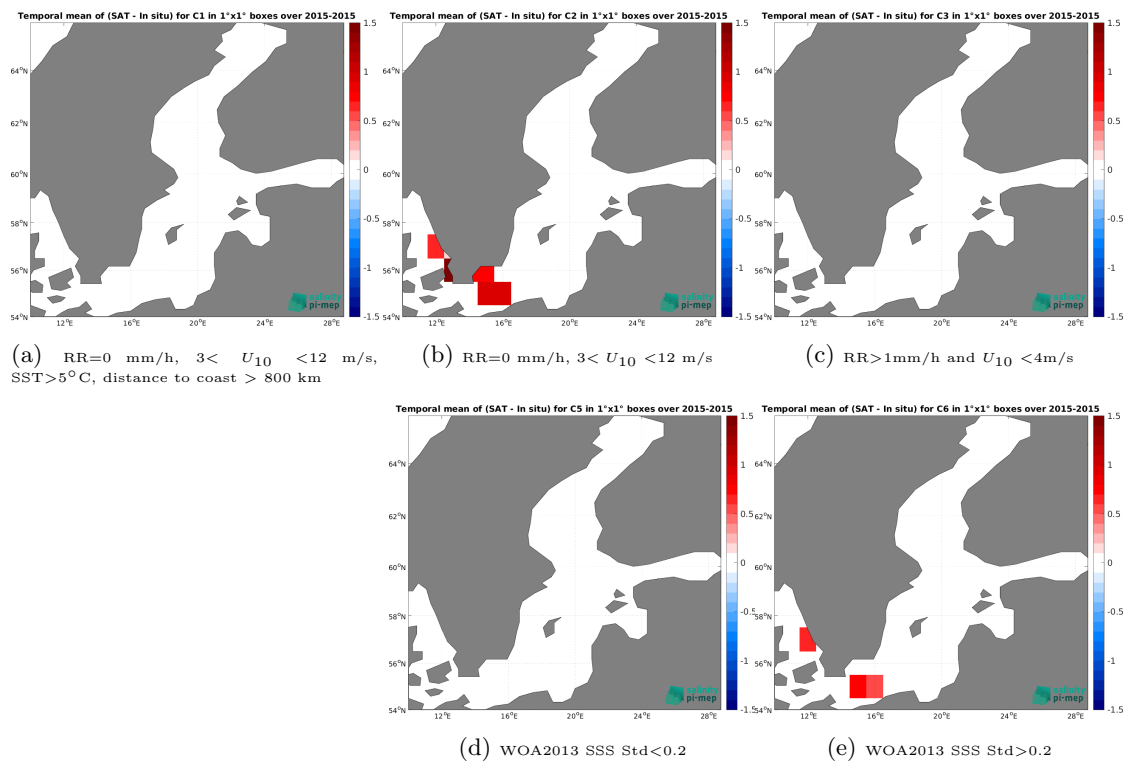
Figure 14: Temporal mean gridded over spatial boxes of size 1^\circ \times 1^\circ of \Delta SSS (SMOS SSS L4 v1 - Monthly (CMEMS-CNR) - TSG (GOSUD-Research-vessel)) for 5 different subdatasets corresponding to:RR=0 mm/h, 3 < U_{10} < 12 m/s, SST >5^\circ\text{C} , distance to coast > 800 km (a), RR=0 mm/h, 3 < U_{10} < 12 m/s (b), RR >1 mm/h and U_{10} < 4 m/s (c), WOA2013 SSS Std <0.2 (d), WOA2013 SSS Std >0.2 (e).
