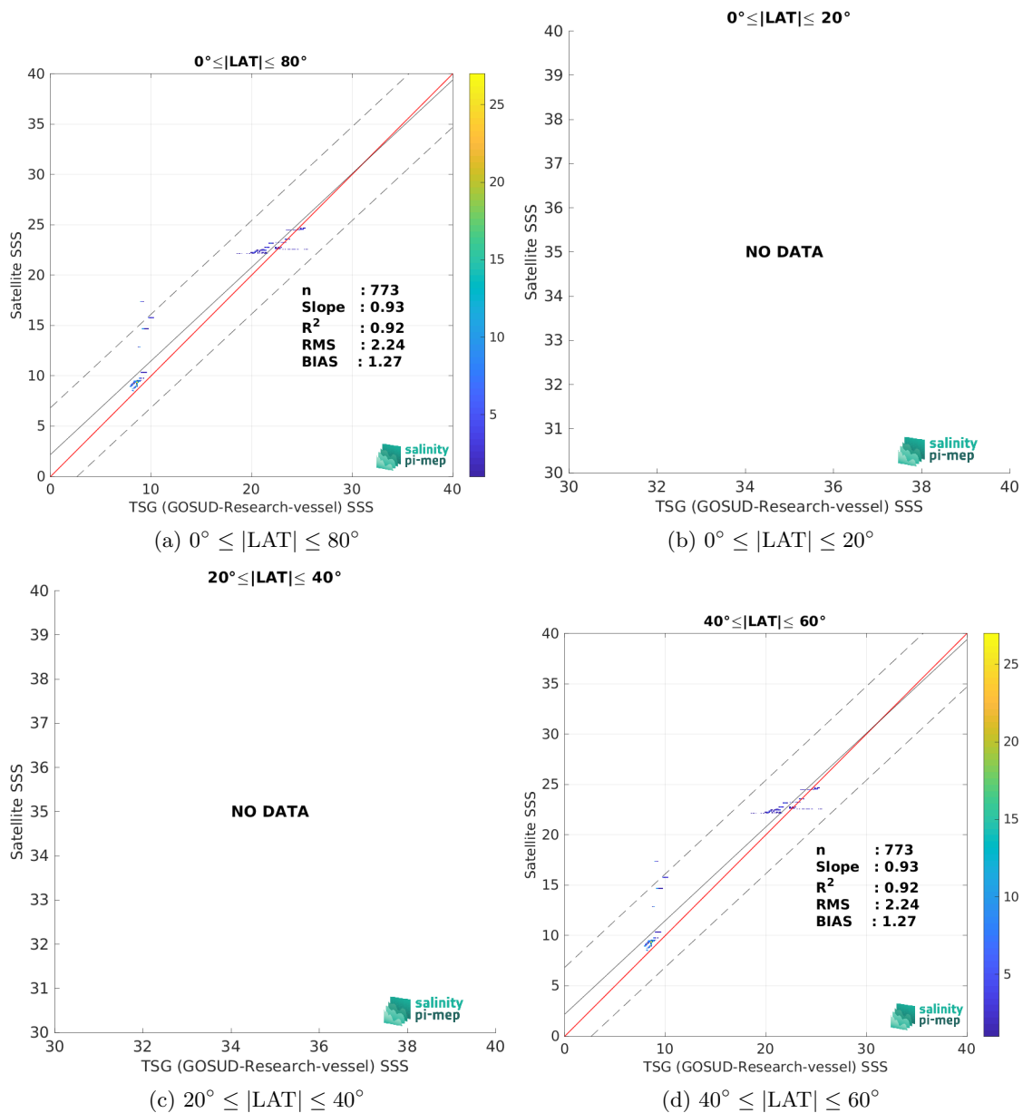
Figure 10: Contour maps of the concentration of SMOS SSS L4 v1 - Monthly (CMEMS-CNR) SSS (y-axis) versus TSG (GOSUD-Research-vessel) SSS (x-axis) at match-up pairs for different latitude bands. For each plot, the red line shows x=y . The black thin and dashed lines indicate a linear fit through the data cloud and the \pm 95\% confidence levels, respectively. The number match-up pairs n , the slope and R^2 coefficient of the linear fit, the root mean square (RMS) and the mean bias between satellite and in situ data are indicated for each latitude band in each plots.
