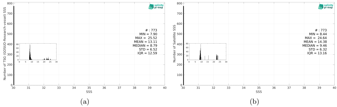
Figure 3: Histograms of SSS from TSG (GOSUD-Research-vessel) (a) and SMOS SSS L4 v1 - Monthly (CMEMS-CNR) (b) considering all match-up pairs per bins of 0.1 over the Baltic Sea Pi-MEP region and for the full satellite product period.
