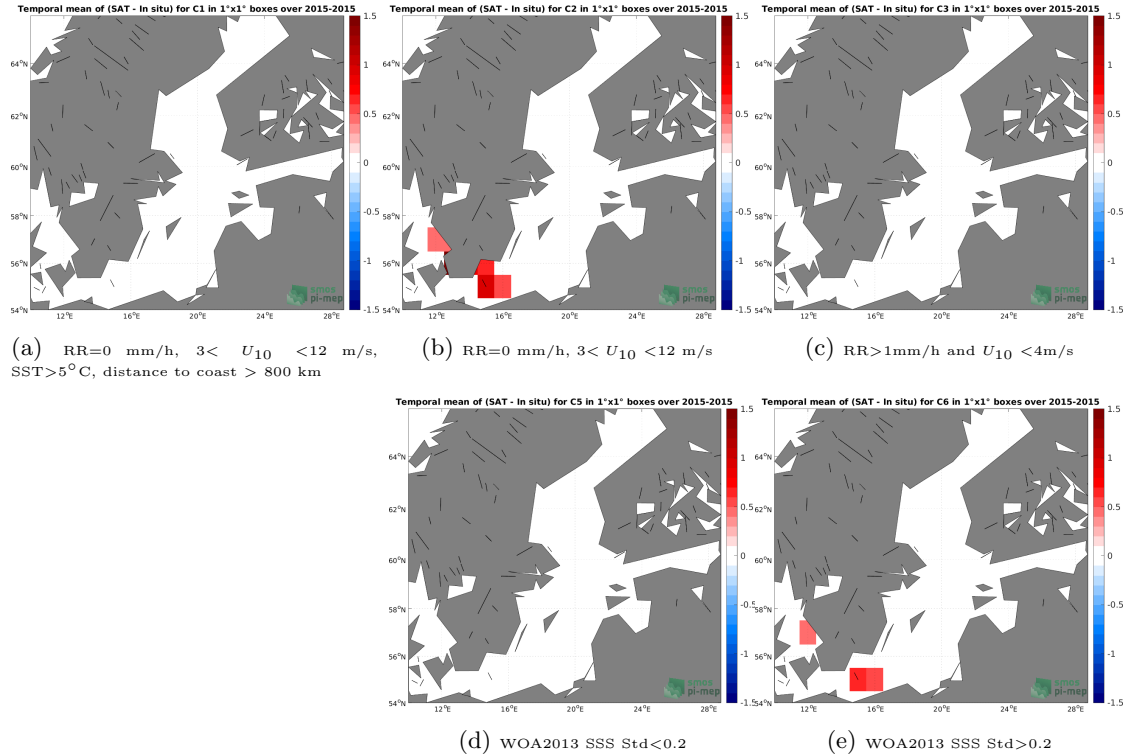
Figure 12: Temporal mean gridded over spatial boxes of size 1^\circ \times 1^\circ of \Delta SSS (SMOS SSS L4 v1 - Monthly (CMEMS-CNR) - TSG (GOSUD-Research-vessel)) for 5 different subdatasets corresponding to:RR=0 mm/h, 3 < U_{10} < 12 m/s, SST > 5^\circ\text{C} , distance to coast > 800 km (a), RR=0 mm/h, 3 < U_{10} < 12 m/s (b), RR > 1 mm/h and U_{10} < 4 m/s (c), WOA2013 SSS Std < 0.2 (d), WOA2013 SSS Std > 0.2 (e).
