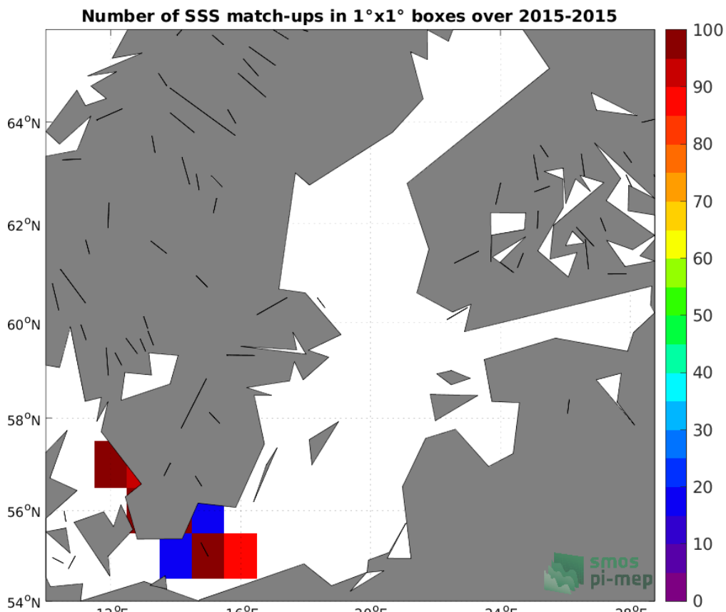
Figure 4: Number of SSS match-ups between TSG (GOSUD-Research-vessel) SSS and the SMOS SSS L4 v1 - Monthly (CMEMS-CNR) SSS product for the Baltic Sea Pi-MEP region over 1^\circ \times 1^\circ boxes and for the full satellite product period.
