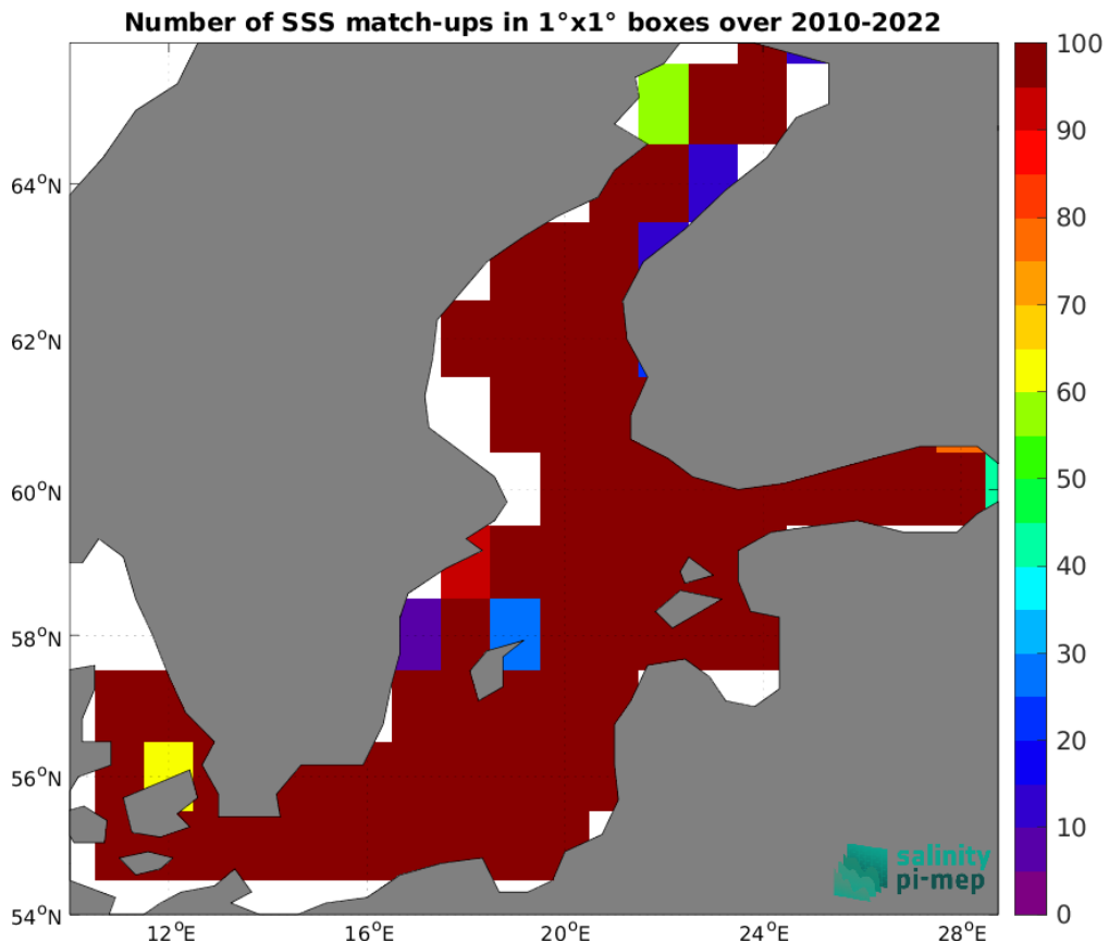
Figure 5: Number of SSS match-ups between ICES SSS and the SMOS SSS L4 v1 - Monthly (CMEMS-CNR) SSS product for the Baltic Sea Pi-MEP region over 1°x1° boxes and for the full satellite product period.
