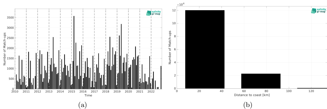
Figure 2: Number of match-ups between ICES and SMOS SSS L4 v1 - Monthly (CMEMS-CNR) SSS as a function of time (a) and as function of the distance to coast (b) over the Baltic Sea Pi-MEP region and for the full satellite product period.
