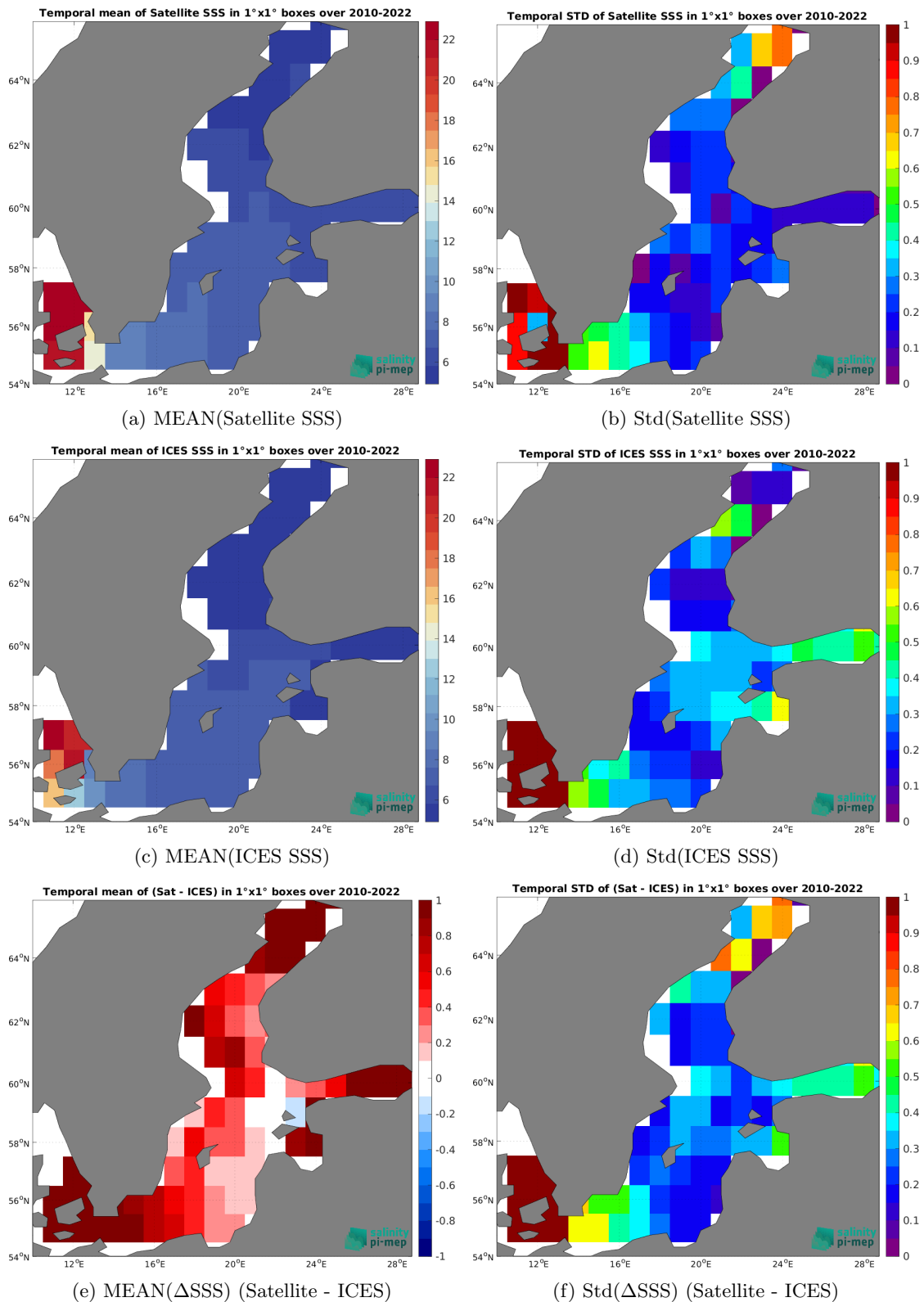
Figure 7: Temporal mean (left) and Std (right) of SSS from SMOS SSS L4 v1 - Monthly (CMEMS-CNR) (top), ICES (middle), and of \Delta SSS (Satellite - ICES). Only match-up pairs are used to generate these maps.
