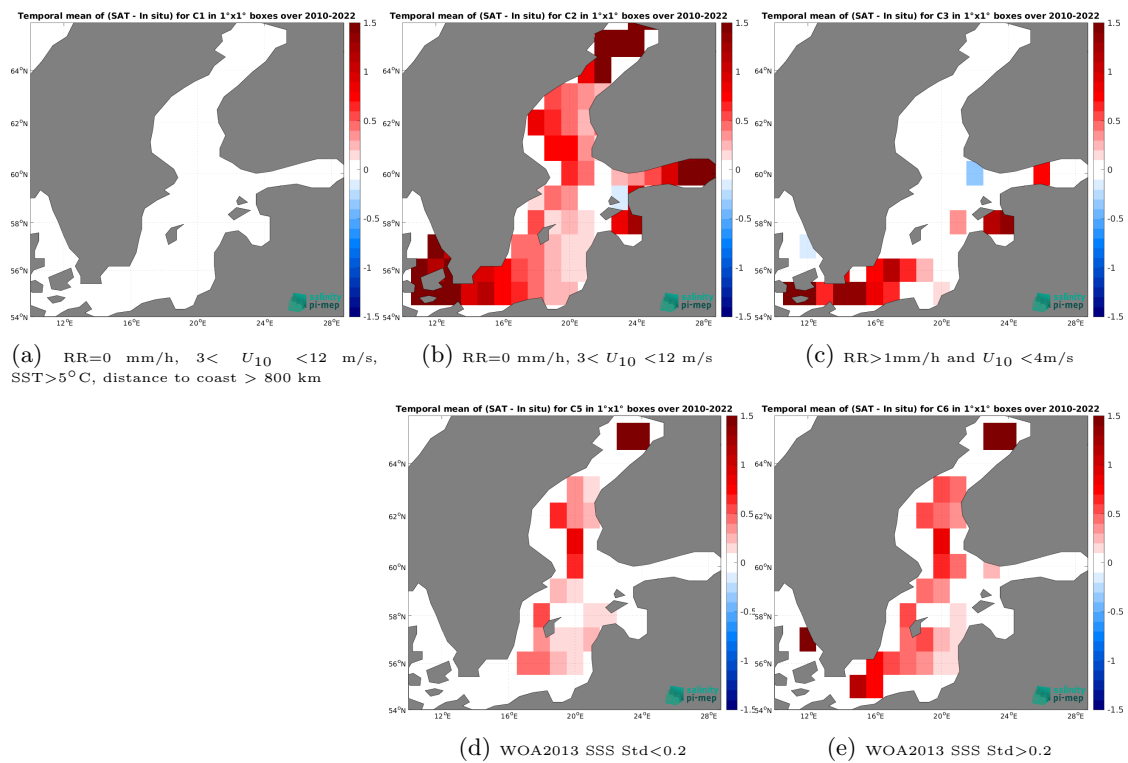
Figure 14: Temporal mean gridded over spatial boxes of size 1^\circ \times 1^\circ of \Delta\text{SSS} (SMOS SSS L4 v1 - Monthly (CMEMS-CNR) - ICES) for 5 different subdatasets corresponding to:RR=0 mm/h, 3 < U_{10} < 12 m/s, SST >5^\circ\text{C} , distance to coast > 800 km (a), RR=0 mm/h, 3 < U_{10} < 12 m/s (b), RR >1 mm/h and U_{10} < 4 m/s (c), WOA2013 SSS Std <0.2 (d), WOA2013 SSS Std >0.2 (e).
