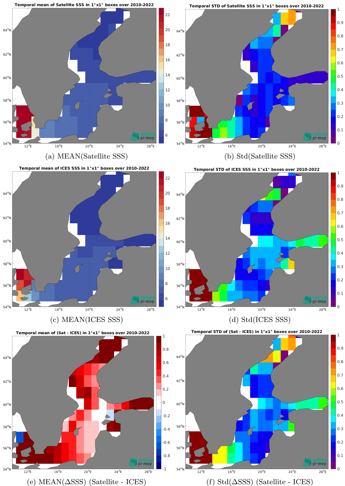
Figure 6: Temporal mean (left) and Std (right) of SSS from SMOS SSS L4 v1 - Monthly (CMEMS-CNR) (top), ICES (middle), and of \Delta SSS (Satellite - ICES). Only match-up pairs are used to generate these maps.
