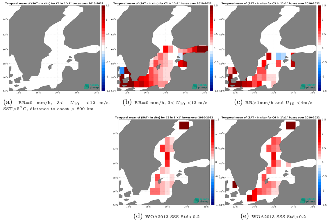
Figure 12: Temporal mean gridded over spatial boxes of size 1^{\circ}\times 1^{\circ} of \Delta\text{SSS} (SMOS SSS L4 v1 - Monthly (CMEMS-CNR) - ICES) for 5 different subdatasets corresponding to: \text{RR}=0 mm/h, 3 < U_{10} < 12 m/s, \text{SST} > 5^{\circ}\text{C} , distance to coast > 800 km (a), \text{RR}=0 mm/h, 3 < U_{10} < 12 m/s (b), \text{RR} > 1\text{mm/h} and U_{10} < 4\text{m/s} (c), WOA2013 SSS Std < 0.2 (d), WOA2013 SSS Std > 0.2 (e).
