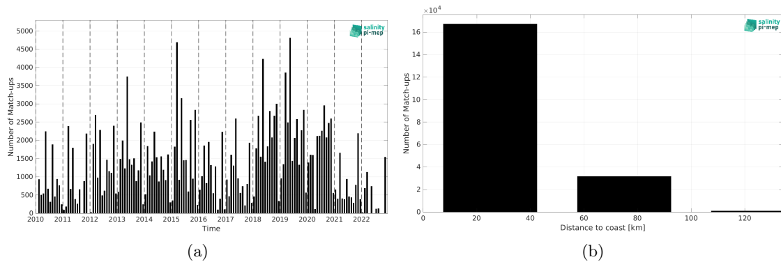
Figure 1: Number of match-ups between ICES and SMOS SSS L4 v1 - Monthly (CMEMS-CNR) SSS as a function of time (a) and as function of the distance to coast (b) over the Baltic Sea Pi-MEP region and for the full satellite product period.
