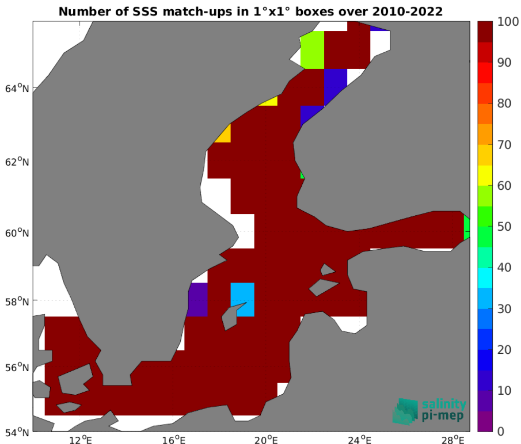
Figure 4: Number of SSS match-ups between ICES SSS and the SMOS SSS L4 v1 - Monthly (CMEMS-CNR) SSS product for the Baltic Sea Pi-MEP region over 1°x1° boxes and for the full satellite product period.
