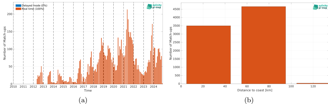
Figure 2: Number of match-ups between Argo and SMOS SSS L4 v1 - Monthly (CMEMS-CNR) SSS as a function of time (a) and as function of the distance to coast (b) over the Baltic Sea Pi-MEP region and for the full satellite product period.
