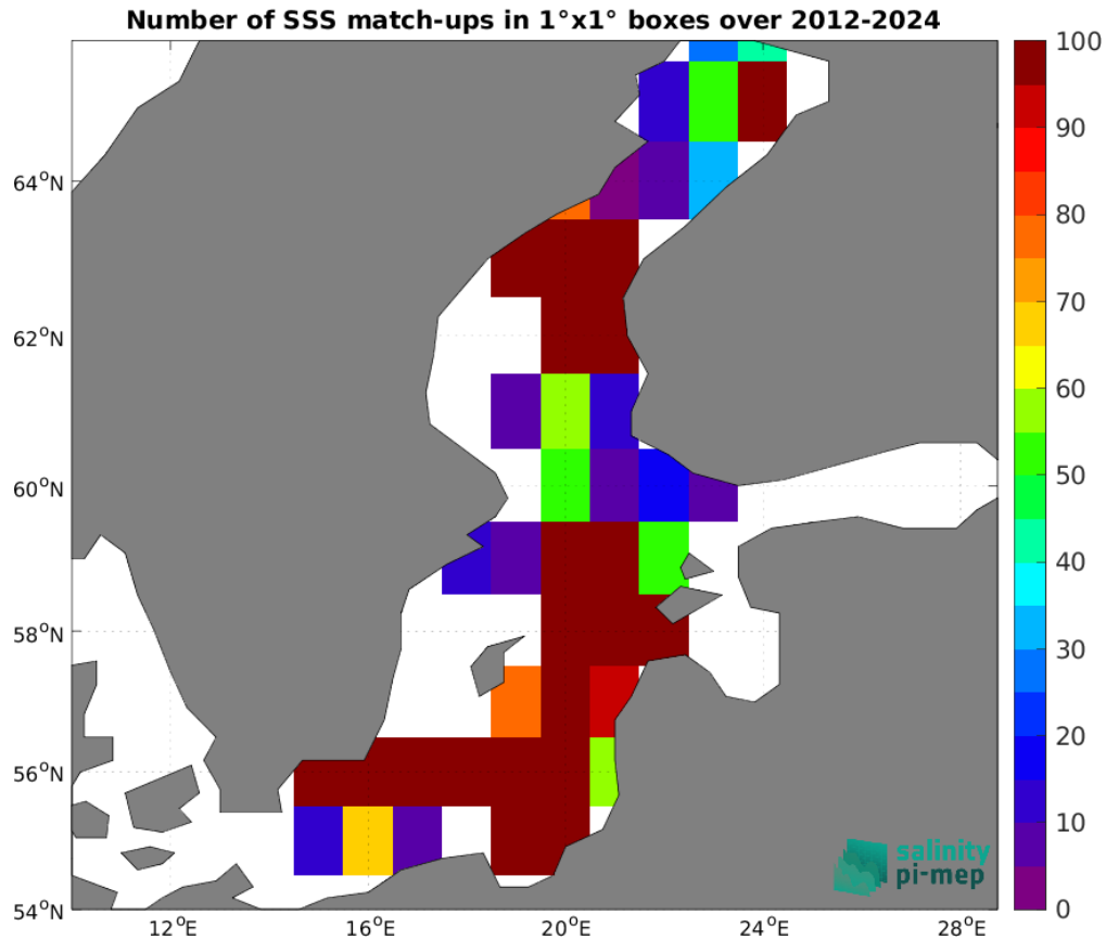
Figure 5: Number of SSS match-ups between Argo SSS and the SMOS SSS L4 v1 - Monthly (CMEMS-CNR) SSS product for the Baltic Sea Pi-MEP region over 1^\circ \times 1^\circ boxes and for the full satellite product period.
