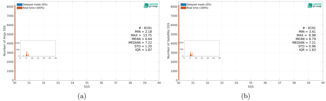
Figure 3: Histograms of SSS from Argo (a) and SMOS SSS L4 v1 - Monthly (CMEMS-CNR) (b) considering all match-up pairs per bins of 0.1 over the Baltic Sea Pi-MEP region and for the full satellite product period.
