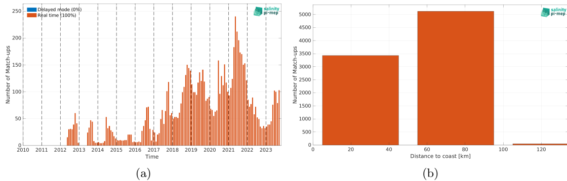
Figure 1: Number of match-ups between Argo and SMOS SSS L4 v1 - Monthly (CMEMS-CNR) SSS as a function of time (a) and as function of the distance to coast (b) over the Baltic Sea Pi-MEP region and for the full satellite product period.
