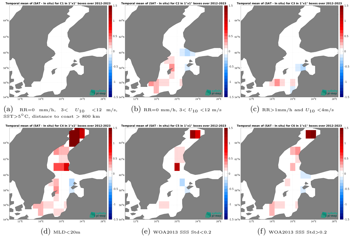
Figure 12: Temporal mean gridded over spatial boxes of size 1^{\circ}\times 1^{\circ} of \Delta\text{SSS} (SMOS SSS L4 v1 - Monthly (CMEMS-CNR) - Argo) for 6 different subdatasets corresponding to:RR=0 mm/h, 3 < U_{10} < 12 m/s, SST >5^{\circ}\text{C} , distance to coast > 800 km (a), RR=0 mm/h, 3 < U_{10} < 12 m/s (b), RR >1\text{mm/h} and U_{10} < 4\text{m/s} (c),MLD <20\text{m} (d),WOA2013 SSS Std <0.2 (e),WOA2013 SSS Std >0.2 (f).
