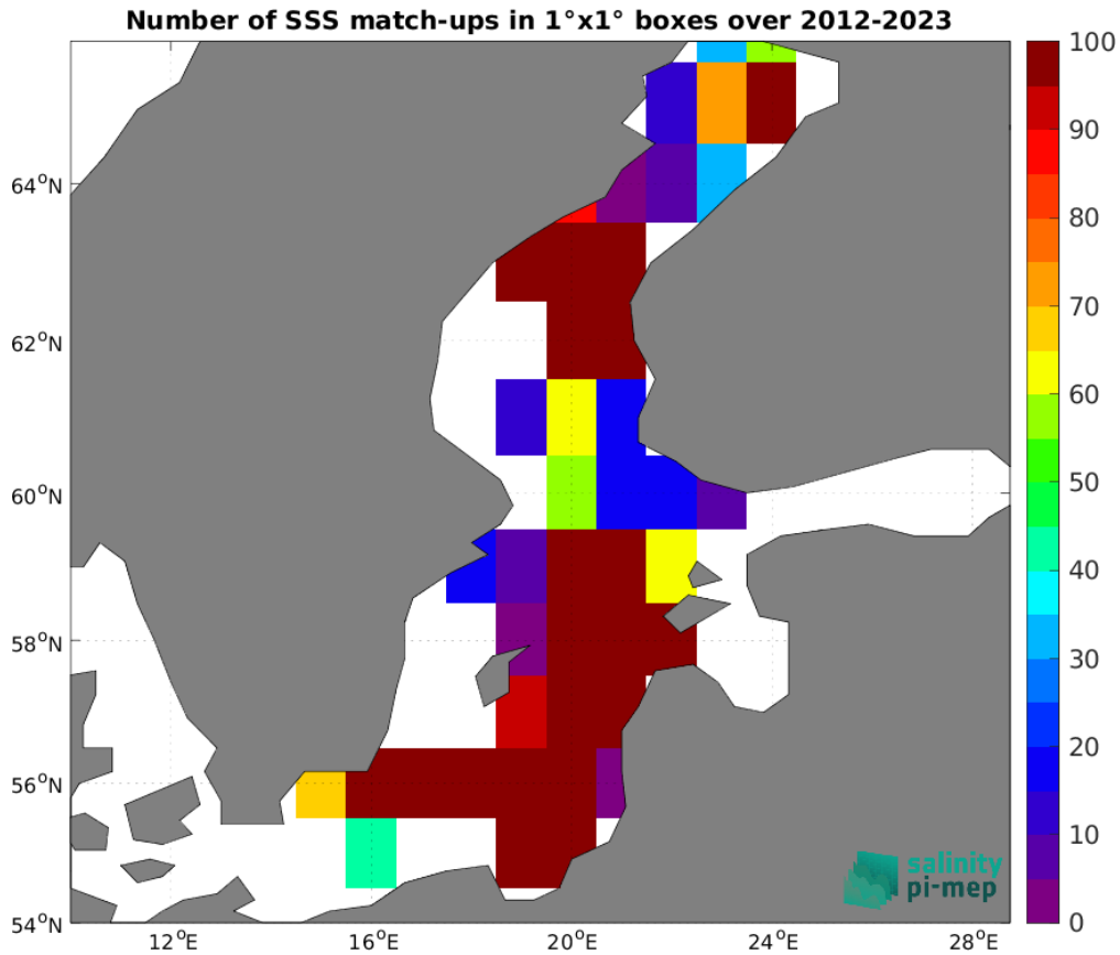
Figure 4: Number of SSS match-ups between Argo SSS and the SMOS SSS L4 v1 - Monthly (CMEMS-CNR) SSS product for the Baltic Sea Pi-MEP region over 1^\circ \times 1^\circ boxes and for the full satellite product period.
