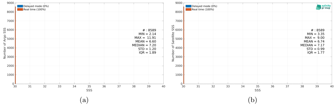
Figure 2: Histograms of SSS from Argo (a) and SMOS SSS L4 v1 - Monthly (CMEMS-CNR) (b) considering all match-up pairs per bins of 0.1 over the Baltic Sea Pi-MEP region and for the full satellite product period.
