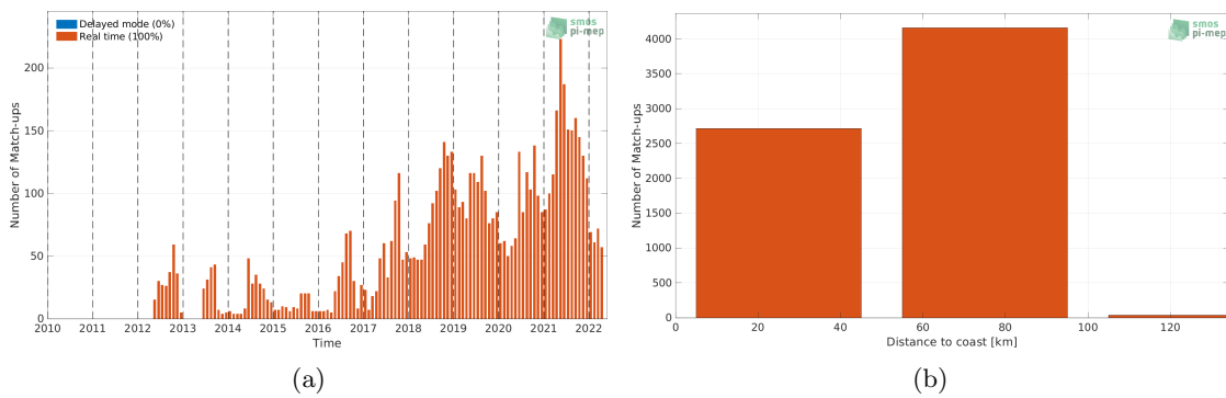
Figure 1: Number of match-ups between Argo and SMOS SSS L4 v1 - Monthly (CMEMS-CNR) SSS as a function of time (a) and as function of the distance to coast (b) over the Baltic Sea Pi-MEP region and for the full satellite product period.
