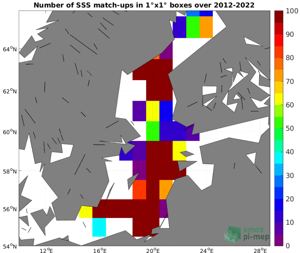
Figure 4: Number of SSS match-ups between Argo SSS and the SMOS SSS L4 v1 - Monthly (CMEMS-CNR) SSS product for the Baltic Sea Pi-MEP region over 1°x1° boxes and for the full satellite product period.
