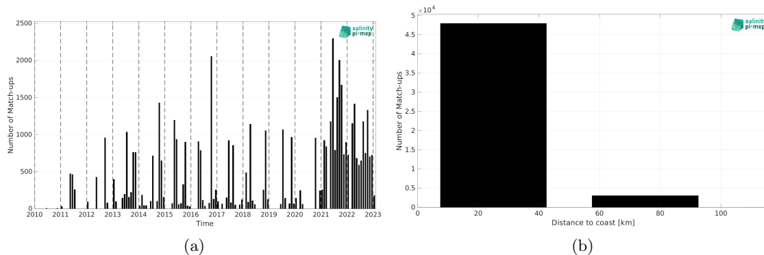
Figure 2: Number of match-ups between TSG (LEGOS-DM) and SMOS SSS L4 v1 - Daily (CMEMS-CNR) SSS as a function of time (a) and as function of the distance to coast (b) over the Baltic Sea Pi-MEP region and for the full satellite product period.
