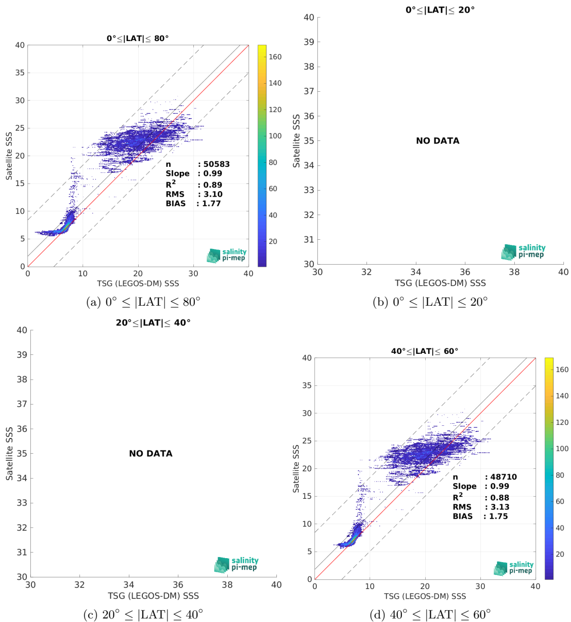
Figure 10: Contour maps of the concentration of SMOS SSS L4 v1 - Daily (CMEMS-CNR) SSS (y-axis) versus TSG (LEGOS-DM) SSS (x-axis) at match-up pairs for different latitude bands. For each plot, the red line shows x=y . The black thin and dashed lines indicate a linear fit through the data cloud and the \pm 95\% confidence levels, respectively. The number match-up pairs n , the slope and R^2 coefficient of the linear fit, the root mean square (RMS) and the mean bias between satellite and in situ data are indicated for each latitude band in each plots.
