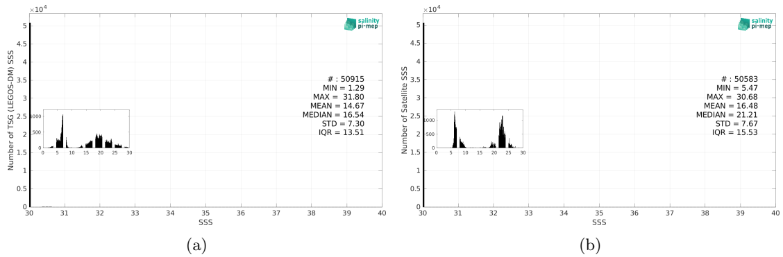
Figure 3: Histograms of SSS from TSG (LEGOS-DM) (a) and SMOS SSS L4 v1 - Daily (CMEMS-CNR) (b) considering all match-up pairs per bins of 0.1 over the Baltic Sea Pi-MEP region and for the full satellite product period.
