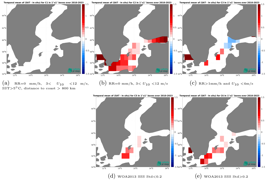
Figure 14: Temporal mean gridded over spatial boxes of size 1^\circ \times 1^\circ of \Delta SSS (SMOS SSS L4 v1 - Daily (CMEMS-CNR) - TSG (LEGOS-DM)) for 5 different subdatasets corresponding to:RR=0 mm/h, 3 < U_{10} < 12 m/s, SST >5^\circ\text{C} , distance to coast > 800 km (a), RR=0 mm/h, 3 < U_{10} < 12 m/s (b), RR >1 mm/h and U_{10} < 4 m/s (c), WOA2013 SSS Std <0.2 (d), WOA2013 SSS Std >0.2 (e).
