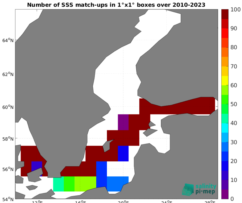
Figure 5: Number of SSS match-ups between TSG (LEGOS-DM) SSS and the SMOS SSS L4 v1 - Daily (CMEMS-CNR) SSS product for the Baltic Sea Pi-MEP region over 1°x1° boxes and for the full satellite product period.
