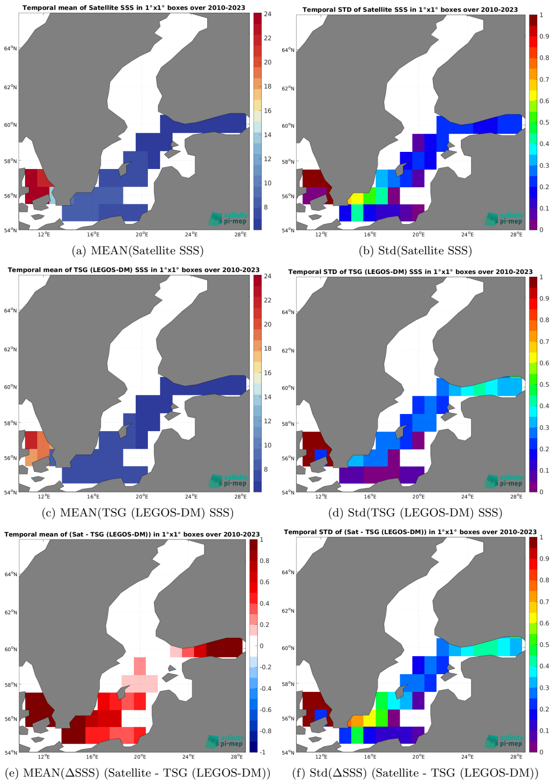
Figure 7: Temporal mean (left) and Std (right) of SSS from SMOS SSS L4 v1 - Daily (CMEMS-CNR) (top), TSG (LEGOS-DM) (middle), and of \Delta SSS (Satellite - TSG (LEGOS-DM)). Only match-up pairs are used to generate these maps.
