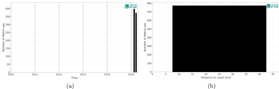
Figure 2: Number of match-ups between TSG (GOSUD-Research-vessel) and SMOS SSS L4 v1 - Daily (CMEMS-CNR) SSS as a function of time (a) and as function of the distance to coast (b) over the Baltic Sea Pi-MEP region and for the full satellite product period.
