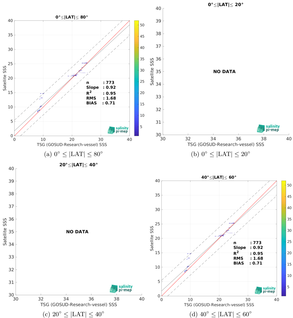
Figure 10: Contour maps of the concentration of SMOS SSS L4 v1 - Daily (CMEMS-CNR) SSS (y-axis) versus TSG (GOSUD-Research-vessel) SSS (x-axis) at match-up pairs for different latitude bands. For each plot, the red line shows x=y . The black thin and dashed lines indicate a linear fit through the data cloud and the \pm 95\% confidence levels, respectively. The number match-up pairs n , the slope and R^2 coefficient of the linear fit, the root mean square (RMS) and the mean bias between satellite and in situ data are indicated for each latitude band in each plots.
