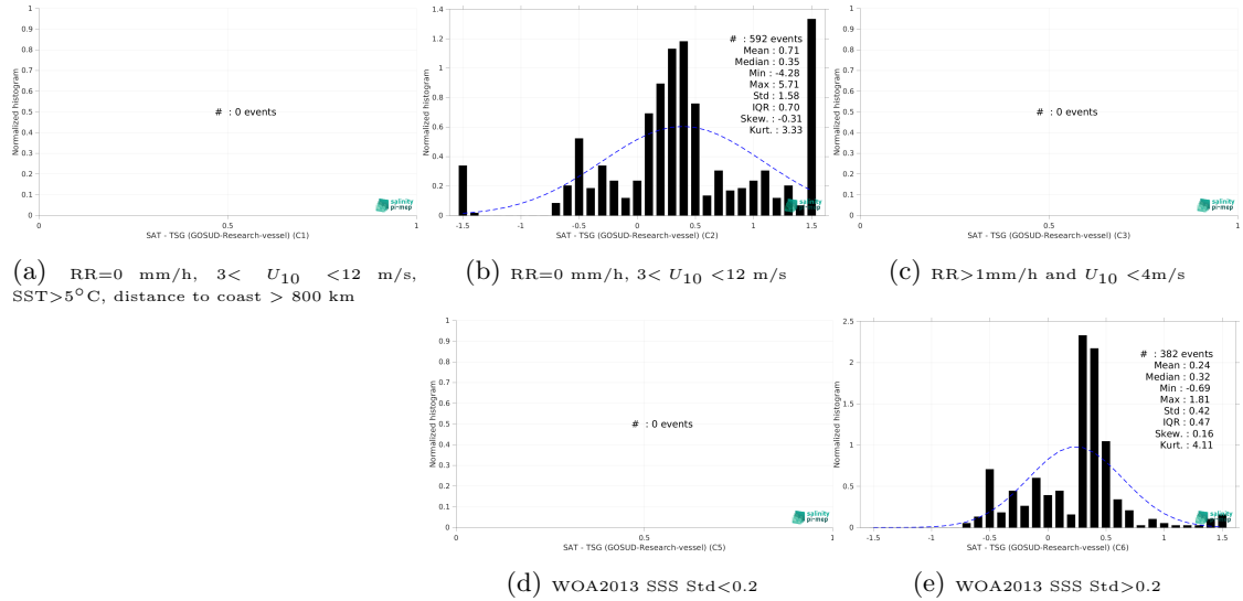
Figure 15: Normalized histogram of \Delta SSS (SMOS SSS L4 v1 - Daily (CMEMS-CNR) - TSG (GOSUD-Research-vessel)) for 5 different subdatasets corresponding to: RR=0 mm/h, 3 < U_{10} < 12 m/s, SST > 5°C, distance to coast > 800 km (a), RR=0 mm/h, 3 < U_{10} < 12 m/s (b), RR > 1mm/h and U_{10} < 4 m/s (c), WOA2013 SSS Std < 0.2 (d), WOA2013 SSS Std > 0.2 (e).
