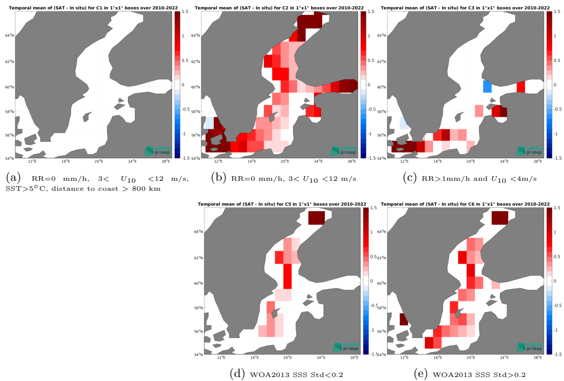
Figure 14: Temporal mean gridded over spatial boxes of size 1^\circ \times 1^\circ of \Delta\text{SSS} (SMOS SSS L4 v1 - Daily (CMEMS-CNR) - ICES) for 5 different subdatasets corresponding to:RR=0 mm/h, 3 < U_{10} < 12 m/s, SST >5^\circ\text{C} , distance to coast > 800 km (a), RR=0 mm/h, 3 < U_{10} < 12 m/s (b), RR >1 mm/h and U_{10} < 4 m/s (c), WOA2013 SSS Std <0.2 (d), WOA2013 SSS Std >0.2 (e).
