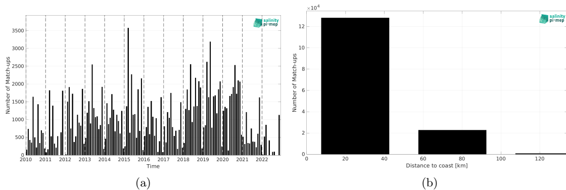
Figure 2: Number of match-ups between ICES and SMOS SSS L4 v1 - Daily (CMEMS-CNR) SSS as a function of time (a) and as function of the distance to coast (b) over the Baltic Sea Pi-MEP region and for the full satellite product period.
