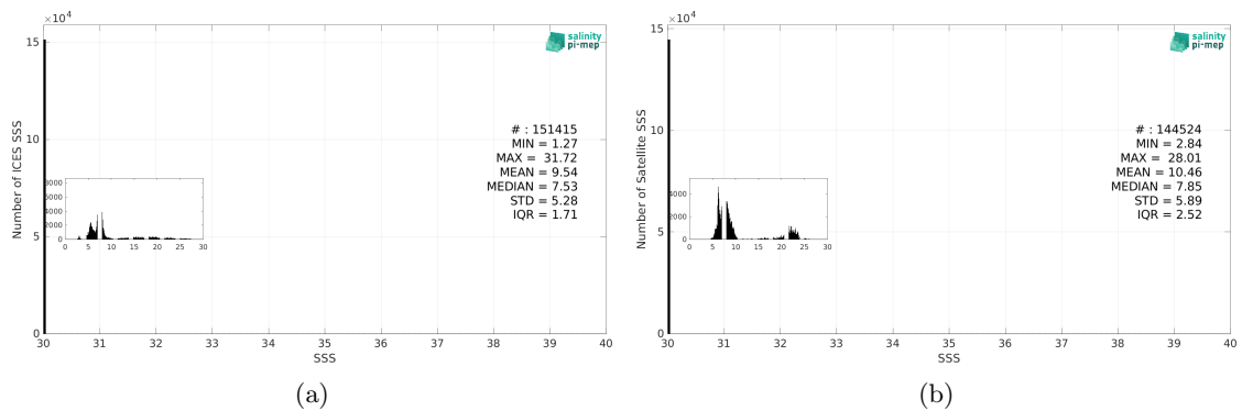
Figure 3: Histograms of SSS from ICES (a) and SMOS SSS L4 v1 - Daily (CMEMS-CNR) (b) considering all match-up pairs per bins of 0.1 over the Baltic Sea Pi-MEP region and for the full satellite product period.
