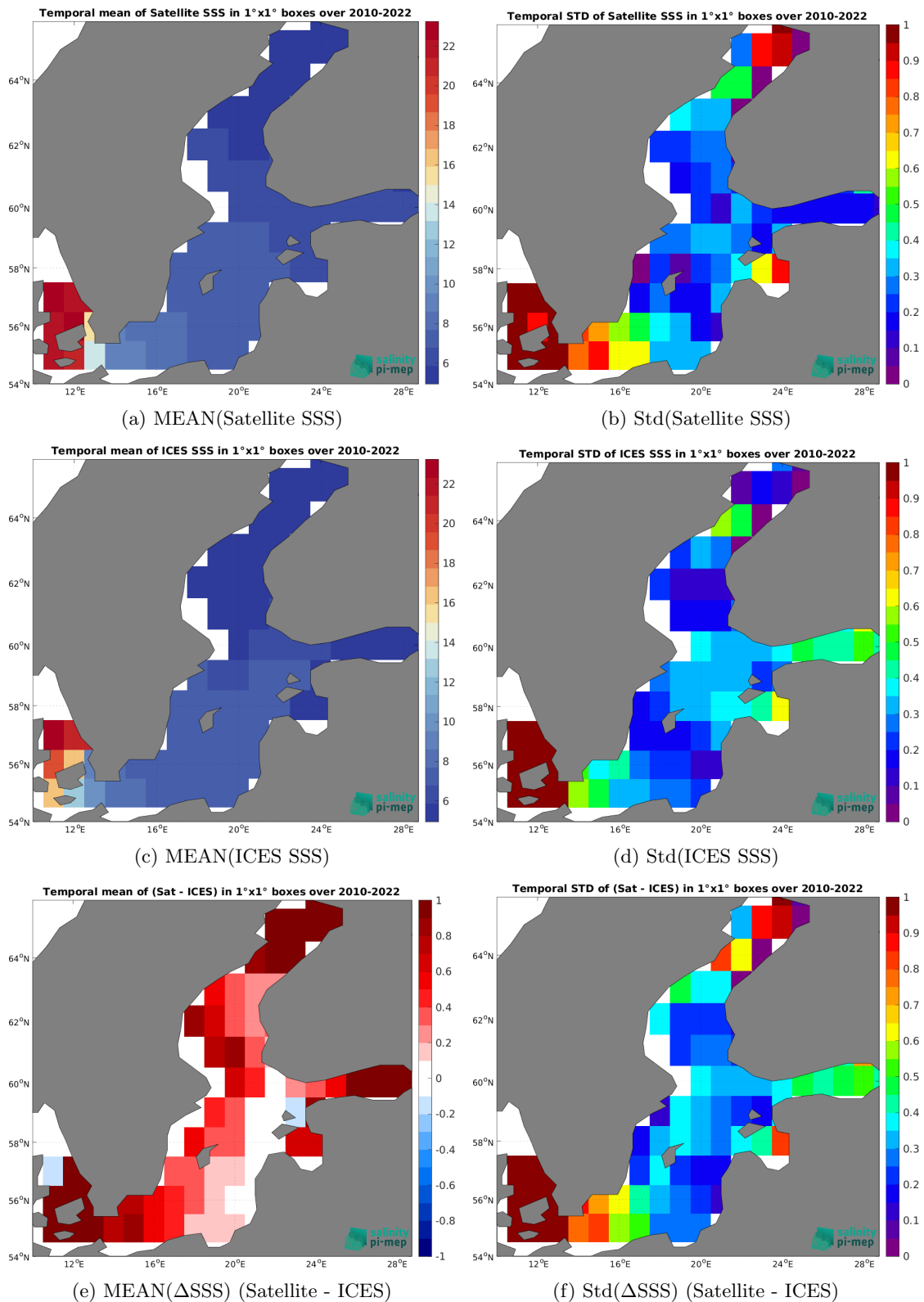
Figure 7: Temporal mean (left) and Std (right) of SSS from SMOS SSS L4 v1 - Daily (CMEMS-CNR) (top), ICES (middle), and of \Delta SSS (Satellite - ICES). Only match-up pairs are used to generate these maps.
