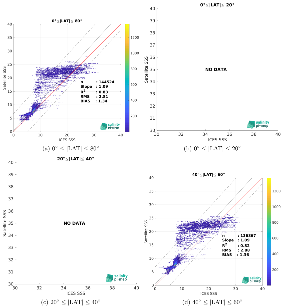
Figure 10: Contour maps of the concentration of SMOS SSS L4 v1 - Daily (CMEMS-CNR) SSS (y-axis) versus ICES SSS (x-axis) at match-up pairs for different latitude bands. For each plot, the red line shows x=y . The black thin and dashed lines indicate a linear fit through the data cloud and the \pm 95\% confidence levels, respectively. The number match-up pairs n , the slope and R^2 coefficient of the linear fit, the root mean square (RMS) and the mean bias between satellite and in situ data are indicated for each latitude band in each plots.
