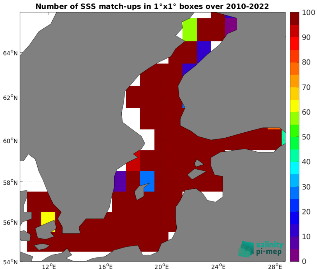
Figure 5: Number of SSS match-ups between ICES SSS and the SMOS SSS L4 v1 - Daily (CMEMS-CNR) SSS product for the Baltic Sea Pi-MEP region over 1°x1° boxes and for the full satellite product period.
