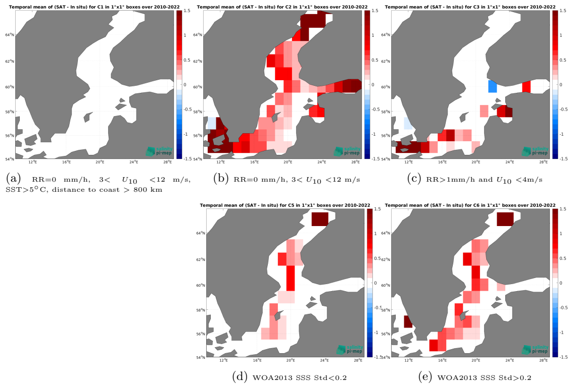
Figure 14: Temporal mean gridded over spatial boxes of size 1^\circ \times 1^\circ of \Delta SSS (SMOS SSS L4 v1 - Daily (CMEMS-CNR) - ICES) for 5 different subdatasets corresponding to:RR=0 mm/h, 3 < U_{10} < 12 m/s, SST >5^\circ\text{C} , distance to coast > 800 km (a), RR=0 mm/h, 3 < U_{10} < 12 m/s (b), RR >1 mm/h and U_{10} < 4 m/s (c), WOA2013 SSS Std <0.2 (d), WOA2013 SSS Std >0.2 (e).
