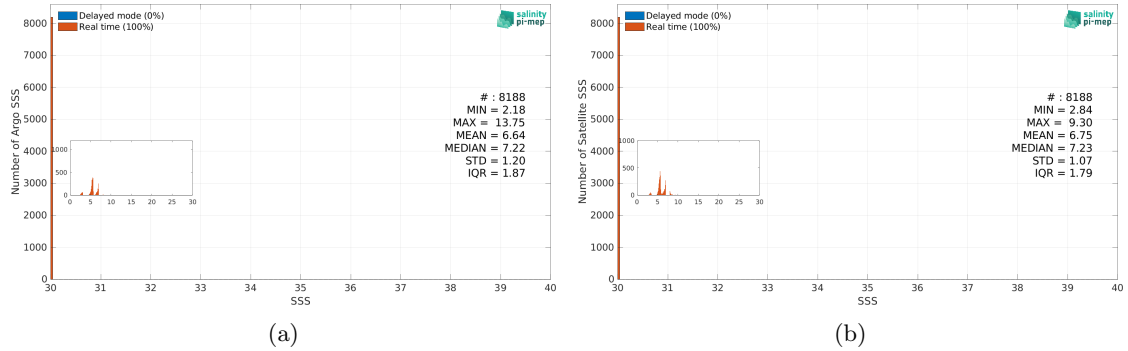
Figure 3: Histograms of SSS from Argo (a) and SMOS SSS L4 v1 - Daily (CMEMS-CNR) (b) considering all match-up pairs per bins of 0.1 over the Baltic Sea Pi-MEP region and for the full satellite product period.
