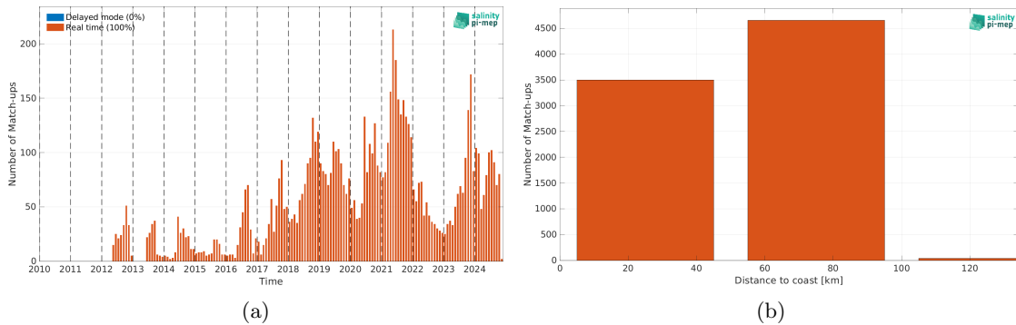
Figure 2: Number of match-ups between Argo and SMOS SSS L4 v1 - Daily (CMEMS-CNR) SSS as a function of time (a) and as function of the distance to coast (b) over the Baltic Sea Pi-MEP region and for the full satellite product period.
