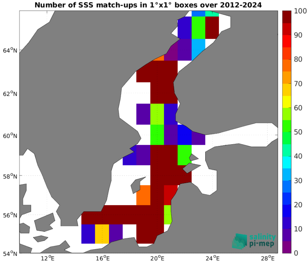
Figure 5: Number of SSS match-ups between Argo SSS and the SMOS SSS L4 v1 - Daily (CMEMS-CNR) SSS product for the Baltic Sea Pi-MEP region over 1^\circ \times 1^\circ boxes and for the full satellite product period.
