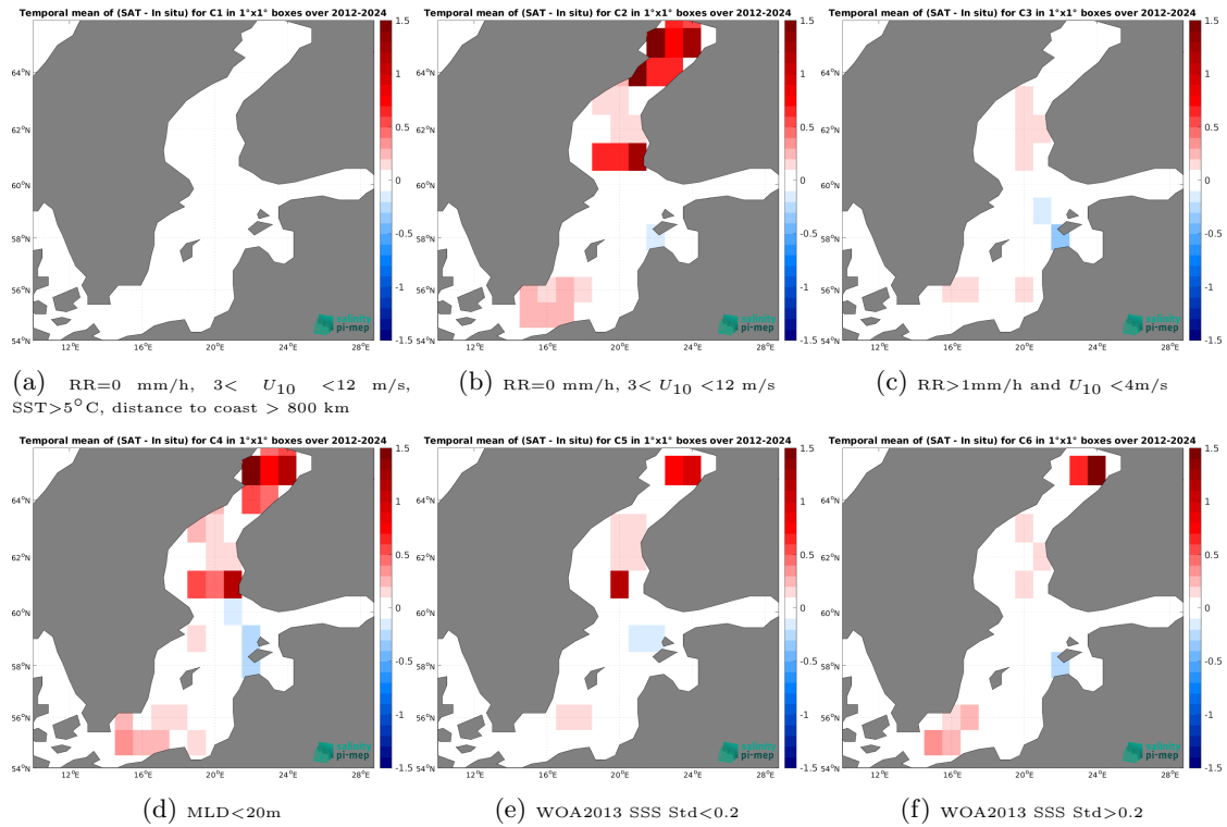
Figure 14: Temporal mean gridded over spatial boxes of size 1^\circ \times 1^\circ of \Delta SSS (SMOS SSS L4 v1 - Daily (CMEMS-CNR) - Argo) for 6 different subdatasets corresponding to:RR=0 mm/h, 3 < U_{10} < 12 m/s, SST>5°C, distance to coast > 800 km (a), RR=0 mm/h, 3 < U_{10} < 12 m/s (b), RR>1mm/h and U_{10} < 4 m/s (c),MLD<20m (d),WOA2013 SSS Std<0.2 (e),WOA2013 SSS Std>0.2 (f).
