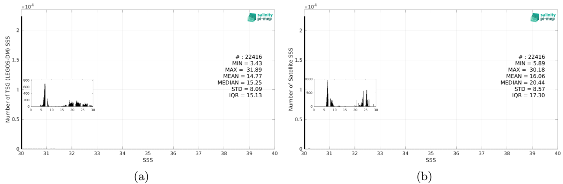
Figure 3: Histograms of SSS from TSG (LEGOS-DM) (a) and SMOS SSS L4 OI v346 - Weekly (CMEMS-CATDS-LOPS) (b) considering all match-up pairs per bins of 0.1 over the Baltic Sea Pi-MEP region and for the full satellite product period.
