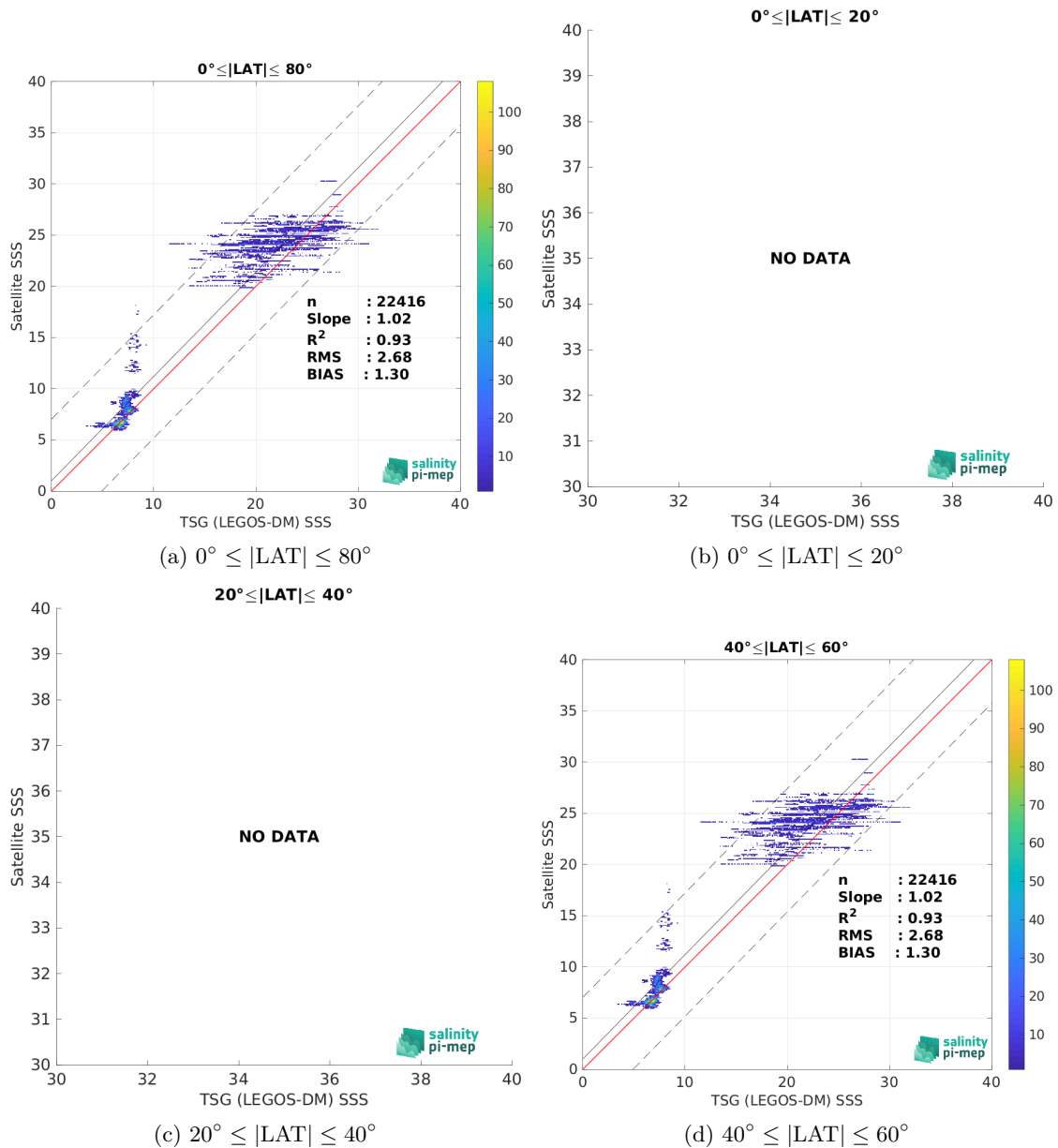
Figure 10: Contour maps of the concentration of SMOS SSS L4 OI v346 - Weekly (CMEMS-CATDS-LOPS) SSS (y-axis) versus TSG (LEGOS-DM) SSS (x-axis) at match-up pairs for different latitude bands. For each plot, the red line shows x=y . The black thin and dashed lines indicate a linear fit through the data cloud and the \pm 95\% confidence levels, respectively. The number match-up pairs n , the slope and R^2 coefficient of the linear fit, the root mean square (RMS) and the mean bias between satellite and in situ data are indicated for each latitude band in each plots.
