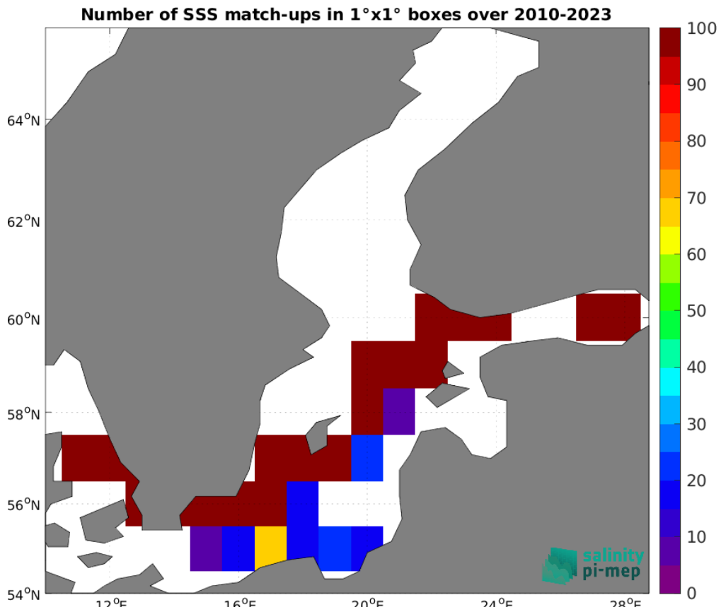
Figure 5: Number of SSS match-ups between TSG (LEGOS-DM) SSS and the SMOS SSS L4 OI v346 - Weekly (CMEMS-CATDS-LOPS) SSS product for the Baltic Sea Pi-MEP region over 1°x1° boxes and for the full satellite product period.
