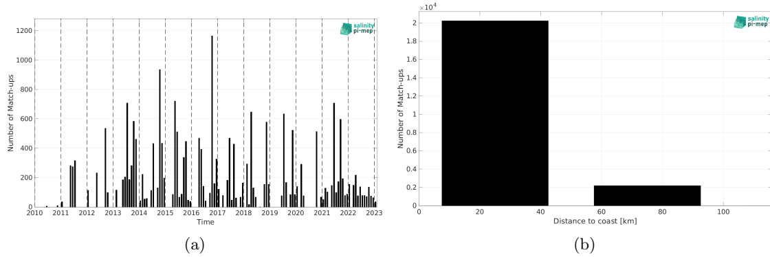
Figure 2: Number of match-ups between TSG (LEGOS-DM) and SMOS SSS L4 OI v346 - Weekly (CMEMS-CATDS-LOPS) SSS as a function of time (a) and as function of the distance to coast (b) over the Baltic Sea Pi-MEP region and for the full satellite product period.
