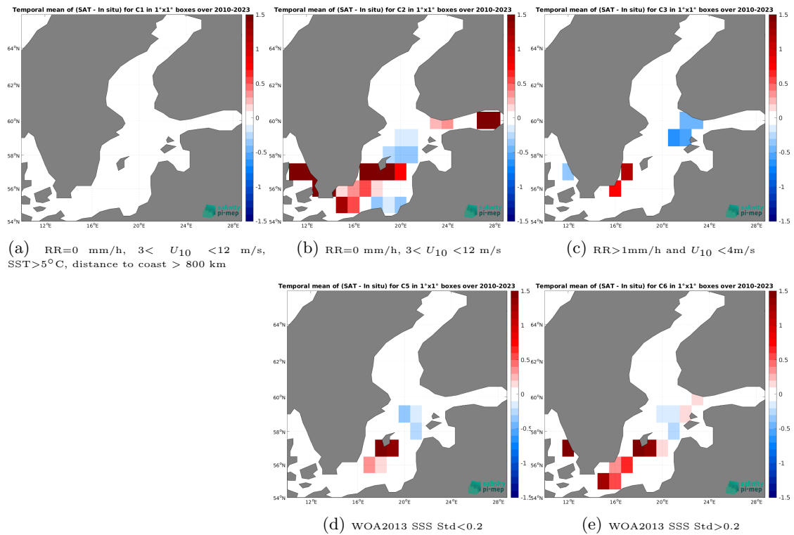
Figure 14: Temporal mean gridded over spatial boxes of size 1^\circ \times 1^\circ of \Delta SSS (SMOS SSS L4 OI v346 - Weekly (CMEMS-CATDS-LOPS) - TSG (LEGOS-DM)) for 5 different subdatasets corresponding to:RR=0 mm/h, 3 < U_{10} < 12 m/s, SST>5°C, distance to coast > 800 km (a), RR=0 mm/h, 3 < U_{10} < 12 m/s (b), RR>1mm/h and U_{10} < 4 m/s (c), WOA2013 SSS Std<0.2 (d), WOA2013 SSS Std>0.2 (e).
