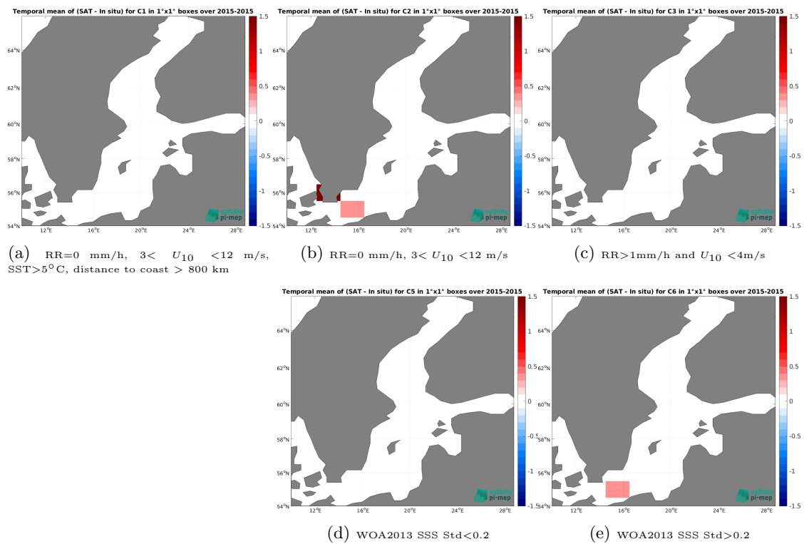
Figure 14: Temporal mean gridded over spatial boxes of size 1^\circ \times 1^\circ of \Delta SSS (SMOS SSS L4 OI v346 - Weekly (CMEMS-CATDS-LOPS) - TSG (GOSUD-Research-vessel)) for 5 different subdatasets corresponding to:RR=0 mm/h, 3 < U_{10} < 12 m/s, SST >5^\circ\text{C} , distance to coast > 800 km (a), RR=0 mm/h, 3 < U_{10} < 12 m/s (b), RR >1 mm/h and U_{10} < 4 m/s (c), WOA2013 SSS Std <0.2 (d), WOA2013 SSS Std >0.2 (e).
