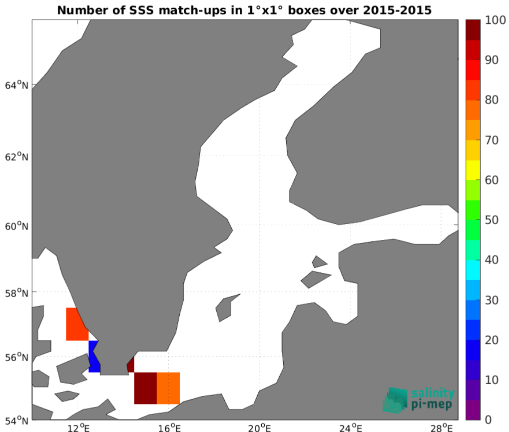
Figure 5: Number of SSS match-ups between TSG (GOSUD-Research-vessel) SSS and the SMOS SSS L4 OI v346 - Weekly (CMEMS-CATDS-LOPS) SSS product for the Baltic Sea Pi-MEP region over 1°x1° boxes and for the full satellite product period.
