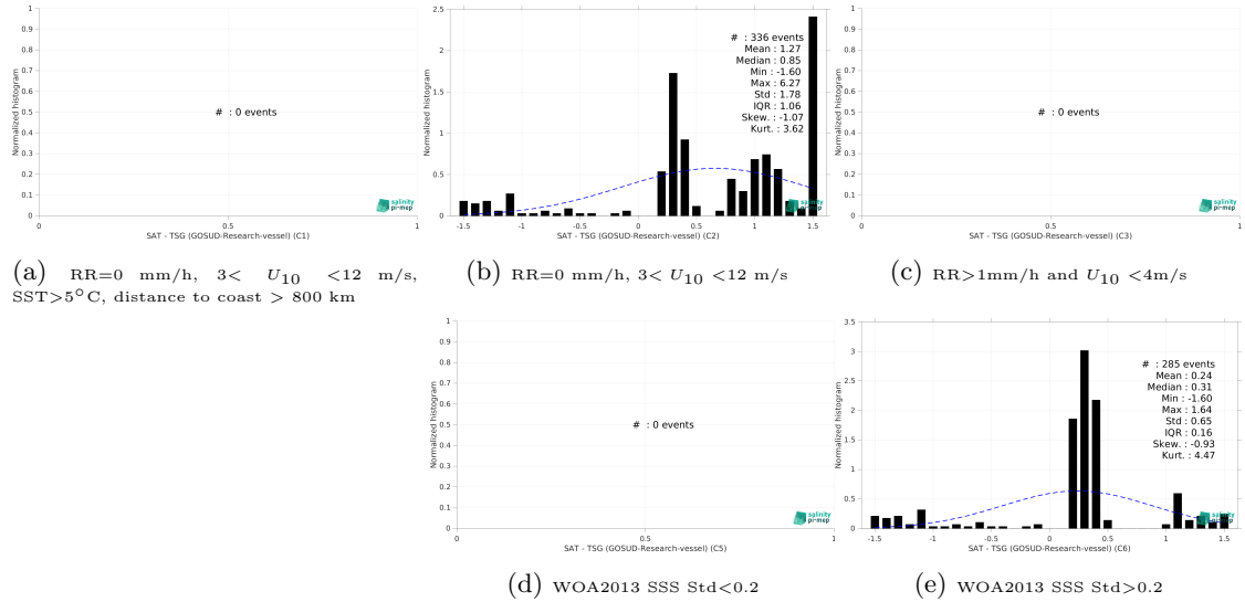
Figure 15: Normalized histogram of \Delta SSS (SMOS SSS L4 OI v346 - Weekly (CMEMS-CATDS-LOPS) - TSG (GOSUD-Research-vessel)) for 5 different subdatasets corresponding to: RR=0 mm/h, 3 < U_{10} < 12 m/s, SST>5°C, distance to coast > 800 km (a), RR=0 mm/h, 3 < U_{10} < 12 m/s (b), RR>1mm/h and U_{10} < 4 m/s (c), WOA2013 SSS Std<0.2 (d), WOA2013 SSS Std>0.2 (e).
