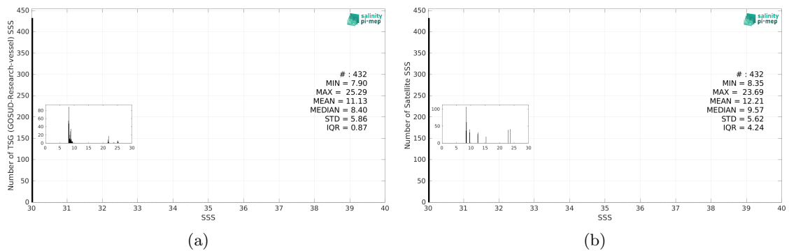
Figure 3: Histograms of SSS from TSG (GOSUD-Research-vessel) (a) and SMOS SSS L4 OI v346 - Weekly (CMEMS-CATDS-LOPS) (b) considering all match-up pairs per bins of 0.1 over the Baltic Sea Pi-MEP region and for the full satellite product period.
