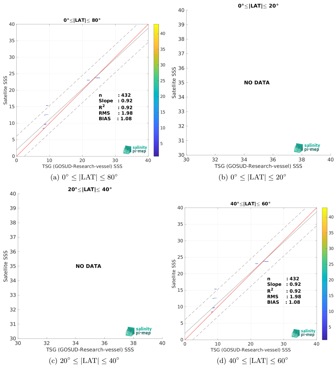
Figure 10: Contour maps of the concentration of SMOS SSS L4 OI v346 - Weekly (CMEMS-CATDS-LOPS) SSS (y-axis) versus TSG (GOSUD-Research-vessel) SSS (x-axis) at match-up pairs for different latitude bands. For each plot, the red line shows x=y . The black thin and dashed lines indicate a linear fit through the data cloud and the \pm 95\% confidence levels, respectively. The number match-up pairs n , the slope and R^2 coefficient of the linear fit, the root mean square (RMS) and the mean bias between satellite and in situ data are indicated for each latitude band in each plots.
