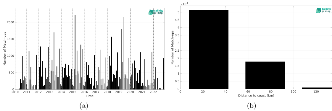
Figure 2: Number of match-ups between ICES and SMOS SSS L4 OI v346 - Weekly (CMEMS-CATDS-LOPS) SSS as a function of time (a) and as function of the distance to coast (b) over the Baltic Sea Pi-MEP region and for the full satellite product period.
