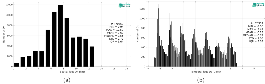
Figure 6: Histograms of the spatial (a) and temporal (b) lags between the location/time of the ICES measurement and the date of the corresponding SMOS SSS L4 OI v346 - Weekly (CMEMS-CATDS-LOPS) SSS pixel.
