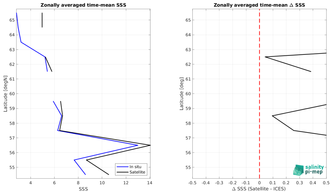
Figure 9: Left panel: Zonal mean SSS from SMOS SSS L4 OI v346 - Weekly (CMEMS-CATDS-LOPS) satellite product (black) and from ICES (blue). Right panel: Zonal mean of \Delta SSS (Satellite - ICES) for all the collected Pi-MEP match-up pairs estimated over the full satellite product period.
