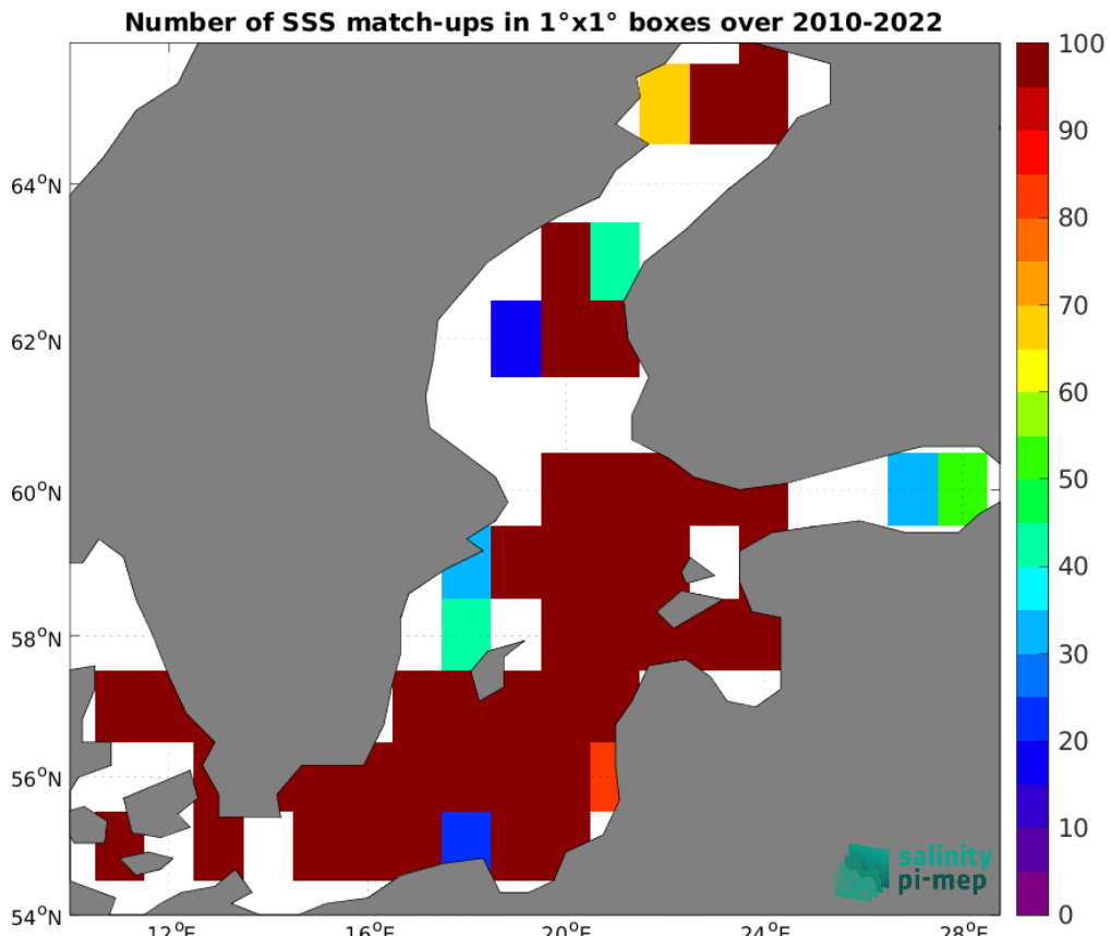
Figure 5: Number of SSS match-ups between ICES SSS and the SMOS SSS L4 OI v346 - Weekly (CMEMS-CATDS-LOPS) SSS product for the Baltic Sea Pi-MEP region over 1°x1° boxes and for the full satellite product period.
