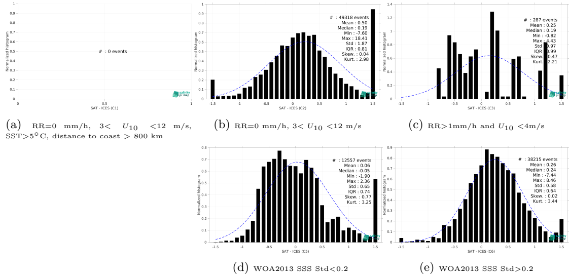
Figure 15: Normalized histogram of \Delta SSS (SMOS SSS L4 OI v346 - Weekly (CMEMS-CATDS-LOPS) - ICES) for 5 different subdatasets corresponding to: RR=0 mm/h, 3 < U_{10} < 12 m/s, SST>5°C, distance to coast > 800 km (a), RR=0 mm/h, 3 < U_{10} < 12 m/s (b), RR>1mm/h and U_{10} < 4 m/s (c), WOA2013 SSS Std<0.2 (d), WOA2013 SSS Std>0.2 (e).
