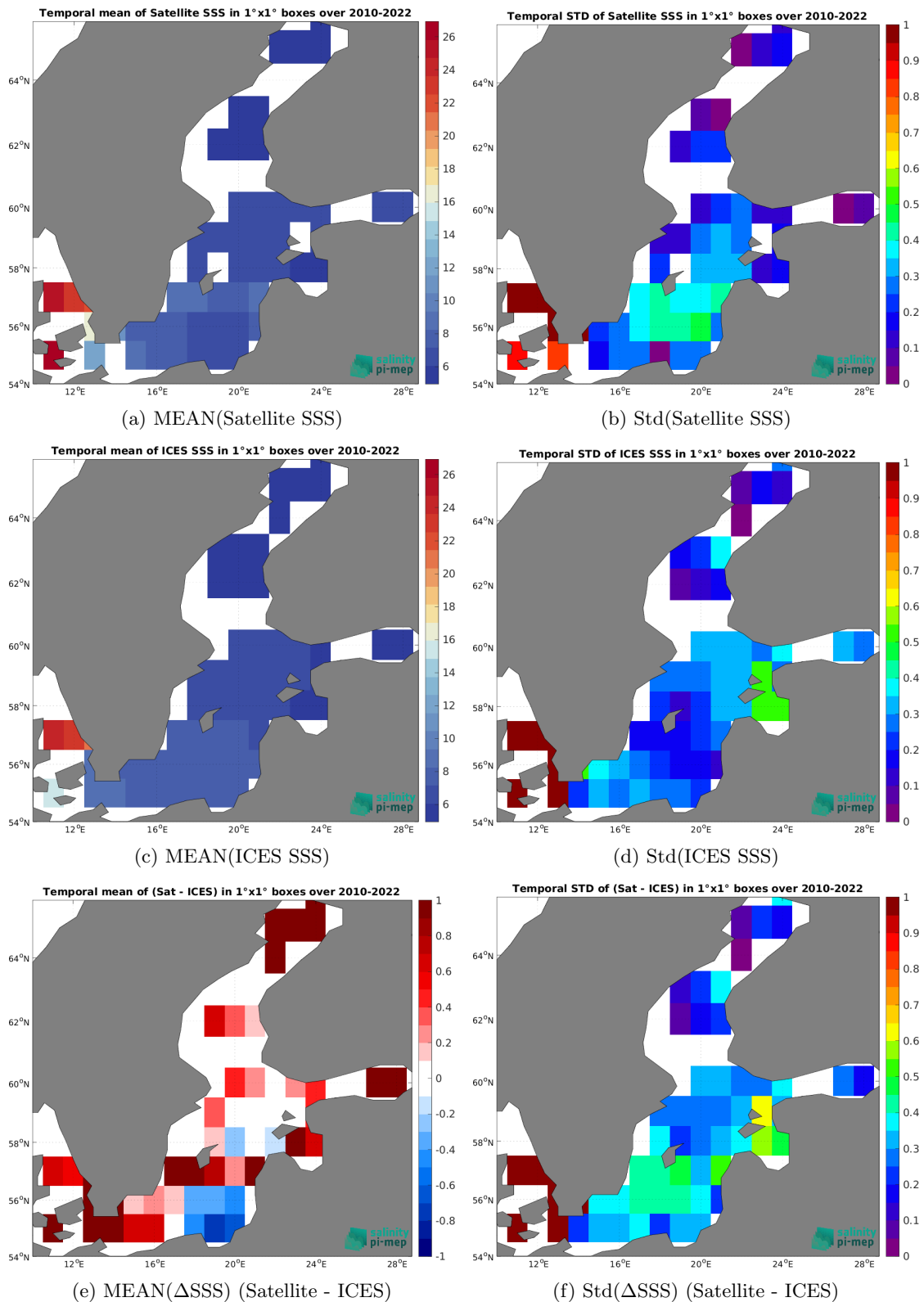
Figure 7: Temporal mean (left) and Std (right) of SSS from SMOS SSS L4 OI v346 - Weekly (CMEMS-CATDS-LOPS) (top), ICES (middle), and of \Delta SSS (Satellite - ICES). Only match-up pairs are used to generate these maps.
