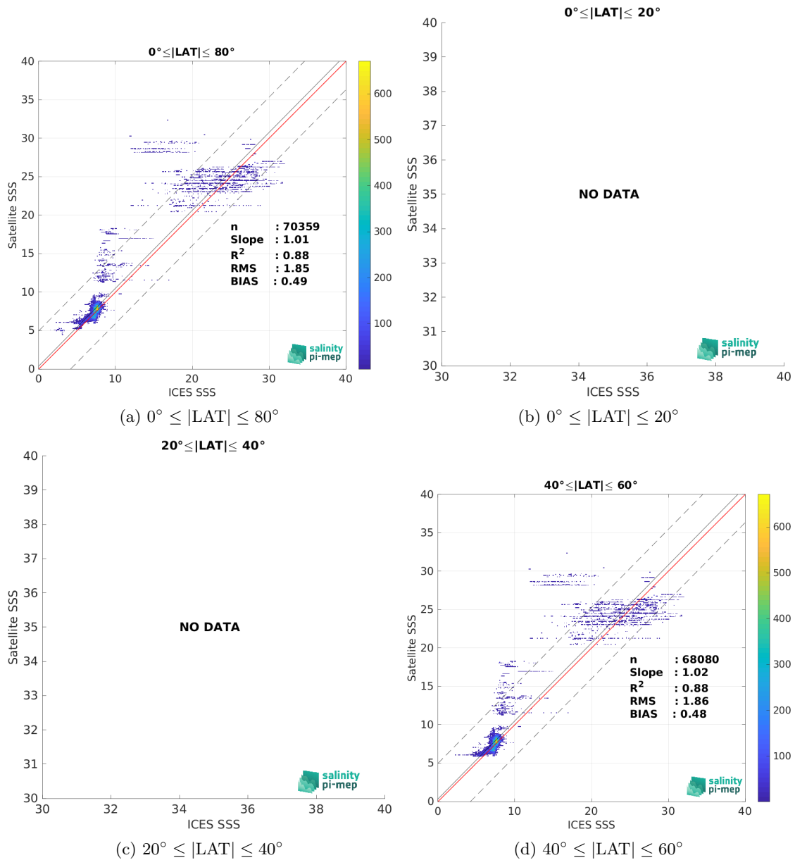
Figure 10: Contour maps of the concentration of SMOS SSS L4 OI v346 - Weekly (CMEMS-CATDS-LOPS) SSS (y-axis) versus ICES SSS (x-axis) at match-up pairs for different latitude bands. For each plot, the red line shows x=y . The black thin and dashed lines indicate a linear fit through the data cloud and the \pm 95\% confidence levels, respectively. The number match-up pairs n , the slope and R^2 coefficient of the linear fit, the root mean square (RMS) and the mean bias between satellite and in situ data are indicated for each latitude band in each plots.
