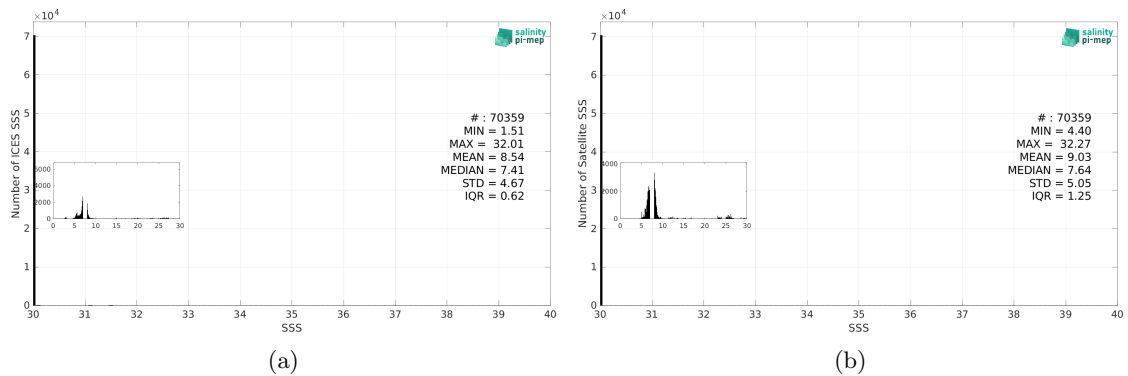
Figure 3: Histograms of SSS from ICES (a) and SMOS SSS L4 OI v346 - Weekly (CMEMS-CATDS-LOPS) (b) considering all match-up pairs per bins of 0.1 over the Baltic Sea Pi-MEP region and for the full satellite product period.
