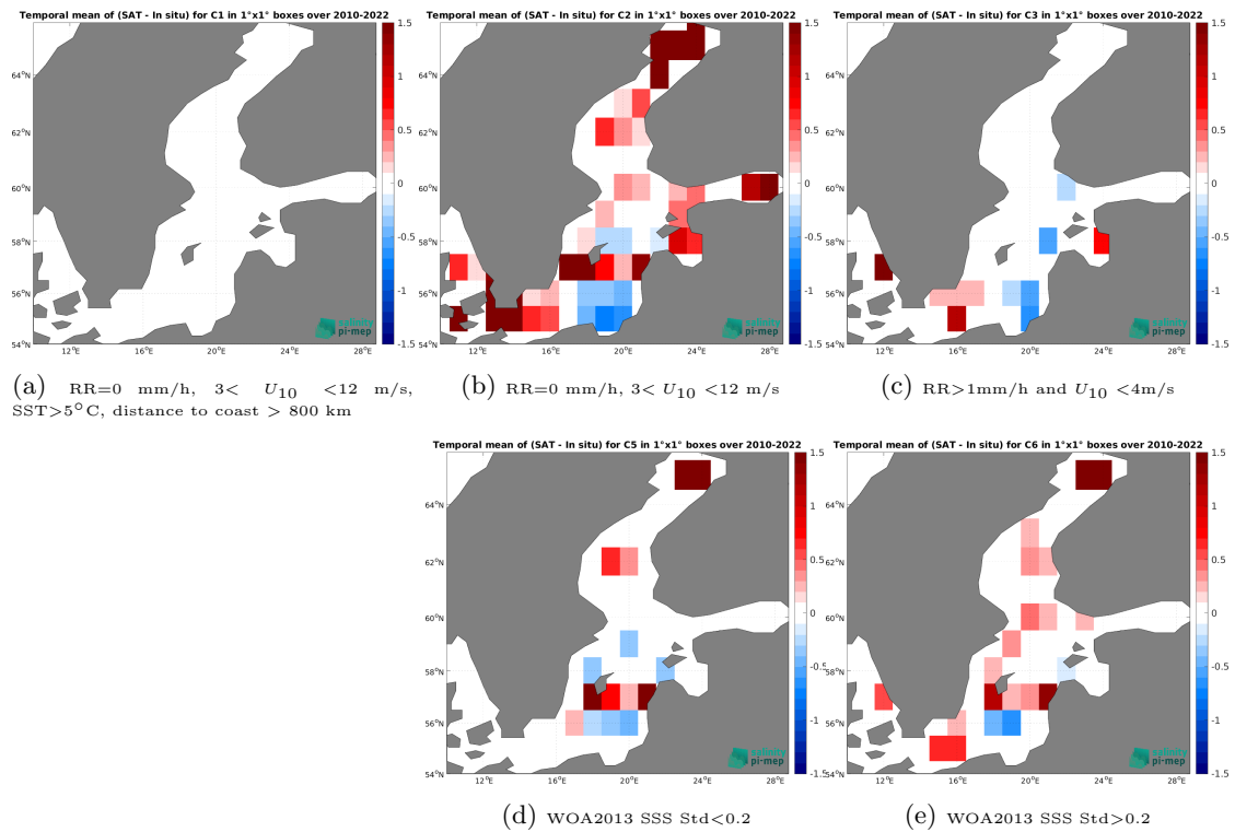
Figure 14: Temporal mean gridded over spatial boxes of size 1^\circ \times 1^\circ of \Delta\text{SSS} (SMOS SSS L4 OI v346 - Weekly (CMEMS-CATDS-LOPS) - ICES) for 5 different subdatasets corresponding to:RR=0 mm/h, 3 < U_{10} < 12 m/s, SST >5^\circ\text{C} , distance to coast > 800 km (a), RR=0 mm/h, 3 < U_{10} < 12 m/s (b), RR >1 mm/h and U_{10} < 4 m/s (c), WOA2013 SSS Std <0.2 (d), WOA2013 SSS Std >0.2 (e).
