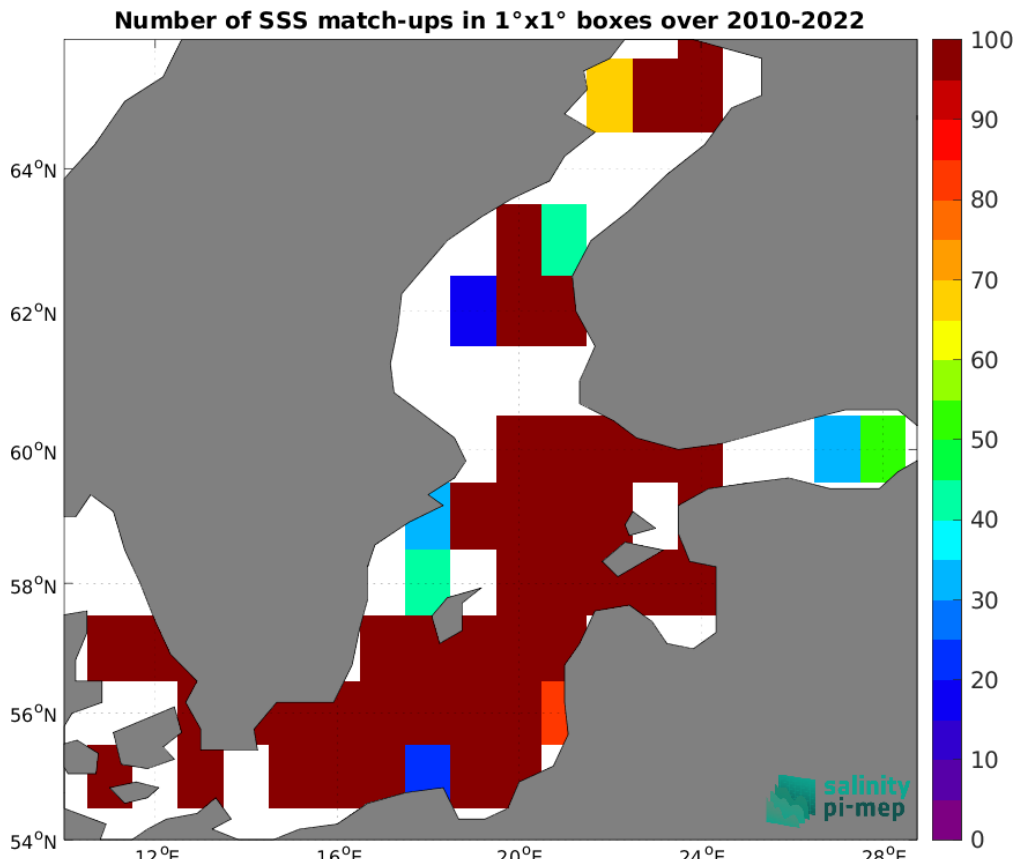
Figure 5: Number of SSS match-ups between ICES SSS and the SMOS SSS L4 OI v346 - Weekly (CMEMS-CATDS-LOPS) SSS product for the Baltic Sea Pi-MEP region over 1°×1° boxes and for the full satellite product period.
