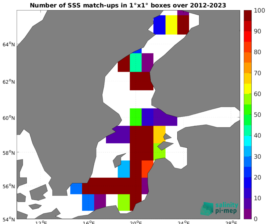
Figure 5: Number of SSS match-ups between Argo SSS and the SMOS SSS L4 OI v346 - Weekly (CMEMS-CATDS-LOPS) SSS product for the Baltic Sea Pi-MEP region over 1°x1° boxes and for the full satellite product period.
