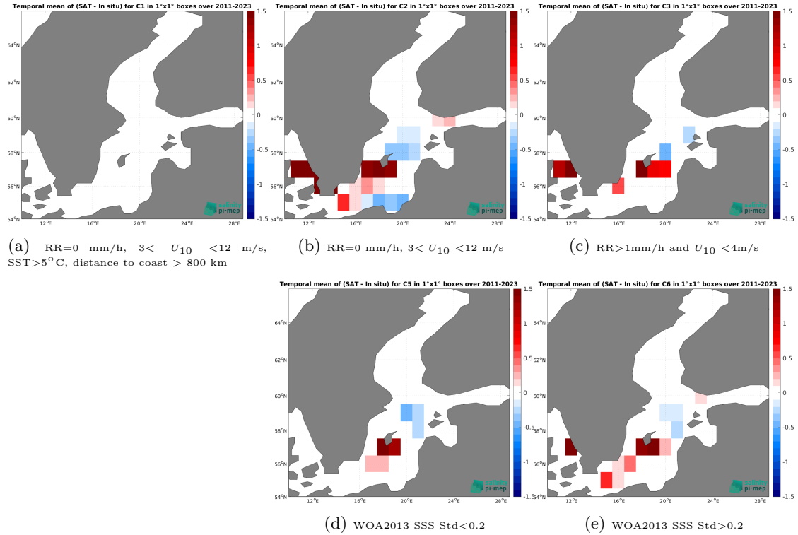
Figure 12: Temporal mean gridded over spatial boxes of size 1^{\circ}\times 1^{\circ} of \Delta\text{SSS} (SMOS SSS L4 OI v342 - Weekly (CMEMS-CATDS-LOPS) - TSG (LEGOS-DM)) for 5 different subdatasets corresponding to:RR=0 mm/h, 3 < U_{10} < 12 m/s, SST >5^{\circ}\text{C} , distance to coast > 800 km (a), RR=0 mm/h, 3 < U_{10} < 12 m/s (b), RR >1\text{mm/h} and U_{10} < 4\text{m/s} (c), WOA2013 SSS Std <0.2 (d), WOA2013 SSS Std >0.2 (e).
