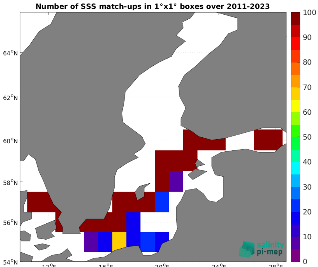
Figure 4: Number of SSS match-ups between TSG (LEGOS-DM) SSS and the SMOS SSS L4 OI v342 - Weekly (CMEMS-CATDS-LOPS) SSS product for the Baltic Sea Pi-MEP region over 1°x1° boxes and for the full satellite product period.
