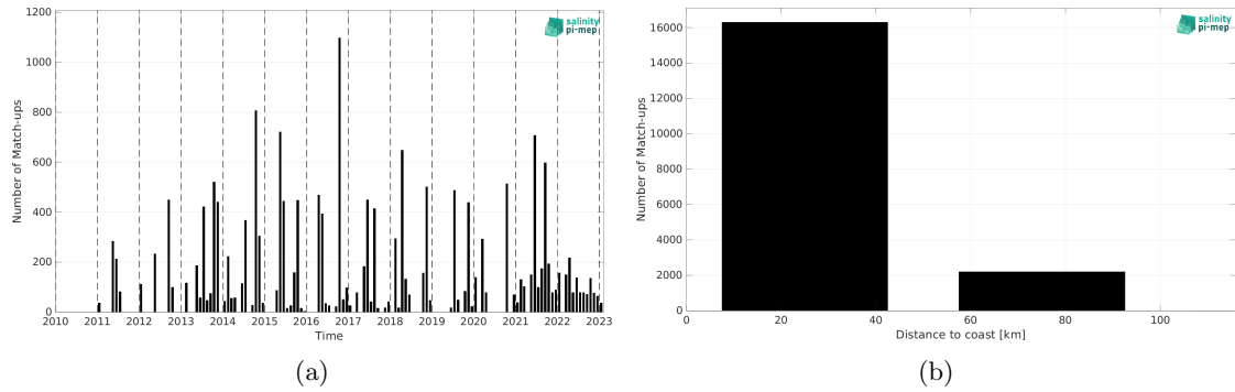
Figure 1: Number of match-ups between TSG (LEGOS-DM) and SMOS SSS L4 OI v342 - Weekly (CMEMS-CATDS-LOPS) SSS as a function of time (a) and as function of the distance to coast (b) over the Baltic Sea Pi-MEP region and for the full satellite product period.
