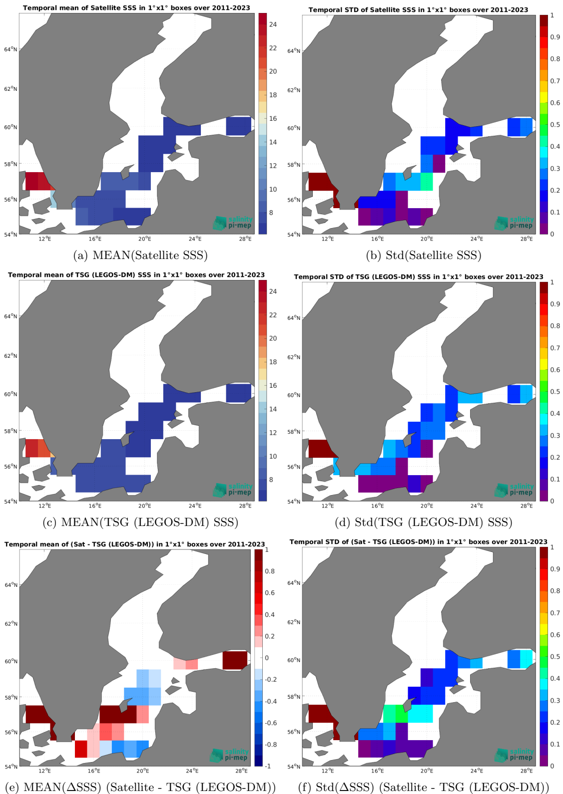
Figure 6: Temporal mean (left) and Std (right) of SSS from SMOS SSS L4 OI v342 - Weekly (CMEMS-CATDS-LOPS) (top), TSG (LEGOS-DM) (middle), and of \Delta SSS (Satellite - TSG (LEGOS-DM)). Only match-up pairs are used to generate these maps.
