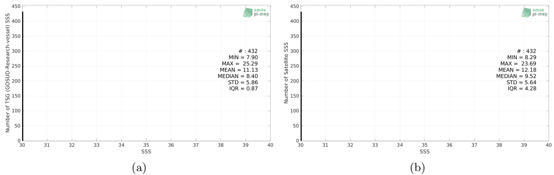
Figure 2: Histograms of SSS from TSG (GOSUD-Research-vessel) (a) and SMOS SSS L4 OI v342 - Weekly (CMEMS-CATDS-LOPS) (b) considering all match-up pairs per bins of 0.1 over the Baltic Sea Pi-MEP region and for the full satellite product period.
