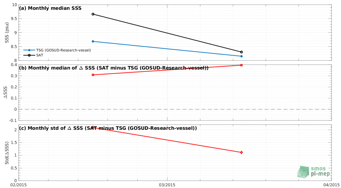
Figure 7: Time series of the monthly median SSS (top), median of \Delta SSS (Satellite - TSG (GOSUD-Research-vessel)) and Std of \Delta SSS (Satellite - TSG (GOSUD-Research-vessel)) over the Baltic Sea Pi-MEP region considering all match-ups collected by the Pi-MEP.
