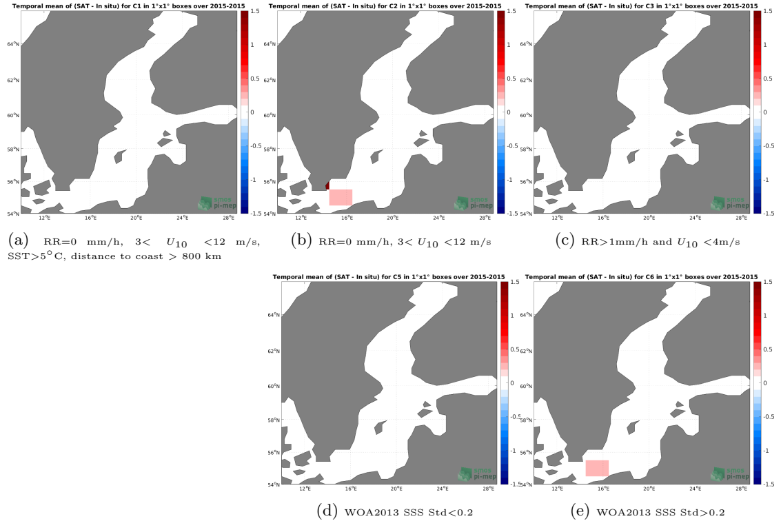
Figure 12: Temporal mean gridded over spatial boxes of size 1^\circ \times 1^\circ of \Delta SSS (SMOS SSS L4 OI v342 - Weekly (CMEMS-CATDS-LOPS) - TSG (GOSUD-Research-vessel)) for 5 different subdatasets corresponding to: RR=0 mm/h, 3 < U_{10} < 12 m/s, SST > 5^\circ\text{C} , distance to coast > 800 km (a), RR=0 mm/h, 3 < U_{10} < 12 m/s (b), RR > 1 mm/h and U_{10} < 4 m/s (c), WOA2013 SSS Std < 0.2 (d), WOA2013 SSS Std > 0.2 (e).
