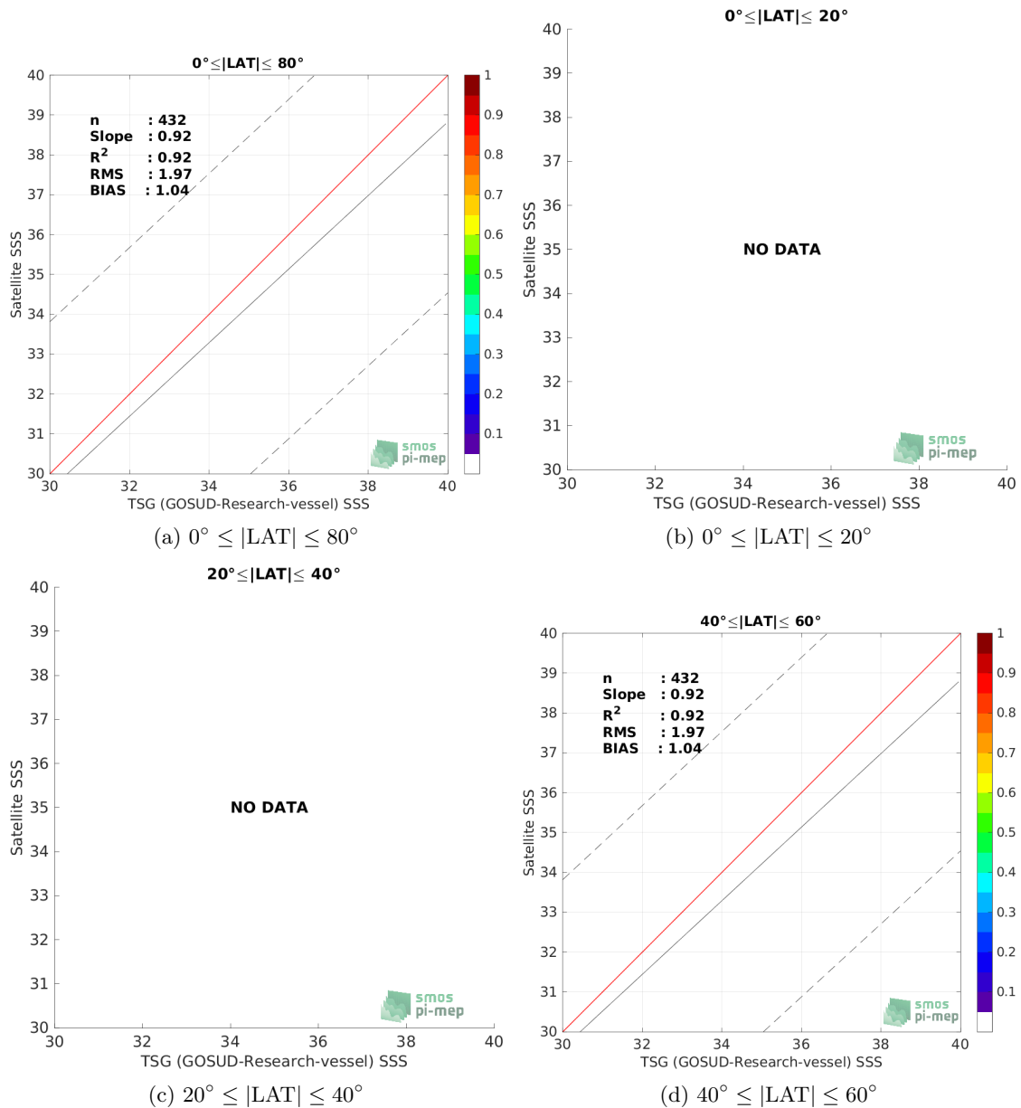
Figure 9: Contour maps of the concentration of SMOS SSS L4 OI v342 - Weekly (CMEMS-CATDS-LOPS) SSS (y-axis) versus TSG (GOSUD-Research-vessel) SSS (x-axis) at match-up pairs for different latitude bands. For each plot, the red line shows x=y . The black thin and dashed lines indicate a linear fit through the data cloud and the \pm 95\% confidence levels, respectively. The number match-up pairs n , the slope and R^2 coefficient of the linear fit, the root mean square (RMS) and the mean bias between satellite and in situ data are indicated for each latitude band in each plots.
