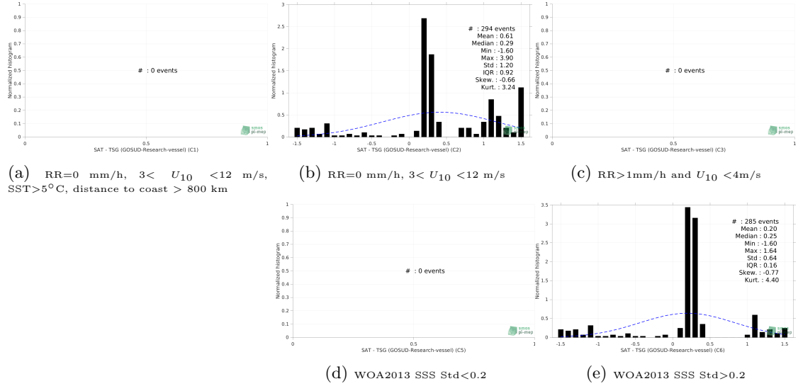
Figure 13: Normalized histogram of \Delta SSS (SMOS SSS L4 OI v342 - Weekly (CMEMS-CATDS-LOPS) - TSG (GOSUD-Research-vessel)) for 5 different subdatasets corresponding to: RR=0 mm/h, 3 < U_{10} < 12 m/s, SST>5°C, distance to coast > 800 km (a), RR=0 mm/h, 3 < U_{10} < 12 m/s (b), RR>1mm/h and U_{10} < 4 m/s (c), WOA2013 SSS Std<0.2 (d), WOA2013 SSS Std>0.2 (e).
