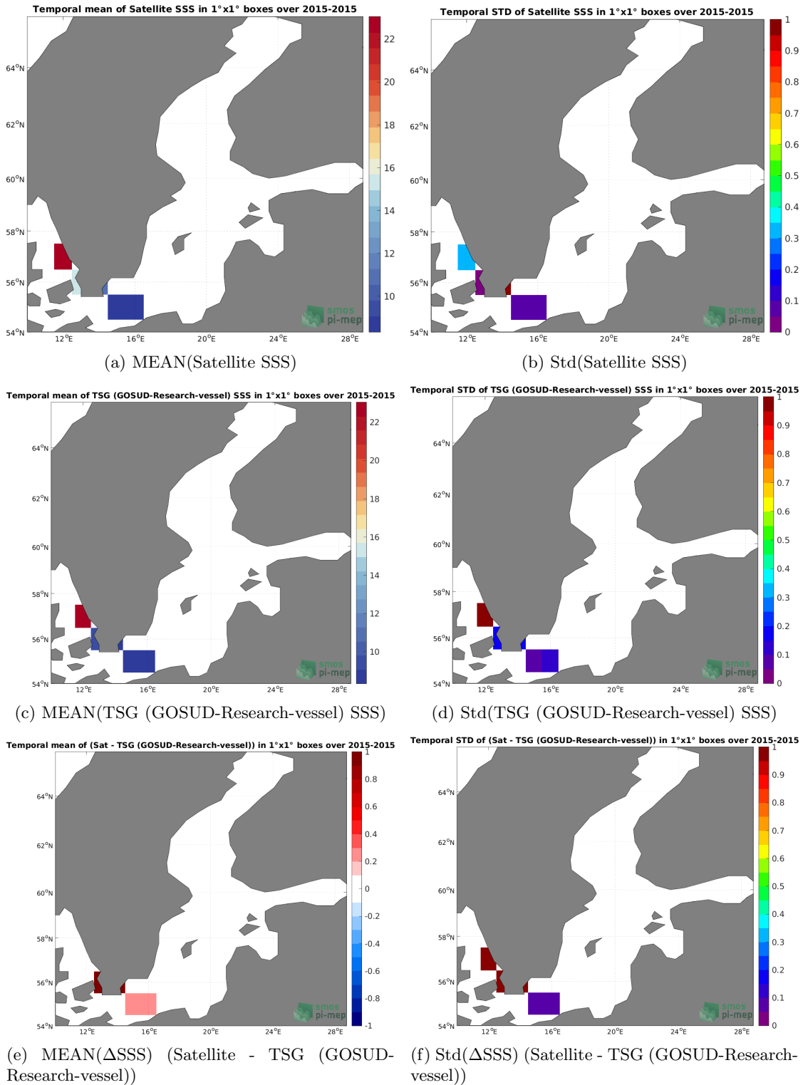
Figure 6: Temporal mean (left) and Std (right) of SSS from SMOS SSS L4 OI v342 - Weekly (CMEMS-CATDS-LOPS) (top), TSG (GOSUD-Research-vessel) (middle), and of \Delta SSS (Satellite - TSG (GOSUD-Research-vessel)). Only match-up pairs are used to generate these maps.
