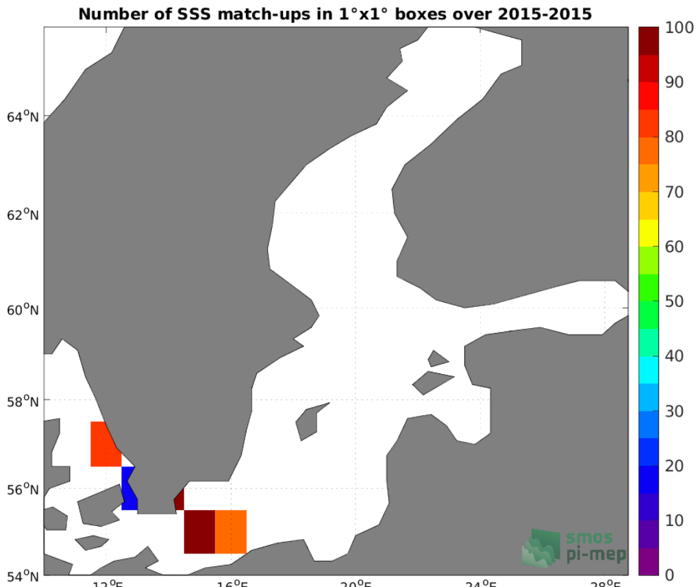
Figure 4: Number of SSS match-ups between TSG (GOSUD-Research-vessel) SSS and the SMOS SSS L4 OI v342 - Weekly (CMEMS-CATDS-LOPS) SSS product for the Baltic Sea Pi-MEP region over 1°x1° boxes and for the full satellite product period.
