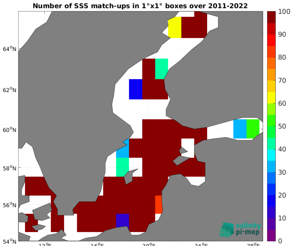
Figure 4: Number of SSS match-ups between ICES SSS and the SMOS SSS L4 OI v342 - Weekly (CMEMS-CATDS-LOPS) SSS product for the Baltic Sea Pi-MEP region over 1°×1° boxes and for the full satellite product period.
