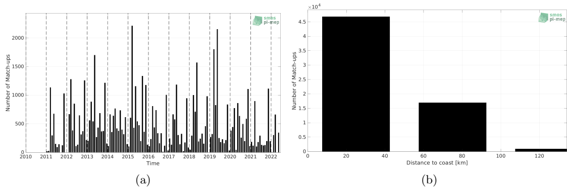
Figure 1: Number of match-ups between ICES and SMOS SSS L4 OI v342 - Weekly (CMEMS-CATDS-LOPS) SSS as a function of time (a) and as function of the distance to coast (b) over the Baltic Sea Pi-MEP region and for the full satellite product period.
