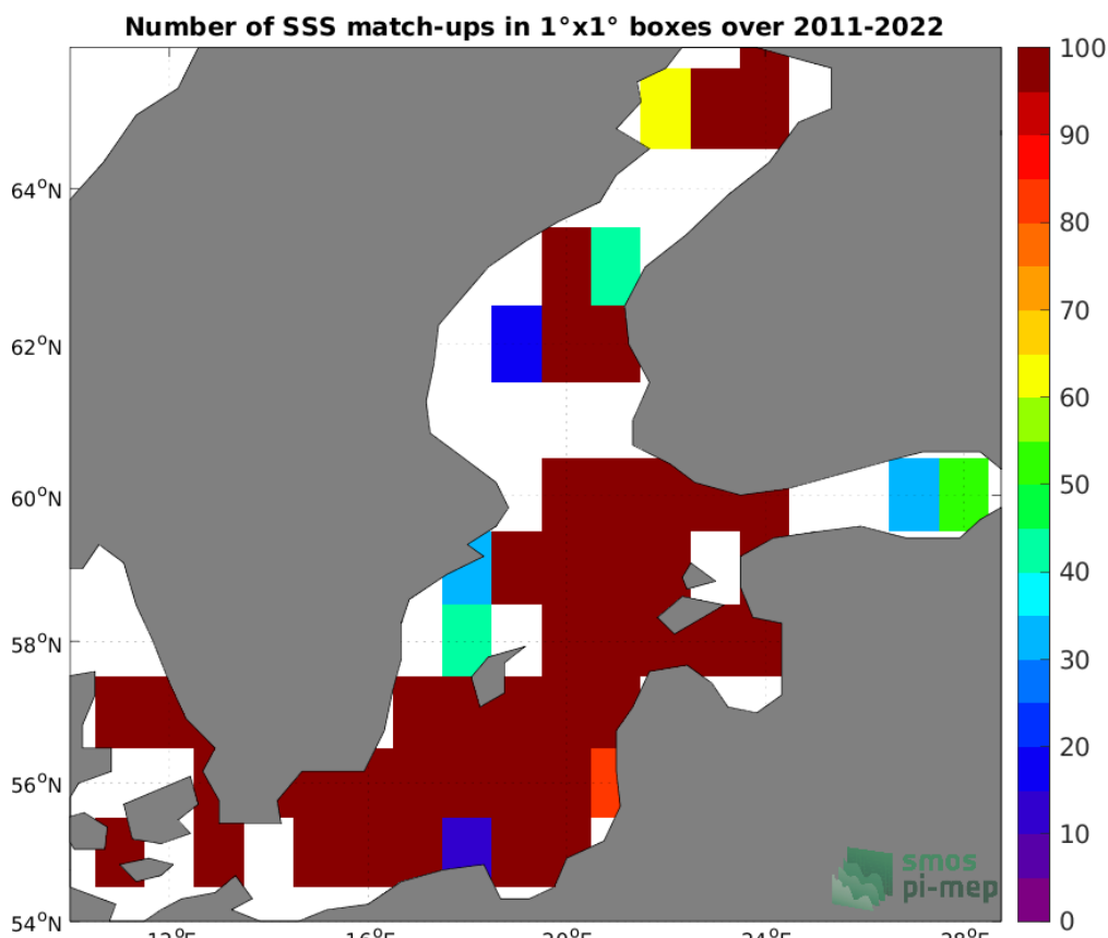
Figure 4: Number of SSS match-ups between ICES SSS and the SMOS SSS L4 OI v342 - Weekly (CMEMS-CATDS-LOPS) SSS product for the Baltic Sea Pi-MEP region over 1°x1° boxes and for the full satellite product period.
