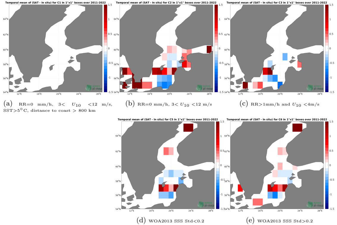
Figure 12: Temporal mean gridded over spatial boxes of size 1^{\circ}\times 1^{\circ} of \Delta\text{SSS} (SMOS SSS L4 OI v342 - Weekly (CMEMS-CATDS-LOPS) - ICES) for 5 different subdatasets corresponding to:RR=0 mm/h, 3 < U_{10} < 12 m/s, SST >5^{\circ}\text{C} , distance to coast > 800 km (a), RR=0 mm/h, 3 < U_{10} < 12 m/s (b), RR >1 mm/h and U_{10} < 4 m/s (c), WOA2013 SSS Std <0.2 (d), WOA2013 SSS Std >0.2 (e).
