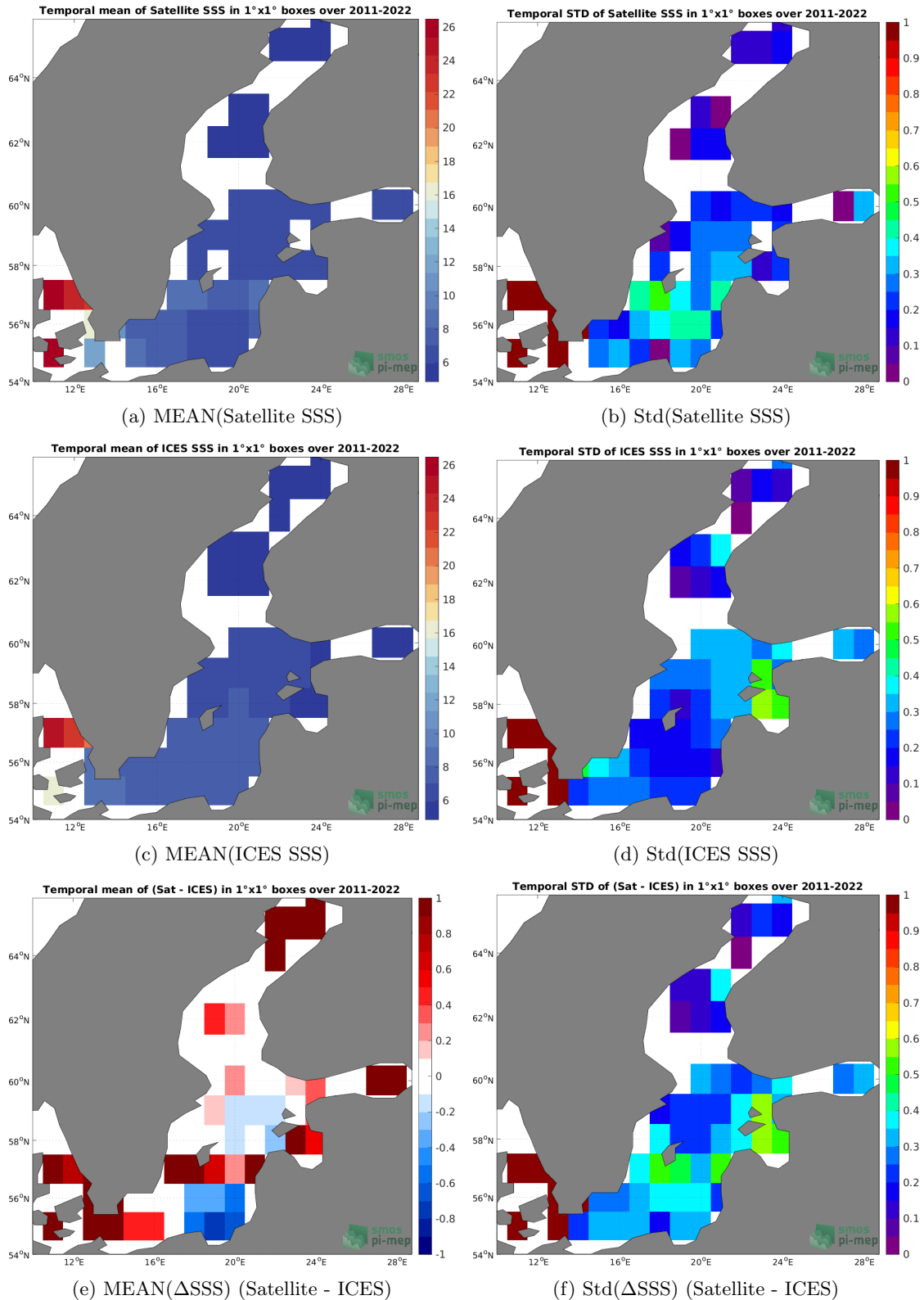
Figure 6: Temporal mean (left) and Std (right) of SSS from SMOS SSS L4 OI v342 - Weekly (CMEMS-CATDS-LOPS) (top), ICES (middle), and of \Delta SSS (Satellite - ICES). Only match-up pairs are used to generate these maps.
