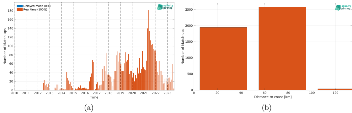
Figure 1: Number of match-ups between Argo and SMOS SSS L4 OI v342 - Weekly (CMEMS-CATDS-LOPS) SSS as a function of time (a) and as function of the distance to coast (b) over the Baltic Sea Pi-MEP region and for the full satellite product period.
