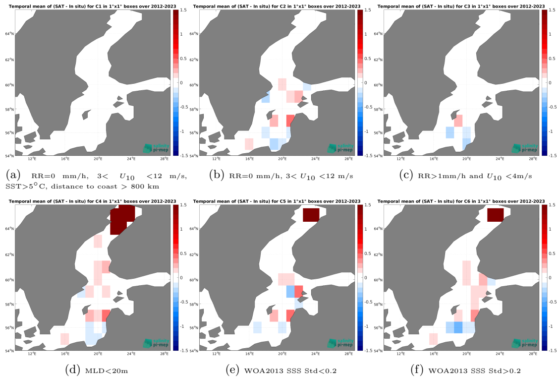
Figure 12: Temporal mean gridded over spatial boxes of size 1^{\circ}\times 1^{\circ} of \Delta\text{SSS} (SMOS SSS L4 OI v342 - Weekly (CMEMS-CATDS-LOPS) - Argo) for 6 different subdatasets corresponding to:RR=0 mm/h, 3 < U_{10} < 12 m/s, SST >5^{\circ}\text{C} , distance to coast > 800 km (a), RR=0 mm/h, 3 < U_{10} < 12 m/s (b), RR >1 mm/h and U_{10} < 4 m/s (c),MLD <20 m (d),WOA2013 SSS Std <0.2 (e),WOA2013 SSS Std >0.2 (f).
