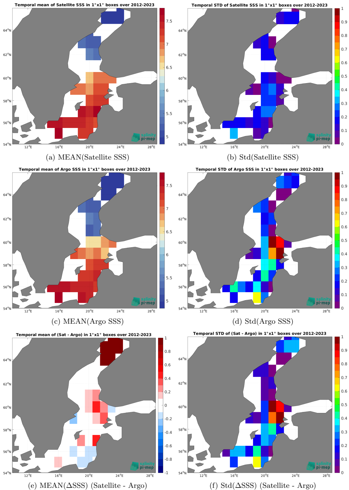
Figure 6: Temporal mean (left) and Std (right) of SSS from SMOS SSS L4 OI v342 - Weekly (CMEMS-CATDS-LOPS) (top), Argo (middle), and of \Delta SSS (Satellite - Argo). Only match-up pairs are used to generate these maps.
