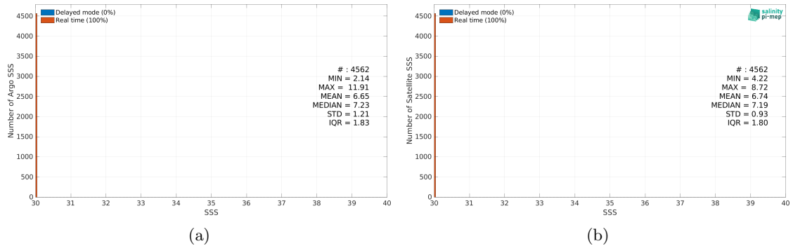
Figure 2: Histograms of SSS from Argo (a) and SMOS SSS L4 OI v342 - Weekly (CMEMS-CATDS-LOPS) (b) considering all match-up pairs per bins of 0.1 over the Baltic Sea Pi-MEP region and for the full satellite product period.
