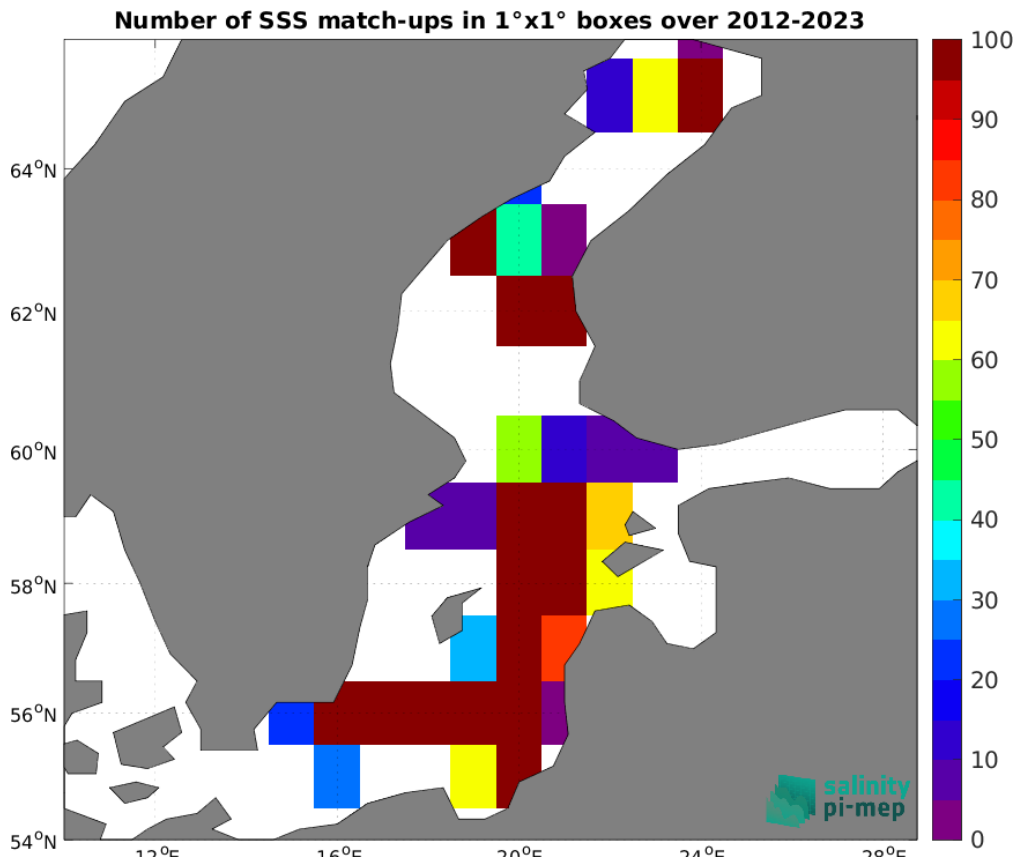
Figure 4: Number of SSS match-ups between Argo SSS and the SMOS SSS L4 OI v342 - Weekly (CMEMS-CATDS-LOPS) SSS product for the Baltic Sea Pi-MEP region over 1°x1° boxes and for the full satellite product period.
