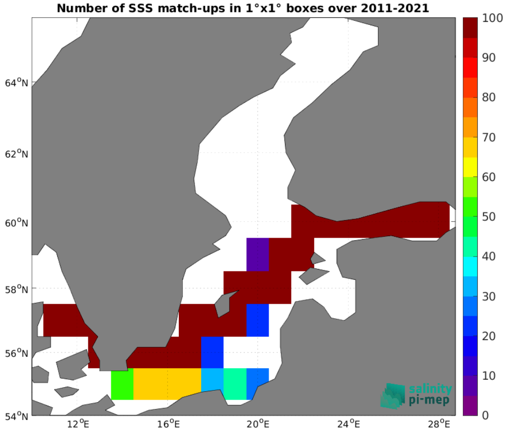
Figure 5: Number of SSS match-ups between TSG (LEGOS-DM) SSS and the SMOS SSS L4 v2 - Daily (BEC) SSS product for the Baltic Sea Pi-MEP region over 1^\circ \times 1^\circ boxes and for the full satellite product period.
