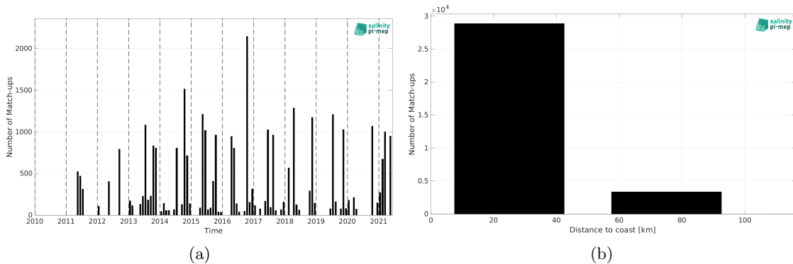
Figure 2: Number of match-ups between TSG (LEGOS-DM) and SMOS SSS L4 v2 - Daily (BEC) SSS as a function of time (a) and as function of the distance to coast (b) over the Baltic Sea Pi-MEP region and for the full satellite product period.
