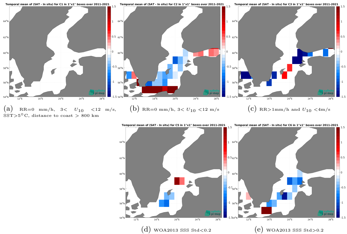
Figure 14: Temporal mean gridded over spatial boxes of size 1^\circ \times 1^\circ of \Delta\text{SSS} (SMOS SSS L4 v2 - Daily (BEC) - TSG (LEGOS-DM)) for 5 different subdatasets corresponding to:RR=0 mm/h, 3 < U_{10} < 12 m/s, SST >5^\circ\text{C} , distance to coast > 800 km (a), RR=0 mm/h, 3 < U_{10} < 12 m/s (b), RR >1 mm/h and U_{10} < 4 m/s (c), WOA2013 SSS Std <0.2 (d), WOA2013 SSS Std >0.2 (e).
