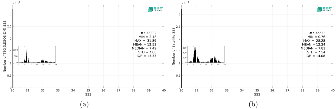
Figure 3: Histograms of SSS from TSG (LEGOS-DM) (a) and SMOS SSS L4 v2 - Daily (BEC) (b) considering all match-up pairs per bins of 0.1 over the Baltic Sea Pi-MEP region and for the full satellite product period.
