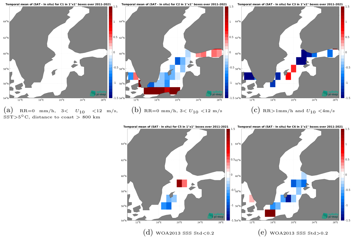
Figure 14: Temporal mean gridded over spatial boxes of size 1^\circ \times 1^\circ of \Delta SSS (SMOS SSS L4 v2 - Daily (BEC) - TSG (LEGOS-DM)) for 5 different subdatasets corresponding to:RR=0 mm/h, 3 < U_{10} < 12 m/s, SST >5^\circ\text{C} , distance to coast > 800 km (a), RR=0 mm/h, 3 < U_{10} < 12 m/s (b), RR >1 mm/h and U_{10} < 4 m/s (c), WOA2013 SSS Std <0.2 (d), WOA2013 SSS Std >0.2 (e).
