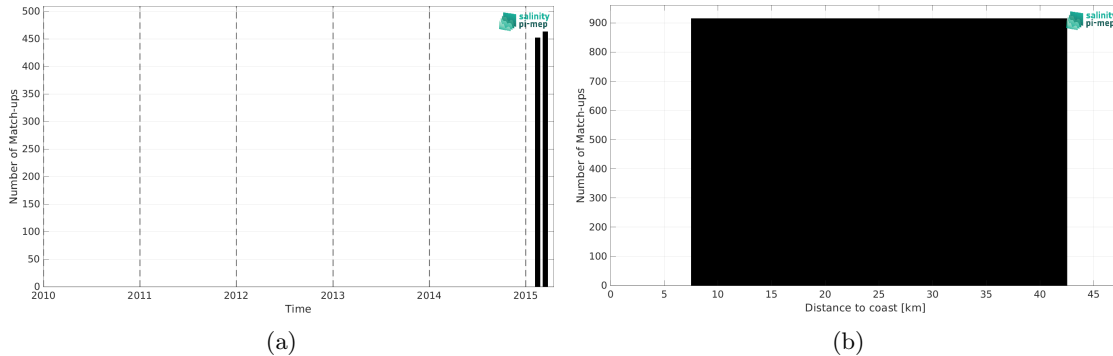
Figure 2: Number of match-ups between TSG (GOSUD-Research-vessel) and SMOS SSS L4 v2 - Daily (BEC) SSS as a function of time (a) and as function of the distance to coast (b) over the Baltic Sea Pi-MEP region and for the full satellite product period.
