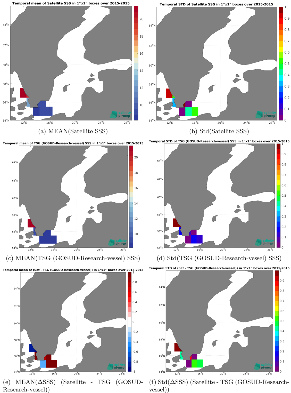
Figure 7: Temporal mean (left) and Std (right) of SSS from SMOS SSS L4 v2 - Daily (BEC) (top), TSG (GOSUD-Research-vessel) (middle), and of \Delta SSS (Satellite - TSG (GOSUD-Research-vessel)). Only match-up pairs are used to generate these maps.
