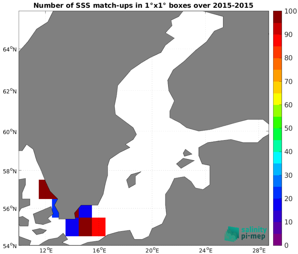
Figure 5: Number of SSS match-ups between TSG (GOSUD-Research-vessel) SSS and the SMOS SSS L4 v2 - Daily (BEC) SSS product for the Baltic Sea Pi-MEP region over 1^\circ \times 1^\circ boxes and for the full satellite product period.
