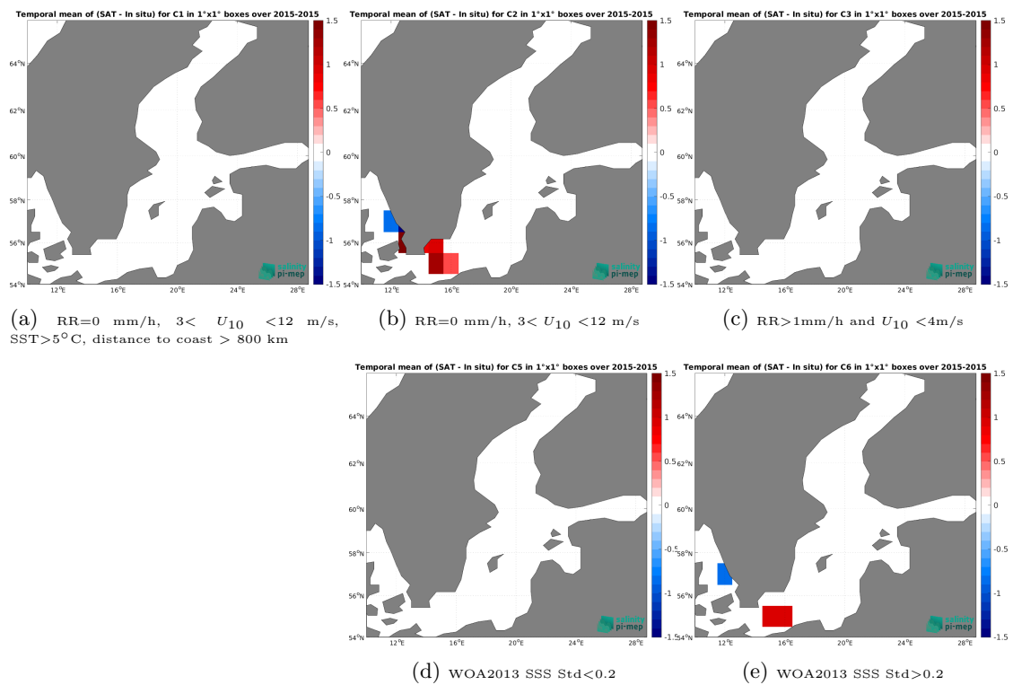
Figure 14: Temporal mean gridded over spatial boxes of size 1^\circ \times 1^\circ of \Delta SSS (SMOS SSS L4 v2 - Daily (BEC) - TSG (GOSUD-Research-vessel)) for 5 different subdatasets corresponding to:RR=0 mm/h, 3 < U_{10} < 12 m/s, SST >5^\circ\text{C} , distance to coast > 800 km (a), RR=0 mm/h, 3 < U_{10} < 12 m/s (b), RR >1 mm/h and U_{10} < 4 m/s (c), WOA2013 SSS Std <0.2 (d), WOA2013 SSS Std >0.2 (e).
