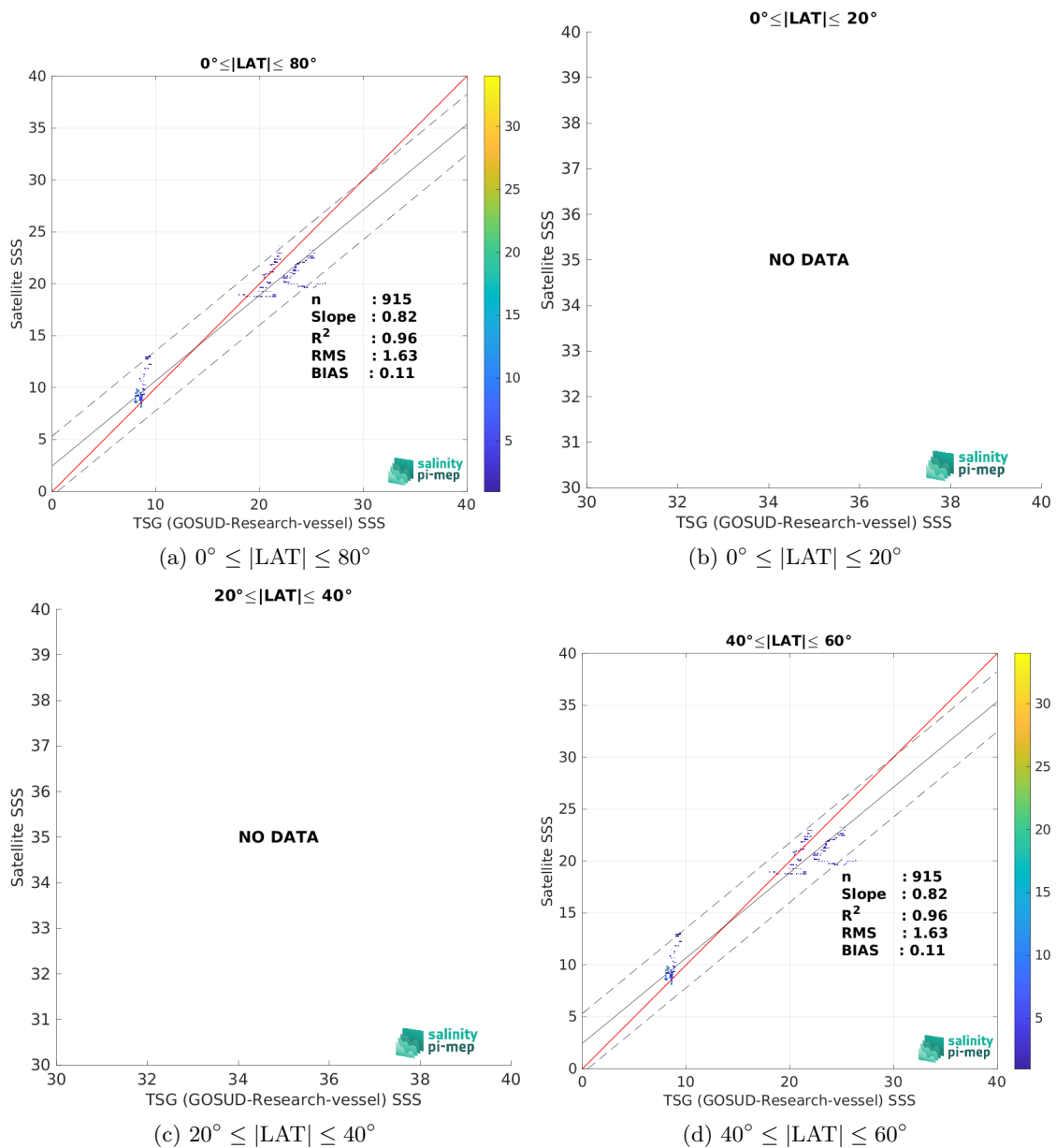
Figure 10: Contour maps of the concentration of SMOS SSS L4 v2 - Daily (BEC) SSS (y-axis) versus TSG (GOSUD-Research-vessel) SSS (x-axis) at match-up pairs for different latitude bands. For each plot, the red line shows x=y . The black thin and dashed lines indicate a linear fit through the data cloud and the \pm 95\% confidence levels, respectively. The number match-up pairs n , the slope and R^2 coefficient of the linear fit, the root mean square (RMS) and the mean bias between satellite and in situ data are indicated for each latitude band in each plots.
