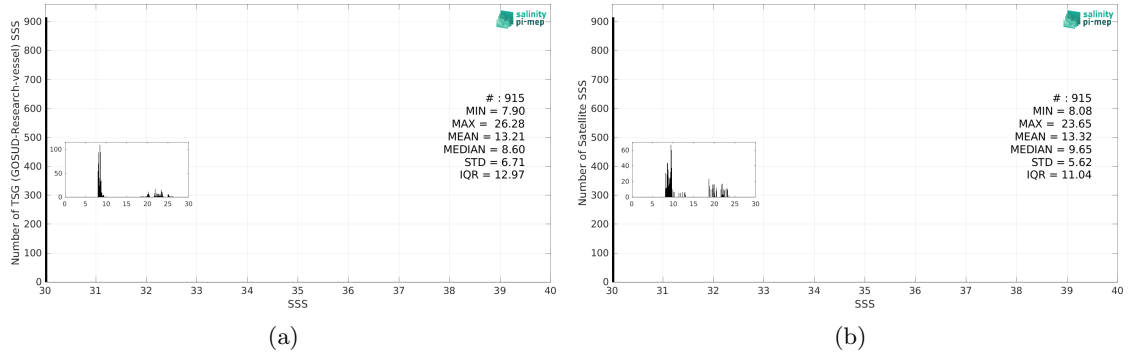
Figure 3: Histograms of SSS from TSG (GOSUD-Research-vessel) (a) and SMOS SSS L4 v2 - Daily (BEC) (b) considering all match-up pairs per bins of 0.1 over the Baltic Sea Pi-MEP region and for the full satellite product period.
