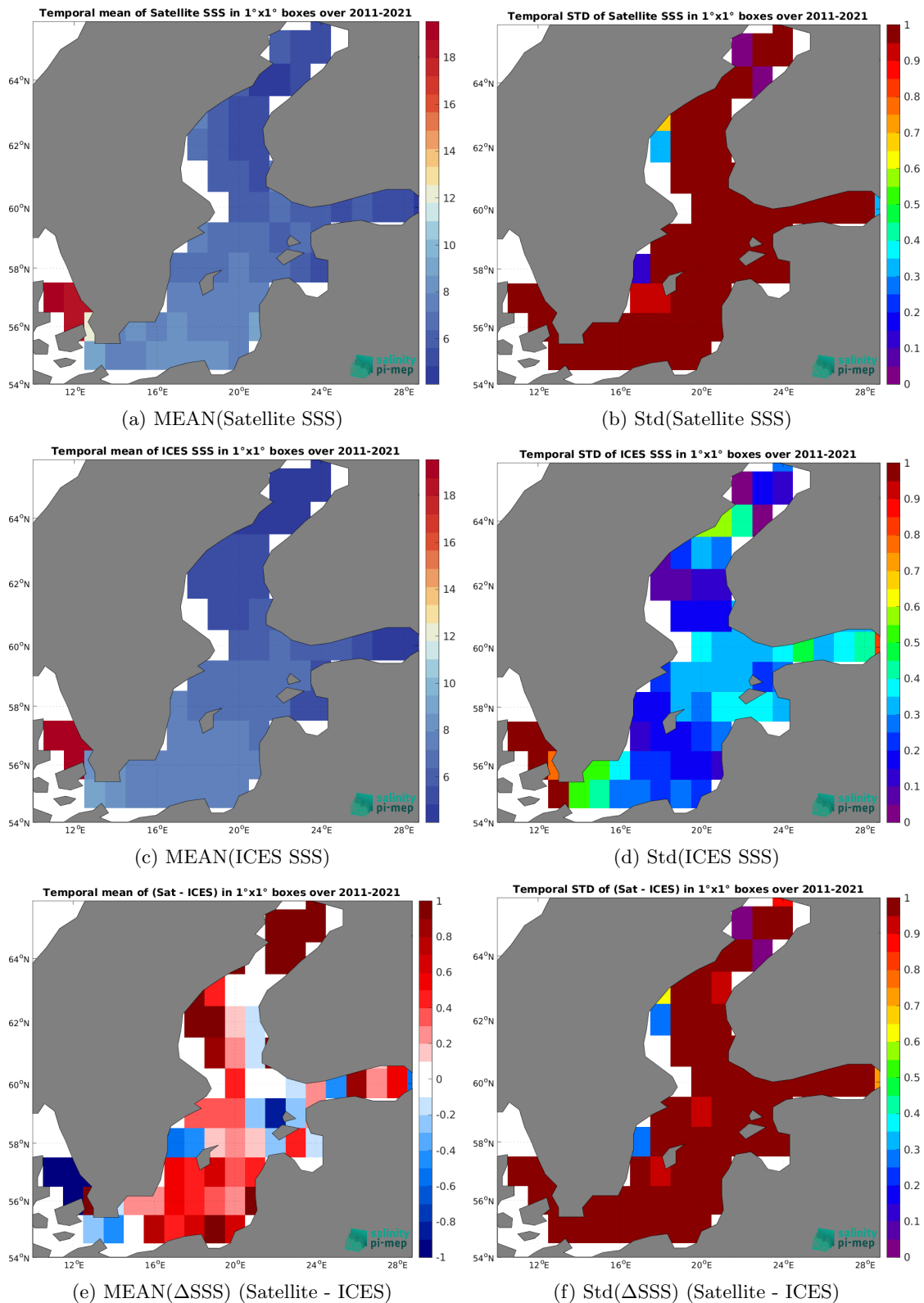
Figure 7: Temporal mean (left) and Std (right) of SSS from SMOS SSS L4 v2 - Daily (BEC) (top), ICES (middle), and of \Delta SSS (Satellite - ICES). Only match-up pairs are used to generate these maps.
