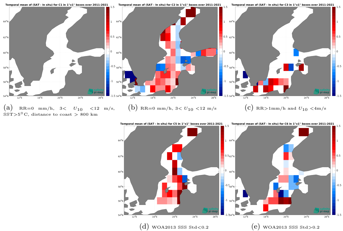
Figure 14: Temporal mean gridded over spatial boxes of size 1^\circ \times 1^\circ of \Delta SSS (SMOS SSS L4 v2 - Daily (BEC) - ICES) for 5 different subdatasets corresponding to:RR=0 mm/h, 3 < U_{10} < 12 m/s, SST >5^\circ C, distance to coast > 800 km (a), RR=0 mm/h, 3 < U_{10} < 12 m/s (b), RR >1 mm/h and U_{10} < 4 m/s (c), WOA2013 SSS Std <0.2 (d), WOA2013 SSS Std >0.2 (e).
