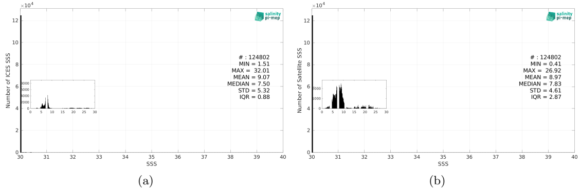
Figure 3: Histograms of SSS from ICES (a) and SMOS SSS L4 v2 - Daily (BEC) (b) considering all match-up pairs per bins of 0.1 over the Baltic Sea Pi-MEP region and for the full satellite product period.
