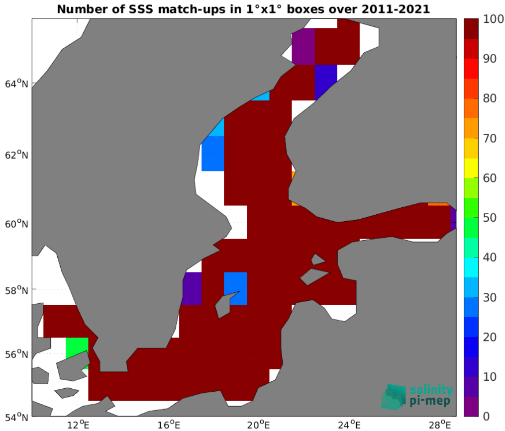
Figure 5: Number of SSS match-ups between ICES SSS and the SMOS SSS L4 v2 - Daily (BEC) SSS product for the Baltic Sea Pi-MEP region over 1^\circ \times 1^\circ boxes and for the full satellite product period.
