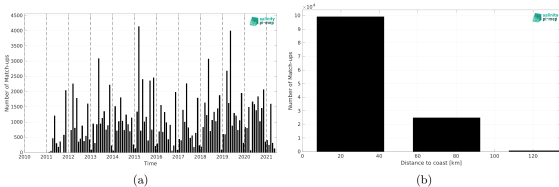
Figure 2: Number of match-ups between ICES and SMOS SSS L4 v2 - Daily (BEC) SSS as a function of time (a) and as function of the distance to coast (b) over the Baltic Sea Pi-MEP region and for the full satellite product period.
