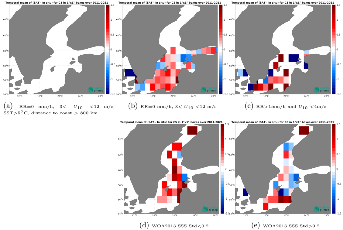
Figure 12: Temporal mean gridded over spatial boxes of size 1^{\circ}\times 1^{\circ} of \Delta\text{SSS} (SMOS SSS L4 v2 - Daily (BEC) - ICES) for 5 different subdatasets corresponding to: \text{RR}=0 mm/h, 3 < U_{10} < 12 m/s, \text{SST} > 5^{\circ}\text{C} , distance to coast > 800 km (a), \text{RR}=0 mm/h, 3 < U_{10} < 12 m/s (b), \text{RR} > 1\text{mm/h} and U_{10} < 4\text{m/s} (c), WOA2013 SSS Std < 0.2 (d), WOA2013 SSS Std > 0.2 (e).
