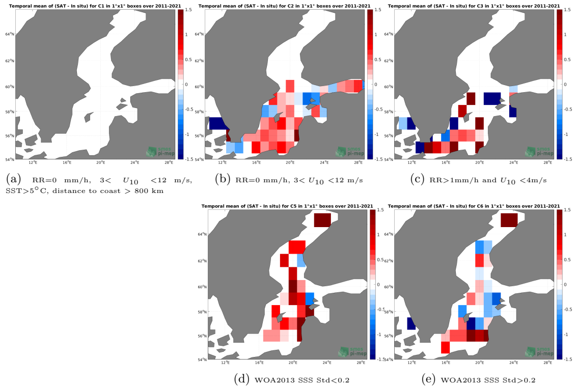
Figure 12: Temporal mean gridded over spatial boxes of size 1^{\circ}\times 1^{\circ} of \Delta\text{SSS} (SMOS SSS L4 v2 - Daily (BEC) - ICES) for 5 different subdatasets corresponding to:RR=0 mm/h, 3 < U_{10} < 12 m/s, SST >5^{\circ}\text{C} , distance to coast > 800 km (a), RR=0 mm/h, 3 < U_{10} < 12 m/s (b), RR >1 mm/h and U_{10} < 4 m/s (c), WOA2013 SSS Std <0.2 (d), WOA2013 SSS Std >0.2 (e).
