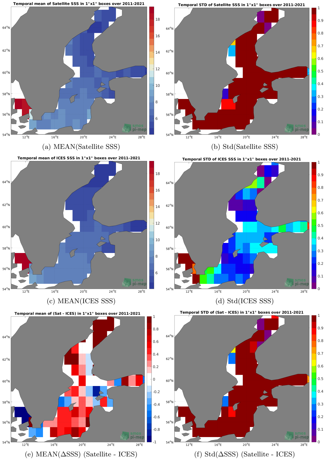
Figure 6: Temporal mean (left) and Std (right) of SSS from SMOS SSS L4 v2 - Daily (BEC) (top), ICES (middle), and of \Delta SSS (Satellite - ICES). Only match-up pairs are used to generate these maps.
