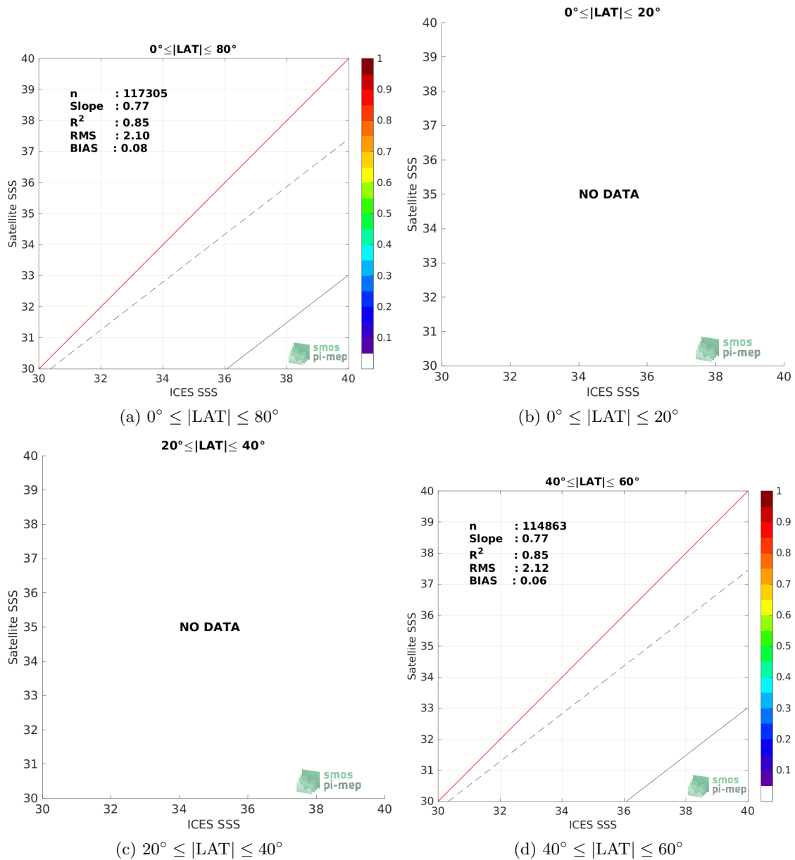
Figure 9: Contour maps of the concentration of SMOS SSS L4 v2 - Daily (BEC) SSS (y-axis) versus ICES SSS (x-axis) at match-up pairs for different latitude bands. For each plot, the red line shows x=y . The black thin and dashed lines indicate a linear fit through the data cloud and the \pm 95\% confidence levels, respectively. The number match-up pairs n , the slope and R^2 coefficient of the linear fit, the root mean square (RMS) and the mean bias between satellite and in situ data are indicated for each latitude band in each plots.
