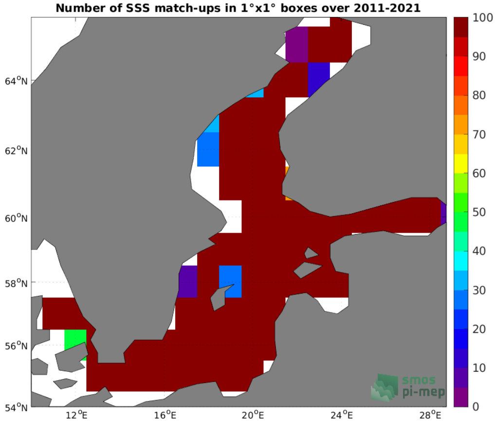
Figure 4: Number of SSS match-ups between ICES SSS and the SMOS SSS L4 v2 - Daily (BEC) SSS product for the Baltic Sea Pi-MEP region over 1^\circ \times 1^\circ boxes and for the full satellite product period.
