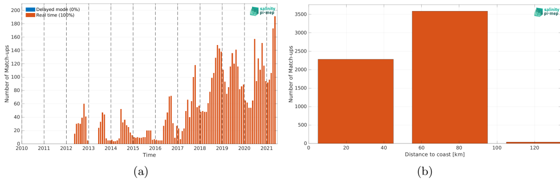
Figure 2: Number of match-ups between Argo and SMOS SSS L4 v2 - Daily (BEC) SSS as a function of time (a) and as function of the distance to coast (b) over the Baltic Sea Pi-MEP region and for the full satellite product period.
