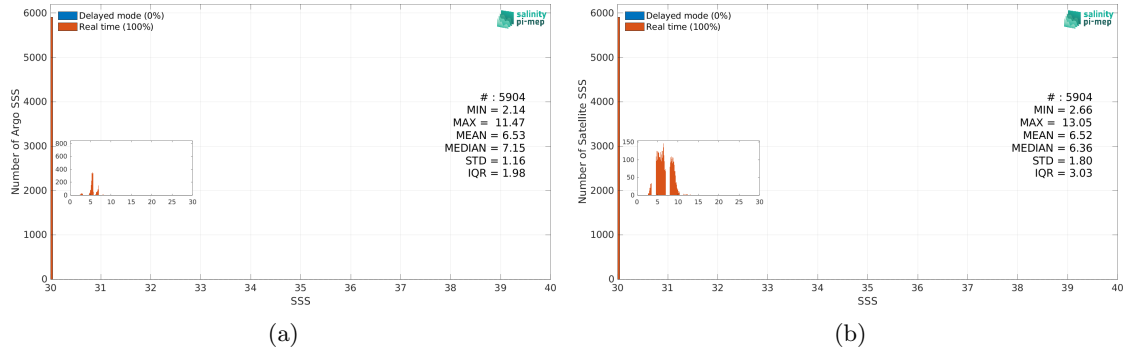
Figure 3: Histograms of SSS from Argo (a) and SMOS SSS L4 v2 - Daily (BEC) (b) considering all match-up pairs per bins of 0.1 over the Baltic Sea Pi-MEP region and for the full satellite product period.
