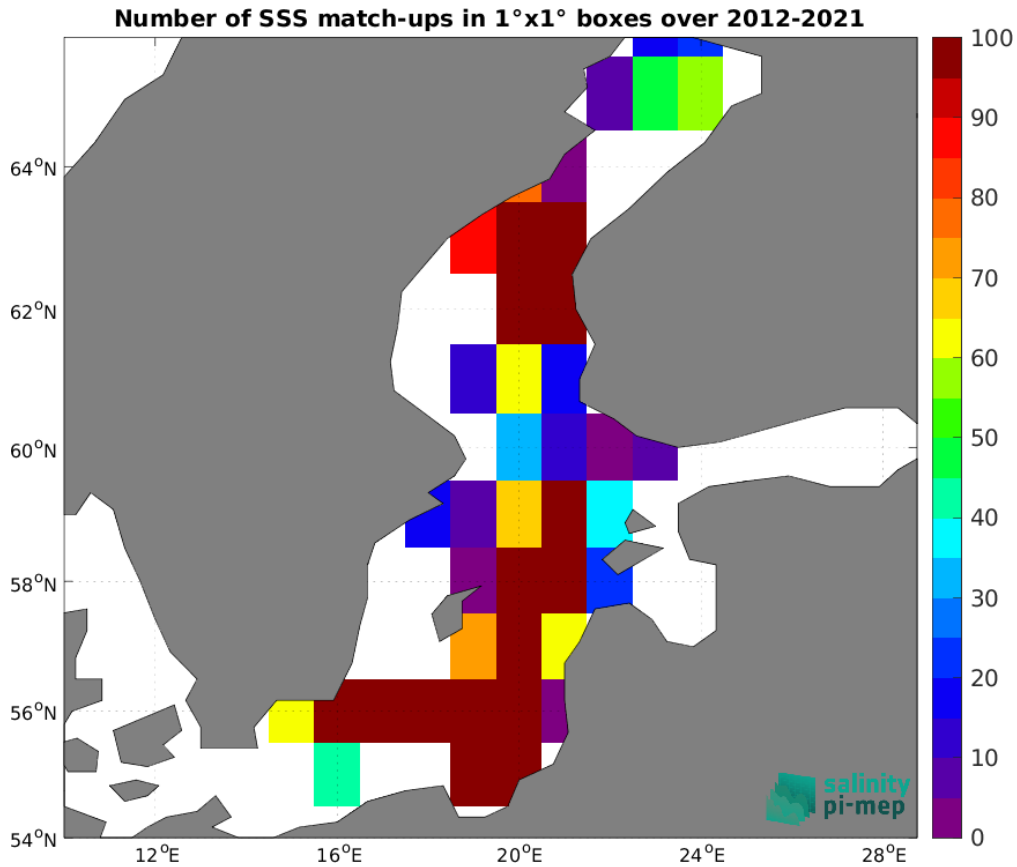
Figure 5: Number of SSS match-ups between Argo SSS and the SMOS SSS L4 v2 - Daily (BEC) SSS product for the Baltic Sea Pi-MEP region over 1^\circ \times 1^\circ boxes and for the full satellite product period.
