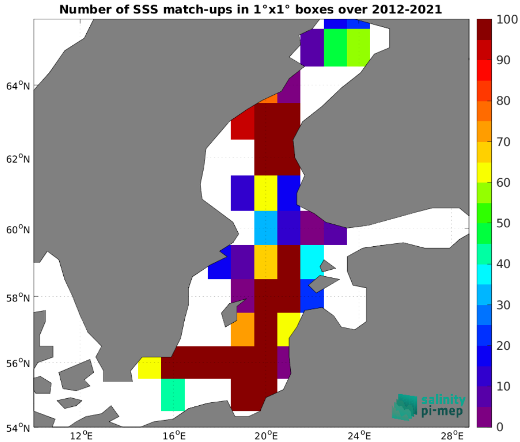
Figure 4: Number of SSS match-ups between Argo SSS and the SMOS SSS L4 v2 - Daily (BEC) SSS product for the Baltic Sea Pi-MEP region over 1^\circ \times 1^\circ boxes and for the full satellite product period.
