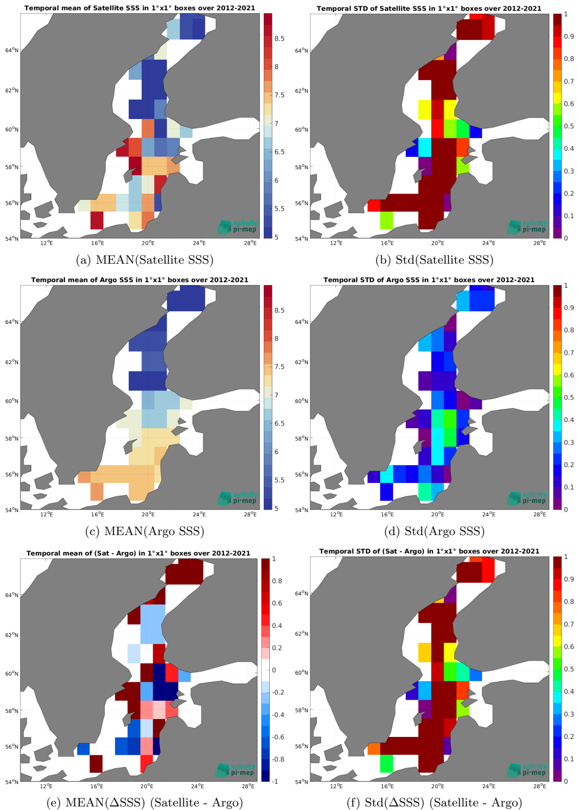
Figure 6: Temporal mean (left) and Std (right) of SSS from SMOS SSS L4 v2 - Daily (BEC) (top), Argo (middle), and of \Delta\text{SSS} (Satellite - Argo). Only match-up pairs are used to generate these maps.
