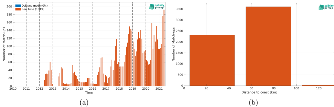
Figure 1: Number of match-ups between Argo and SMOS SSS L4 v2 - Daily (BEC) SSS as a function of time (a) and as function of the distance to coast (b) over the Baltic Sea Pi-MEP region and for the full satellite product period.
