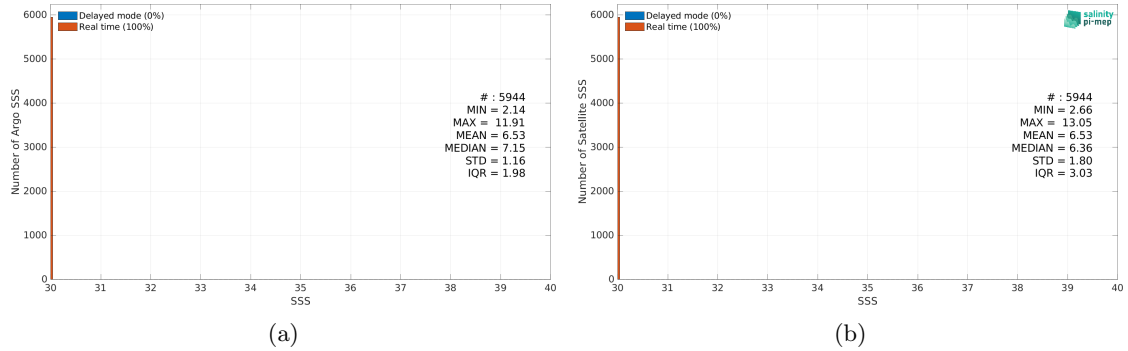
Figure 2: Histograms of SSS from Argo (a) and SMOS SSS L4 v2 - Daily (BEC) (b) considering all match-up pairs per bins of 0.1 over the Baltic Sea Pi-MEP region and for the full satellite product period.
