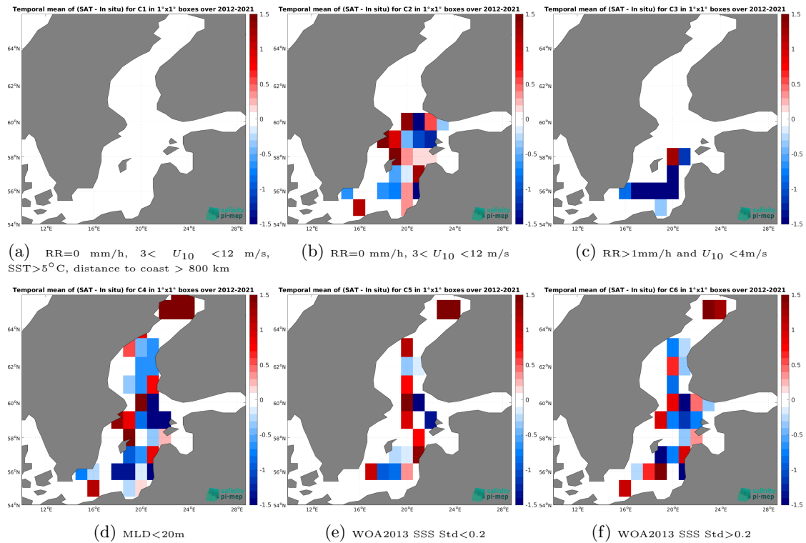
Figure 12: Temporal mean gridded over spatial boxes of size 1^{\circ}\times 1^{\circ} of \Delta\text{SSS} (SMOS SSS L4 v2 - Daily (BEC) - Argo) for 6 different subdatasets corresponding to:RR=0 mm/h, 3 < U_{10} < 12 m/s, SST >5^{\circ}\text{C} , distance to coast > 800 km (a), RR=0 mm/h, 3 < U_{10} < 12 m/s (b), RR >1\text{mm/h} and U_{10} < 4\text{m/s} (c),MLD <20\text{m} (d),WOA2013 SSS Std <0.2 (e),WOA2013 SSS Std >0.2 (f).
