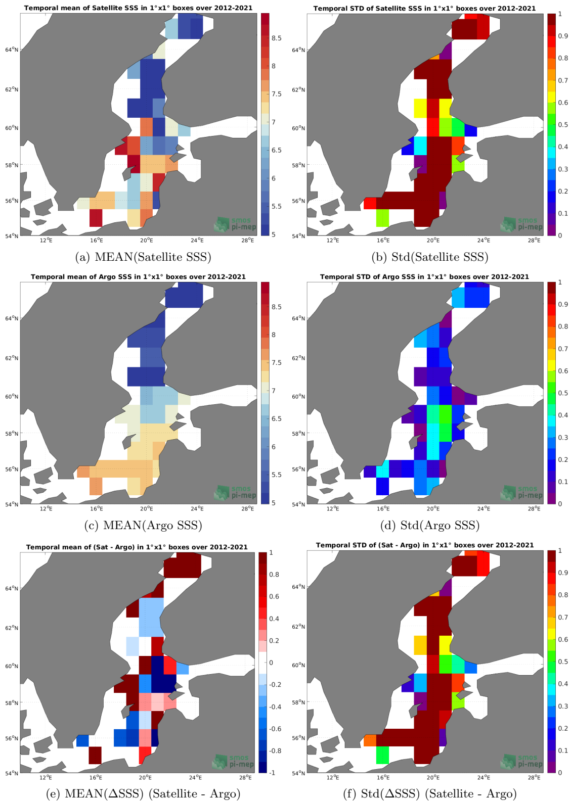
Figure 6: Temporal mean (left) and Std (right) of SSS from SMOS SSS L4 v2 - Daily (BEC) (top), Argo (middle), and of \Delta SSS (Satellite - Argo). Only match-up pairs are used to generate these maps.
