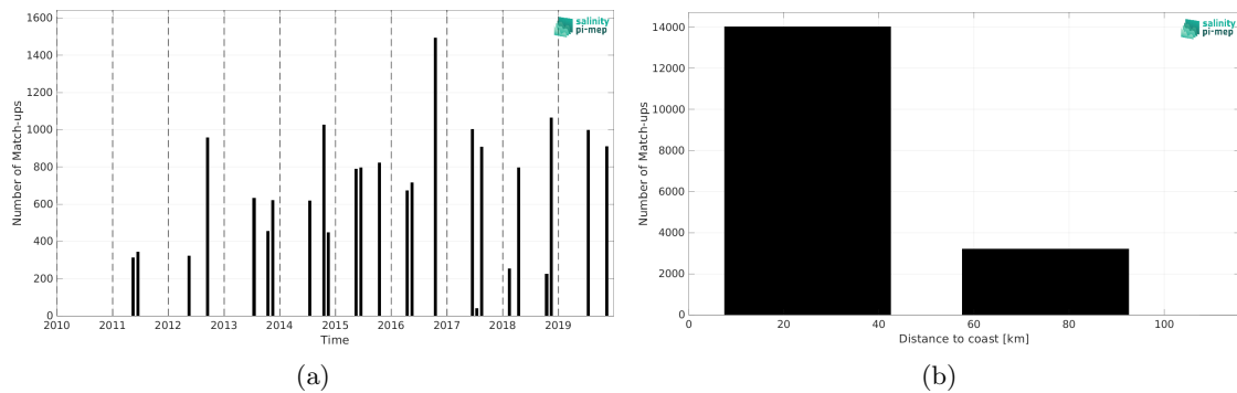
Figure 2: Number of match-ups between TSG (LEGOS-DM) and SMOS SSS L4 Baltic v1 - Daily (BEC) SSS as a function of time (a) and as function of the distance to coast (b) over the Baltic Sea Pi-MEP region and for the full satellite product period.
