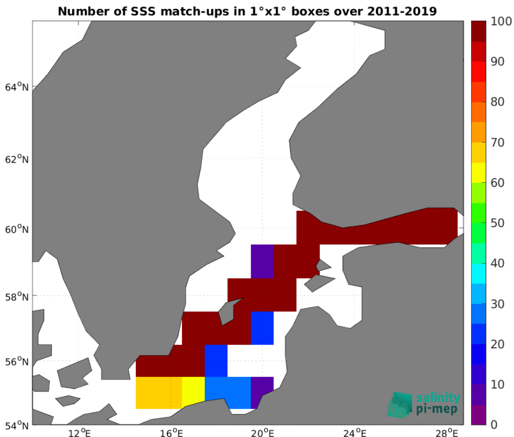
Figure 5: Number of SSS match-ups between TSG (LEGOS-DM) SSS and the SMOS SSS L4 Baltic v1 - Daily (BEC) SSS product for the Baltic Sea Pi-MEP region over 1^\circ \times 1^\circ boxes and for the full satellite product period.
