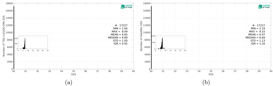
Figure 3: Histograms of SSS from TSG (LEGOS-DM) (a) and SMOS SSS L4 Baltic v1 - Daily (BEC) (b) considering all match-up pairs per bins of 0.1 over the Baltic Sea Pi-MEP region and for the full satellite product period.
