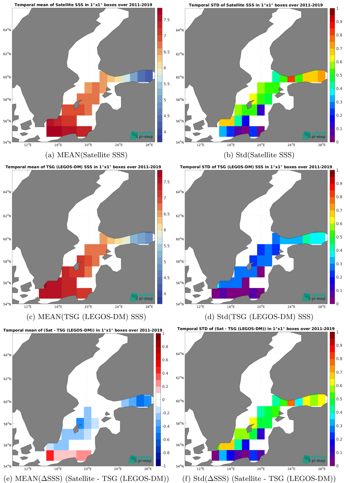
Figure 7: Temporal mean (left) and Std (right) of SSS from SMOS SSS L4 Baltic v1 - Daily (BEC) (top), TSG (LEGOS-DM) (middle), and of \Delta SSS (Satellite - TSG (LEGOS-DM)). Only match-up pairs are used to generate these maps.
