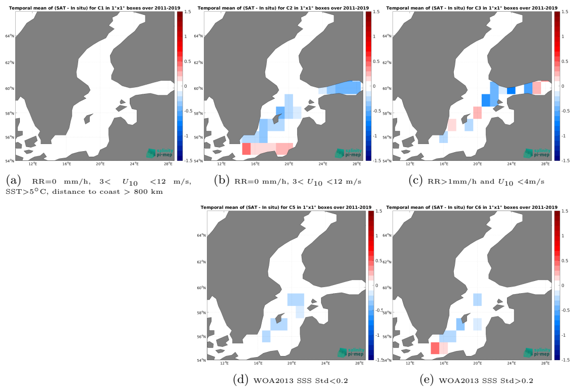
Figure 14: Temporal mean gridded over spatial boxes of size 1^\circ \times 1^\circ of \Delta SSS (SMOS SSS L4 Baltic v1 - Daily (BEC) - TSG (LEGOS-DM)) for 5 different subdatasets corresponding to:RR=0 mm/h, 3 < U_{10} < 12 m/s, SST >5^\circ C, distance to coast > 800 km (a), RR=0 mm/h, 3 < U_{10} < 12 m/s (b), RR >1 mm/h and U_{10} < 4 m/s (c), WOA2013 SSS Std <0.2 (d), WOA2013 SSS Std >0.2 (e).
