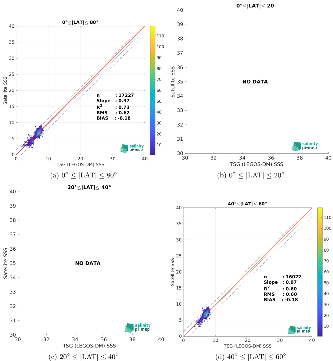
Figure 10: Contour maps of the concentration of SMOS SSS L4 Baltic v1 - Daily (BEC) SSS (y-axis) versus TSG (LEGOS-DM) SSS (x-axis) at match-up pairs for different latitude bands. For each plot, the red line shows x=y . The black thin and dashed lines indicate a linear fit through the data cloud and the \pm 95\% confidence levels, respectively. The number match-up pairs n , the slope and R^2 coefficient of the linear fit, the root mean square (RMS) and the mean bias between satellite and in situ data are indicated for each latitude band in each plots.
