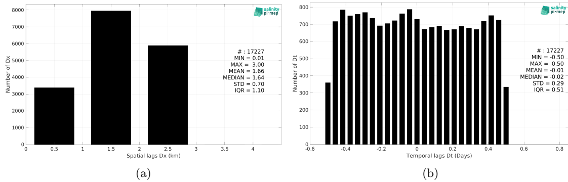
Figure 6: Histograms of the spatial (a) and temporal (b) lags between the location/time of the TSG (LEGOS-DM) measurement and the date of the corresponding SMOS SSS L4 Baltic v1 - Daily (BEC) SSS pixel.
