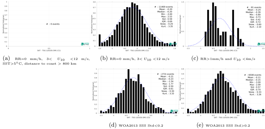
Figure 15: Normalized histogram of \Delta SSS (SMOS SSS L4 Baltic v1 - Daily (BEC) - TSG (LEGOS-DM)) for 5 different subdatasets corresponding to: RR=0 mm/h, 3 < U_{10} < 12 m/s, SST>5°C, distance to coast > 800 km (a), RR=0 mm/h, 3 < U_{10} < 12 m/s (b), RR>1mm/h and U_{10} < 4 m/s (c), WOA2013 SSS Std<0.2 (d), WOA2013 SSS Std>0.2 (e).
