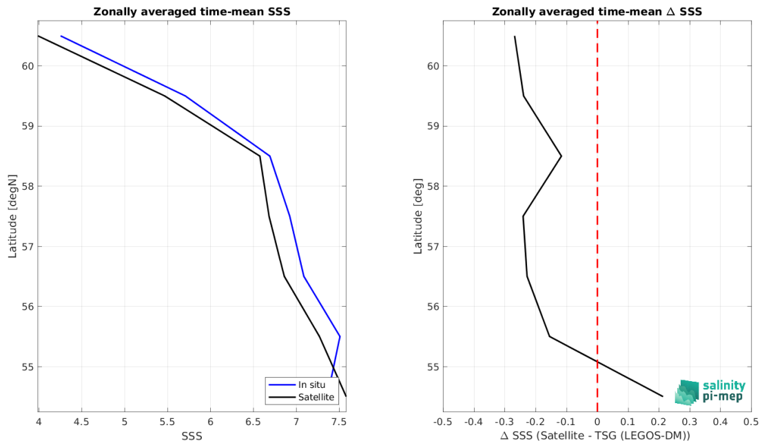
Figure 9: Left panel: Zonal mean SSS from SMOS SSS L4 Baltic v1 - Daily (BEC) satellite product (black) and from TSG (LEGOS-DM) (blue). Right panel: Zonal mean of \Delta SSS (Satellite - TSG (LEGOS-DM)) for all the collected Pi-MEP match-up pairs estimated over the full satellite product period.
